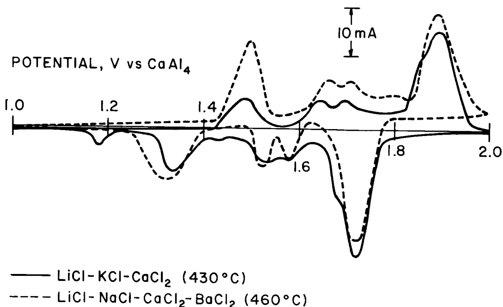
Fig. IX-3. Cyclic Voltammograms for \text{NiS}_2 Electrodes
