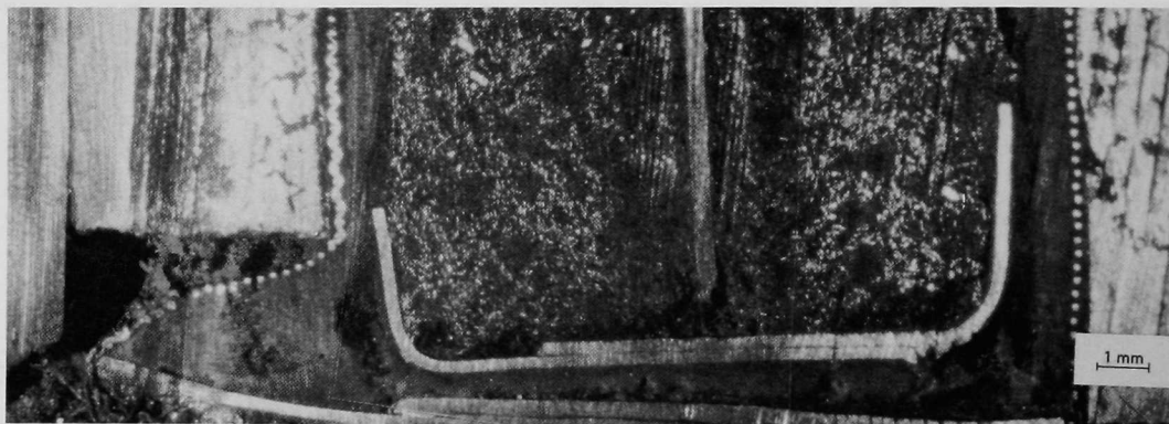
e. Mechanical damage of screen basket caused by negative electrode.
