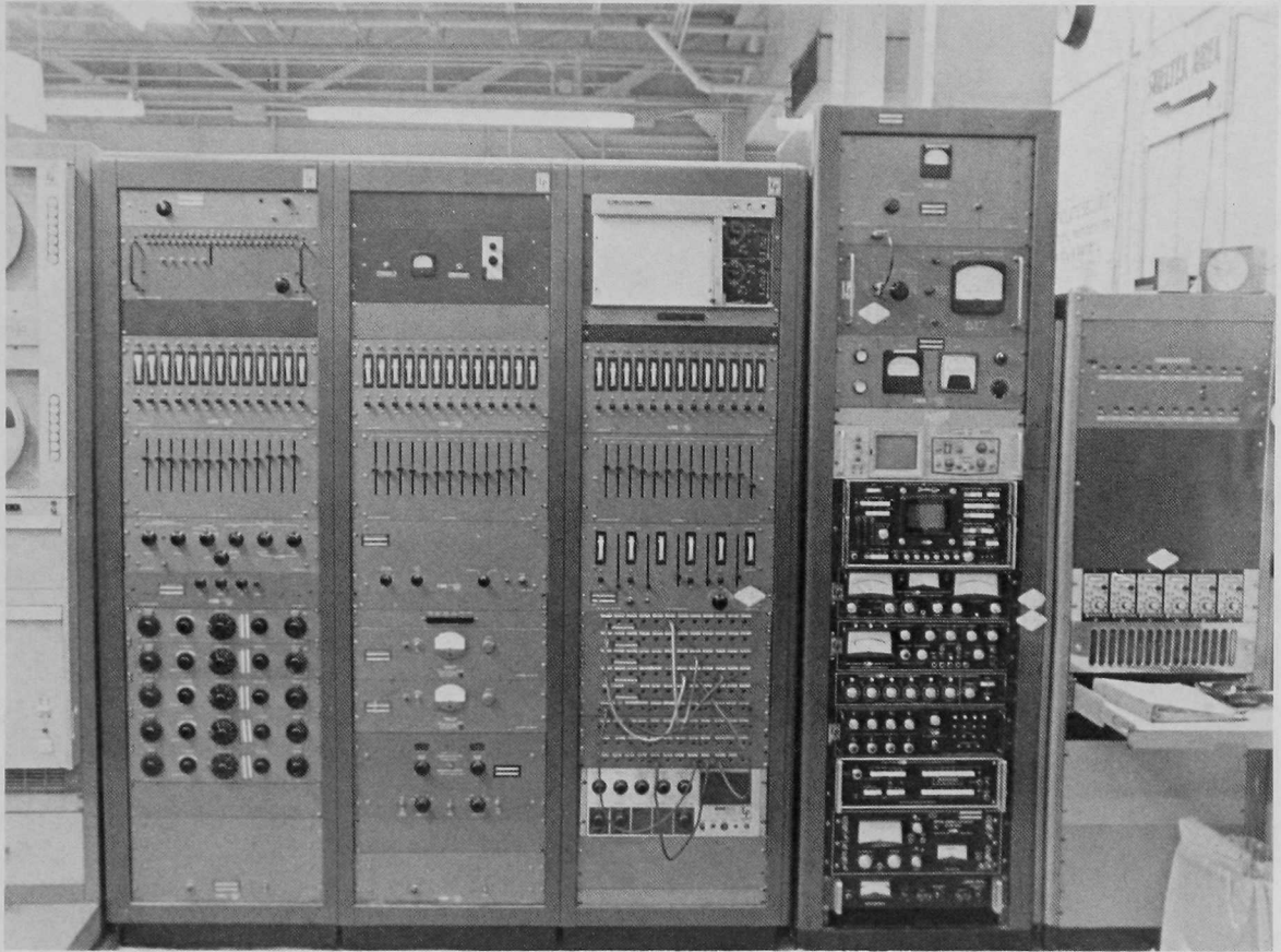
Fig. III-10. Vibration Test Control Equipment
