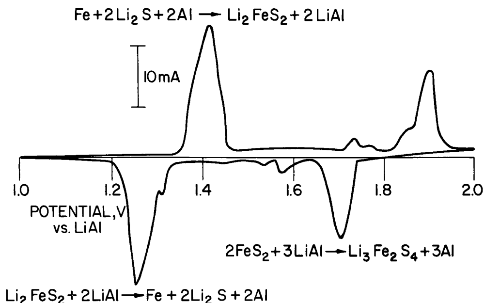
Figure VIII-2. Cyclic Voltammogram of \text{FeS}_2 Electrode in \text{LiCl-KCl} Electrolyte of Eutectic Composition
