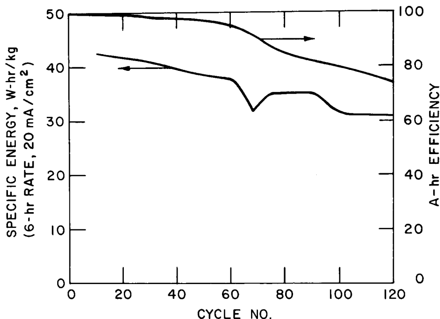
Fig. IX-1. Performance of \text{Ca}(\text{Mg}_2\text{Si})/\text{NiS}_2 Cell
