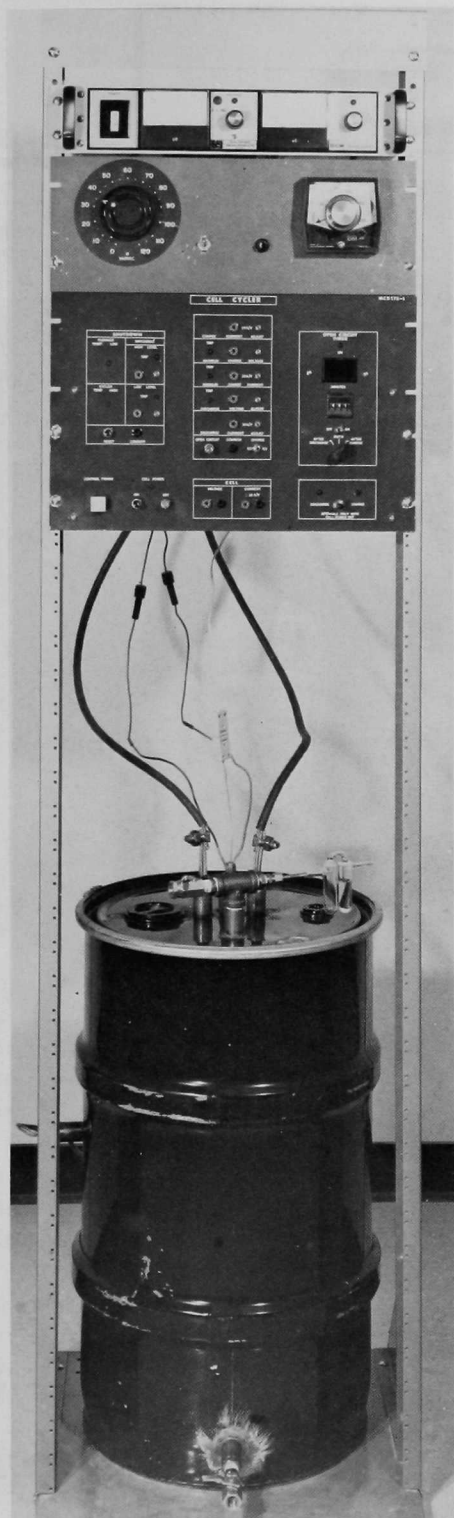
Fig. IV-5. Individual Cell Testing Module (ANL Neg. No. 308-78-178)
