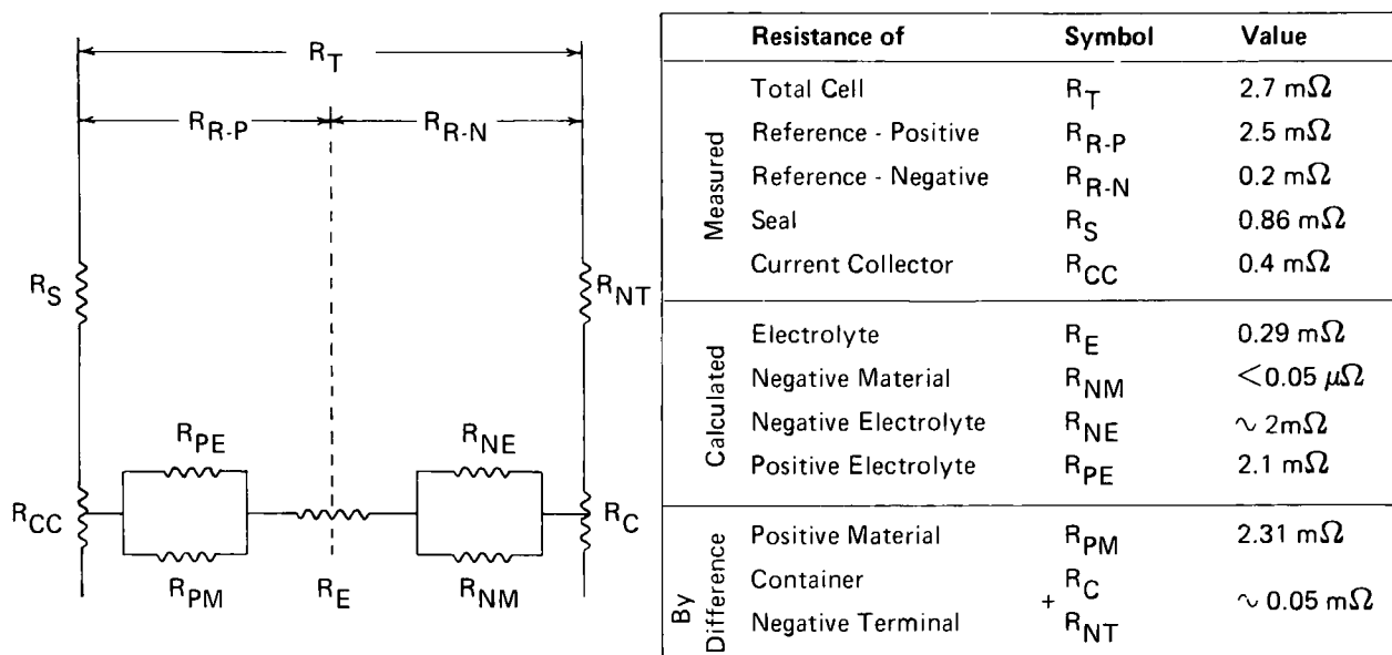
Fig. III-16. Gould LiAl/FeS Bicell Resistance Diagram
