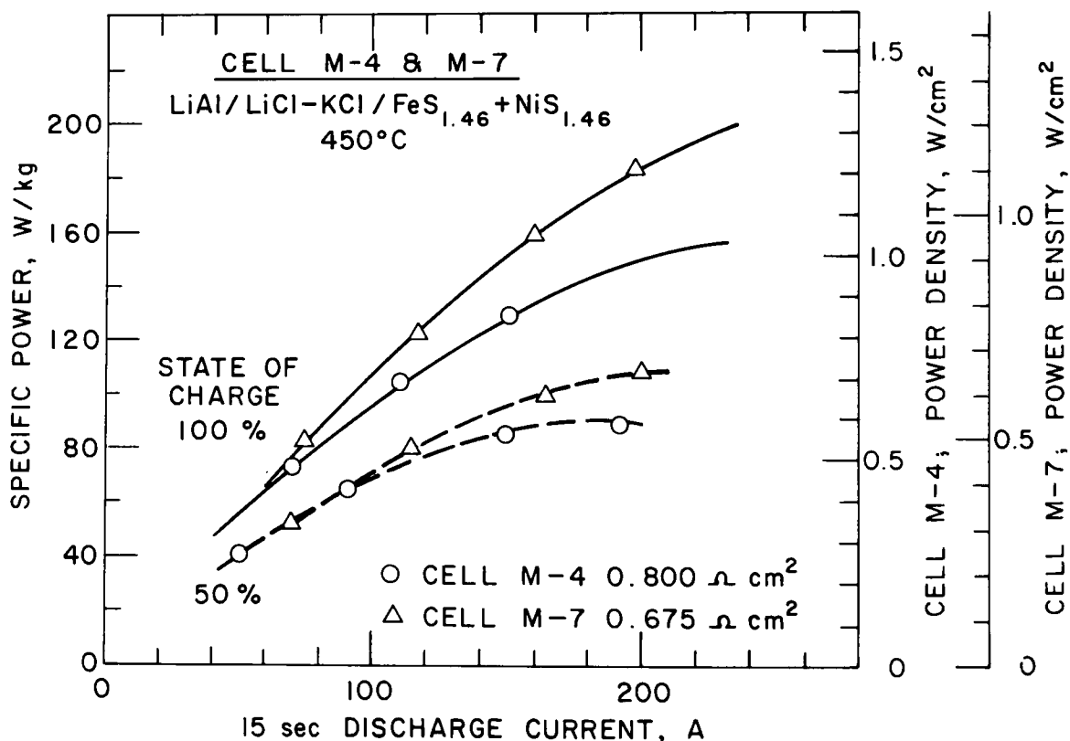
Fig. VI-6. Power Characteristics of Cells M-4 and M-7.
