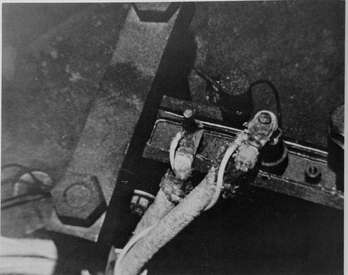
Fig. III-11. Vibration Cell Electrical Connections
