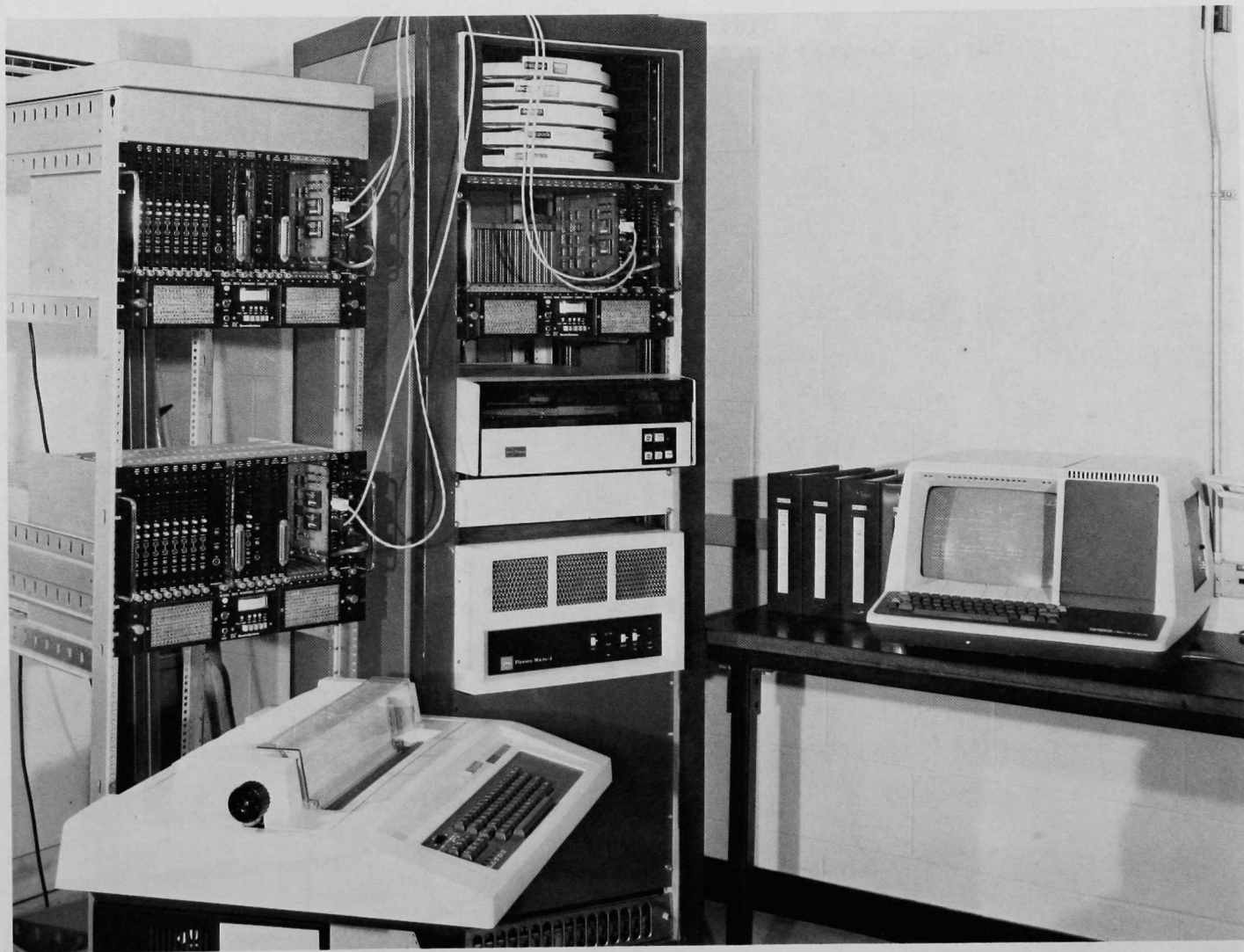
Fig. IV-3. Computer System for Battery Cycling (ANL Neg. No. 308-78-464)
