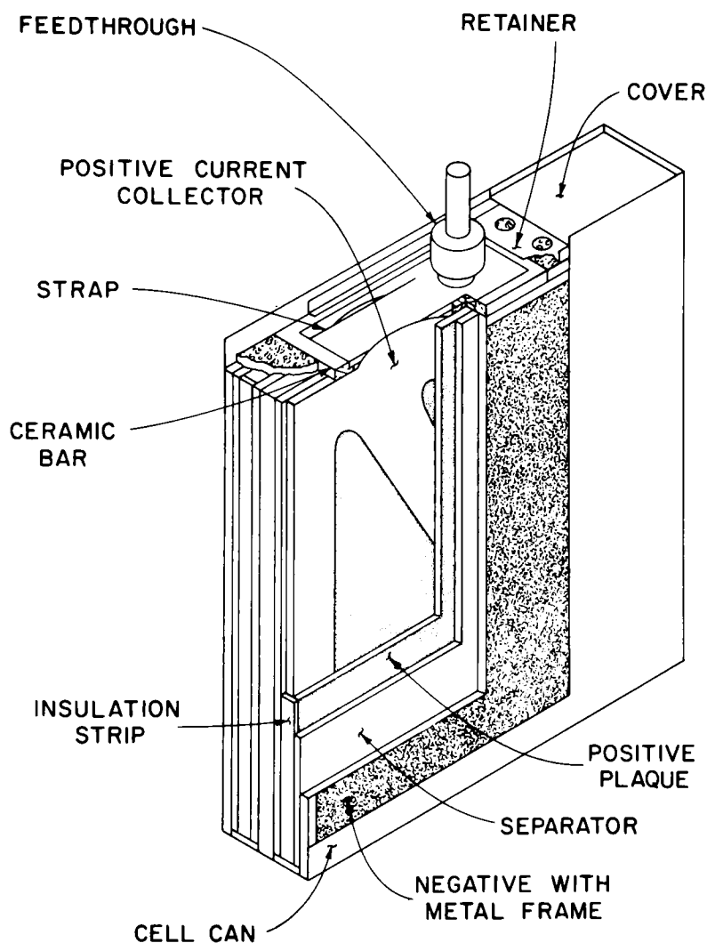
Fig. VI-5. Multiplate Cell Design.
