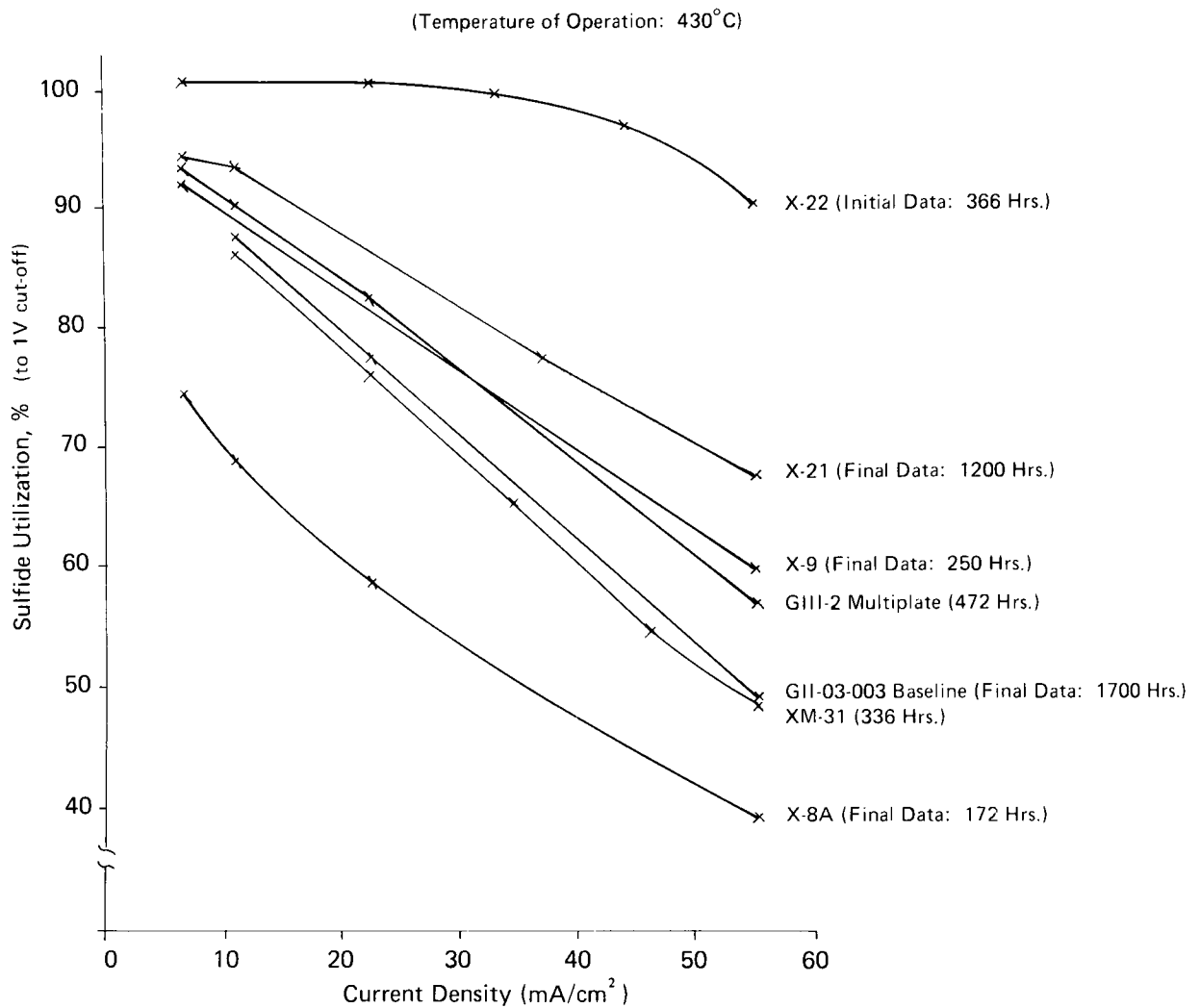
Fig. III-15. Positive Utilization as a Function of Current Density for Seven Gould Cells
