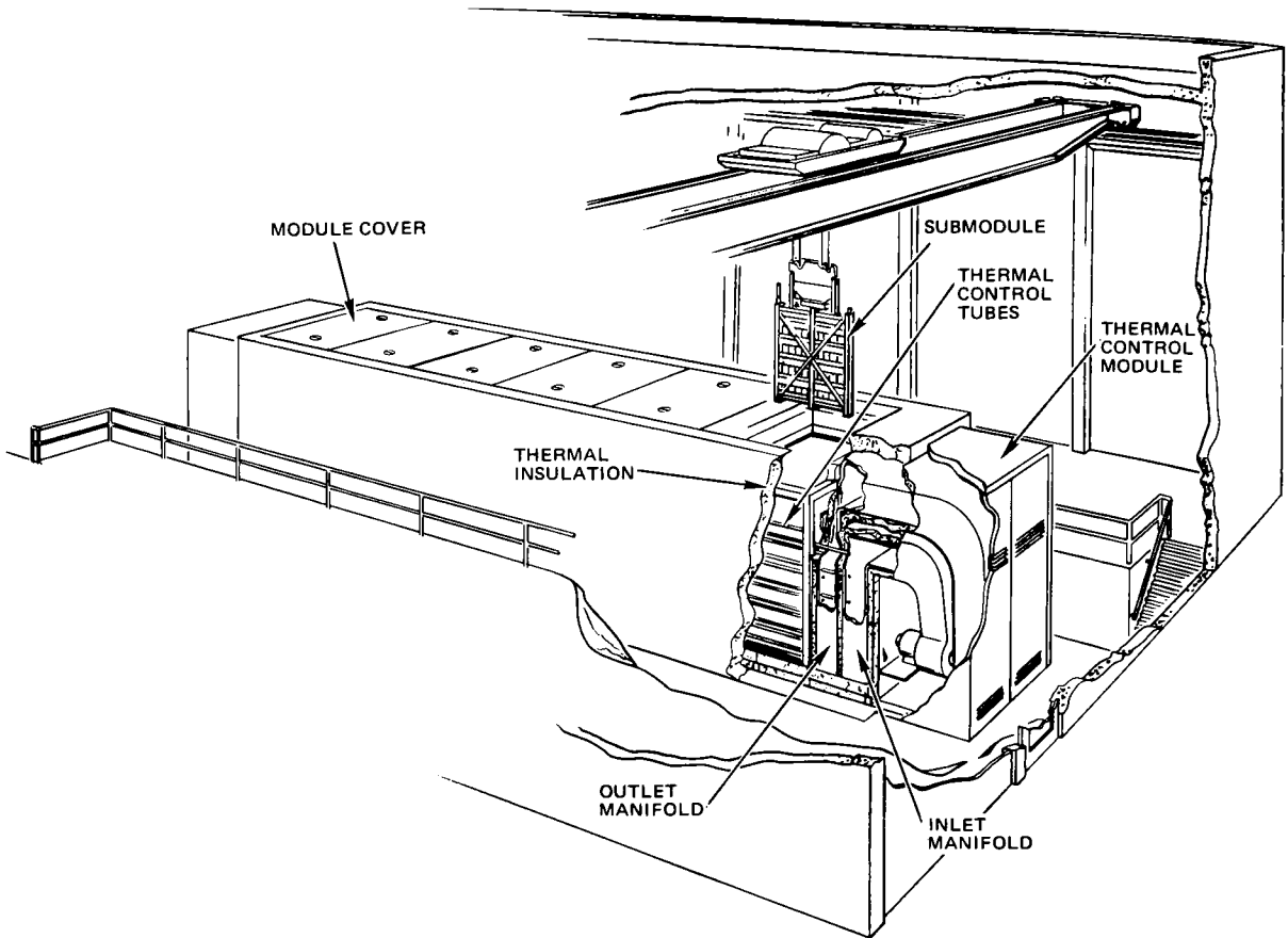
Fig. III-33. A 4-MW-hr Battery Module in the BEST Facility
