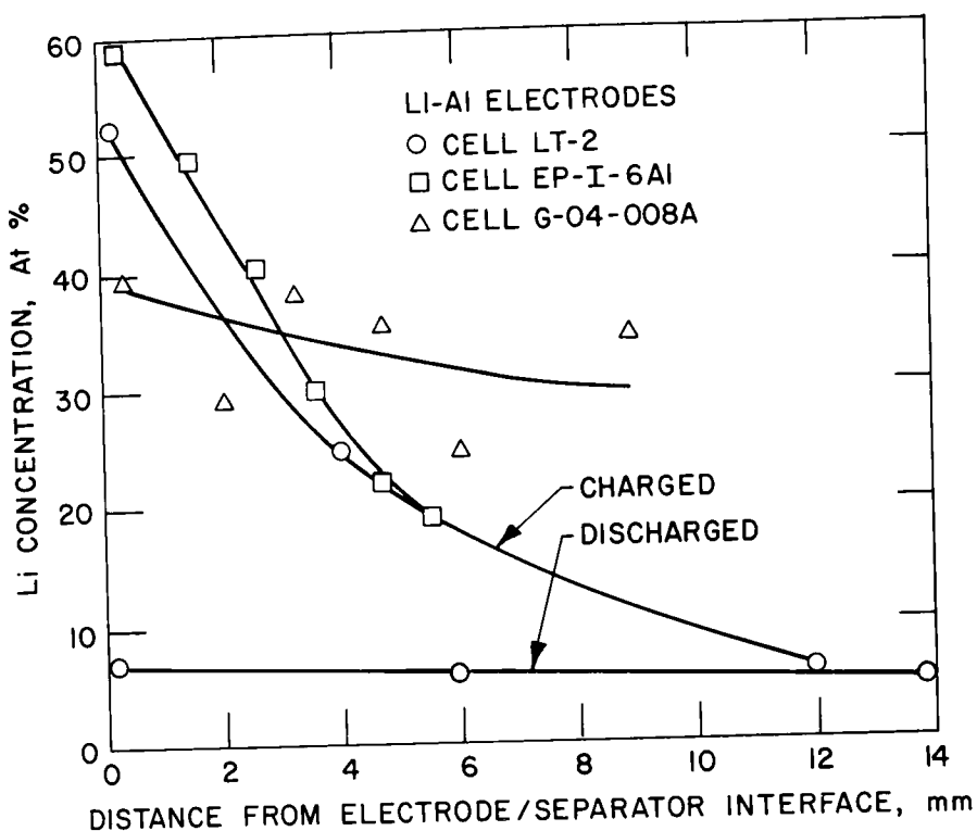
Fig. VII-7. Lithium Concentration Profiles in the Negative Electrodes of Three Cells
