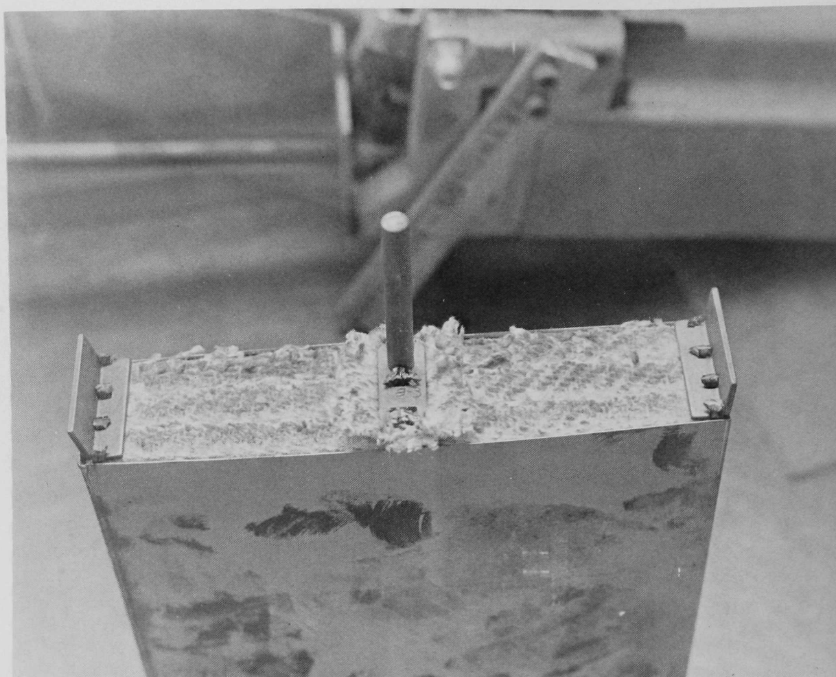
Fig. III-4. Positive and Negative Bus Welded in Place
