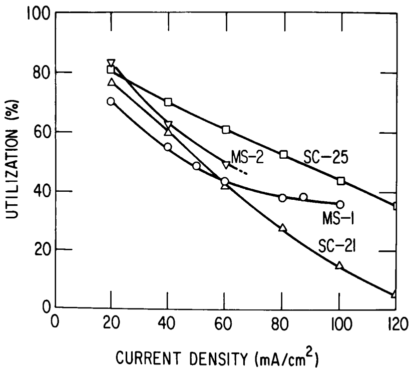
Fig. VII-4. Performance of Cells with Rigid Y_2O_3 (MS-1 and -2), BN Felt (SC-25), and MgO Powder (SC-21) Separators.
