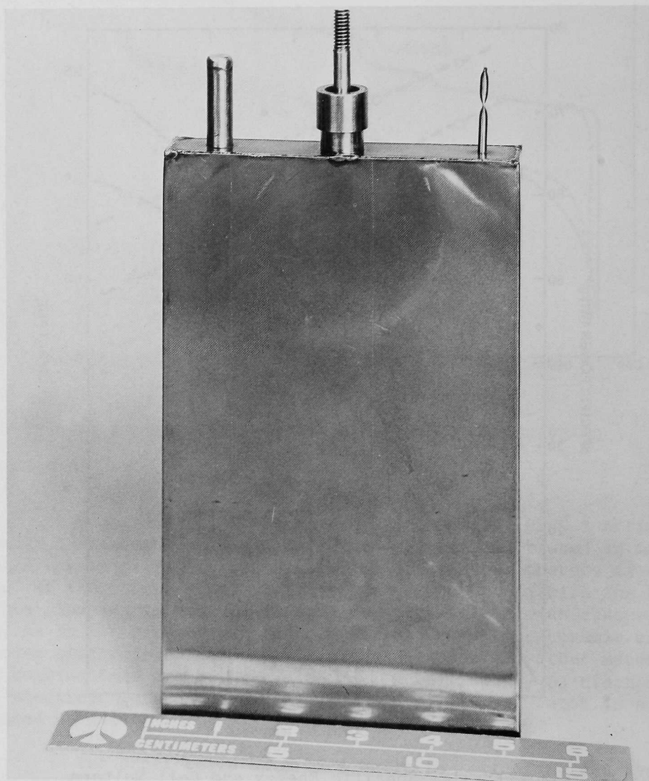
Fig. III-32. Electric-Vehicle Cell
