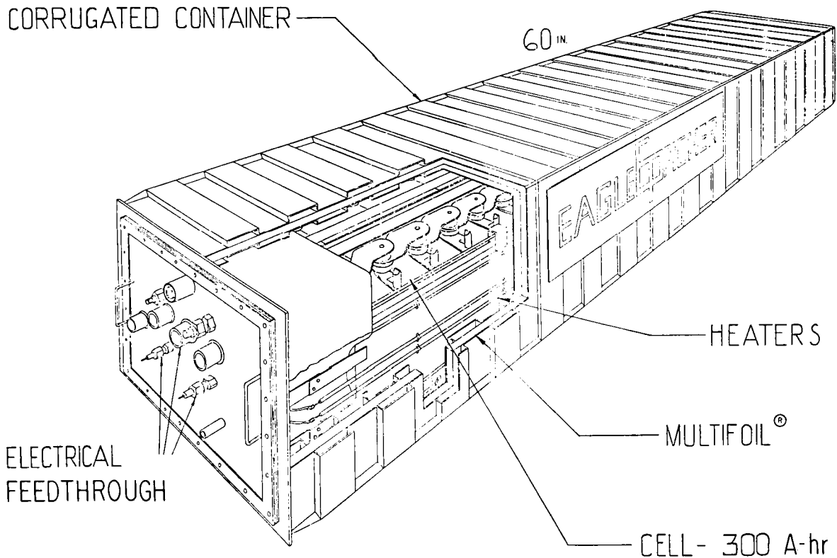
Fig. III-5. Battery Case for a 20-kW-hr Battery Module
