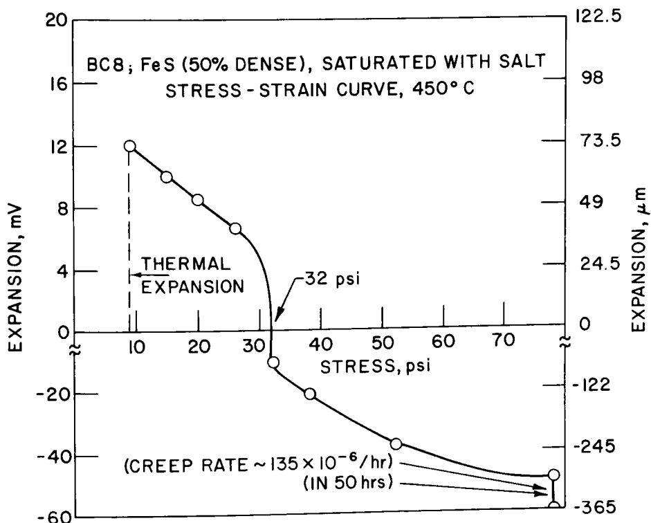
Fig. VII-5. Creep Behavior of FeS + LiCl-KCl Sample (Constrained) at 450°C.
