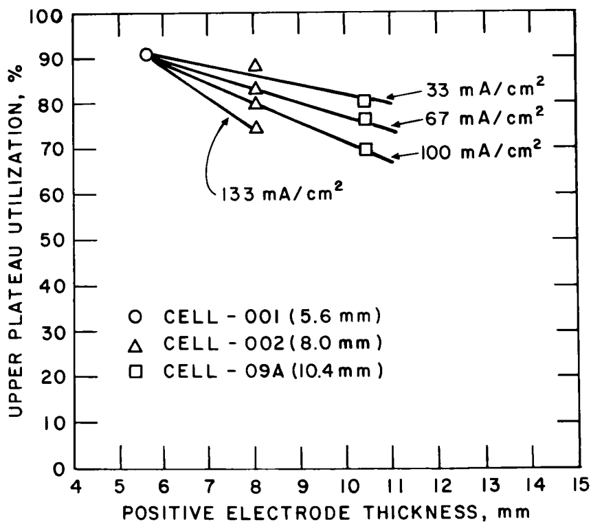
Fig. IV-13. Positive-Electrode Utilization as a Function of Thickness for Three Gould Li-Al/FeS 2 Cells
