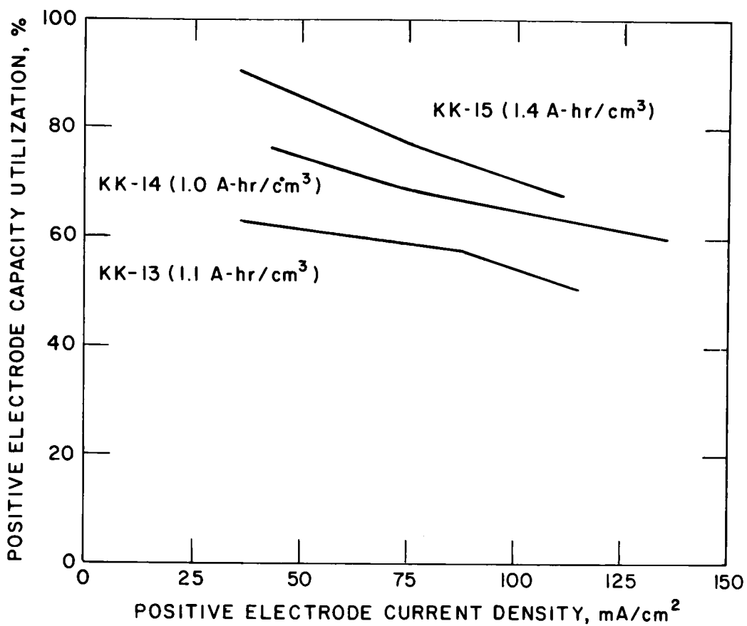
Fig. VI-7. Positive-Electrode Capacity Utilization of Carbon-Bonded Electrodes.
