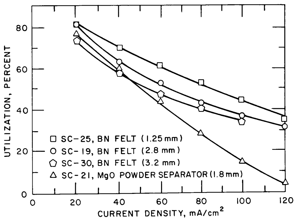
Fig. VII-3. Performance of Four Separator-Test Cells.
