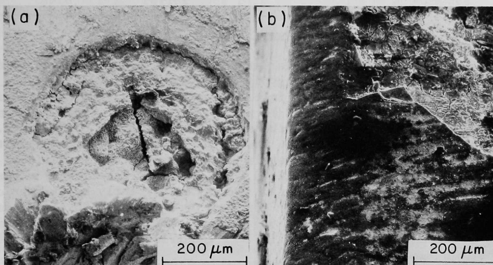
Fig. VII-2. Scanning Electron Micrograph of (a) \text{TiB}_2 Coated Sample after \sim 143 hr in the \text{FeS}_2/\text{LiCl-KCl} + Iron Boride Environment at 500^\circ\text{C} and (b) \text{TiN} Coated Sample after \sim 120 hr in the \text{FeS}_2/\text{LiCl-KCl} Environment at 500^\circ\text{C} . (Neg. No. MSD-65578)
