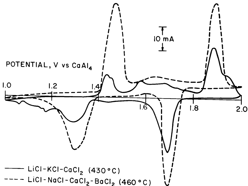
Fig. IX-2. Cyclic Voltammograms for \text{FeS}_2 Electrodes
