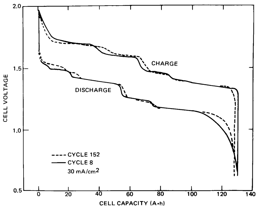
Fig. III-30. Voltage vs. Capacity of Cell REVC-10 at Cycles 8 and 152
