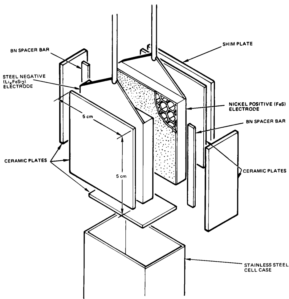
Fig. III-25. Powder Separator Test Cell
