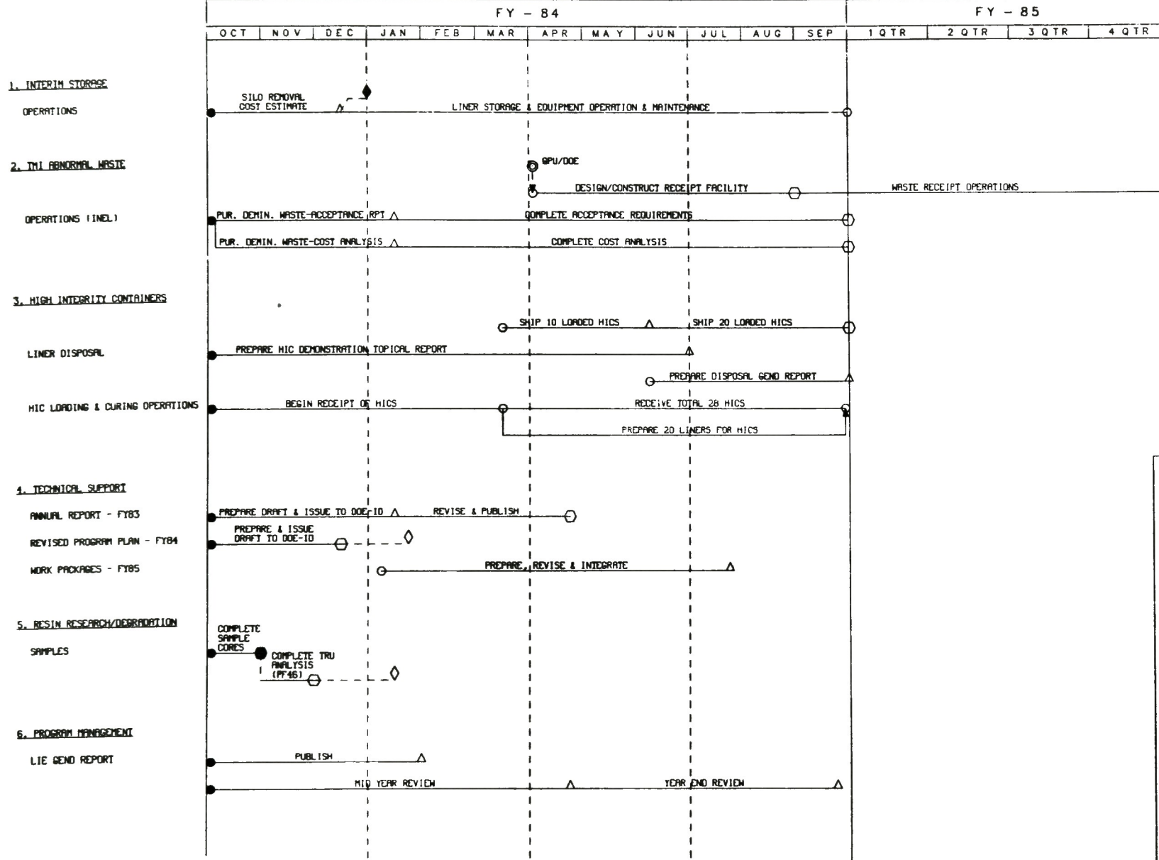
Figure 11. Generalized schedule of EPICOR and Waste Research and Disposition Program
