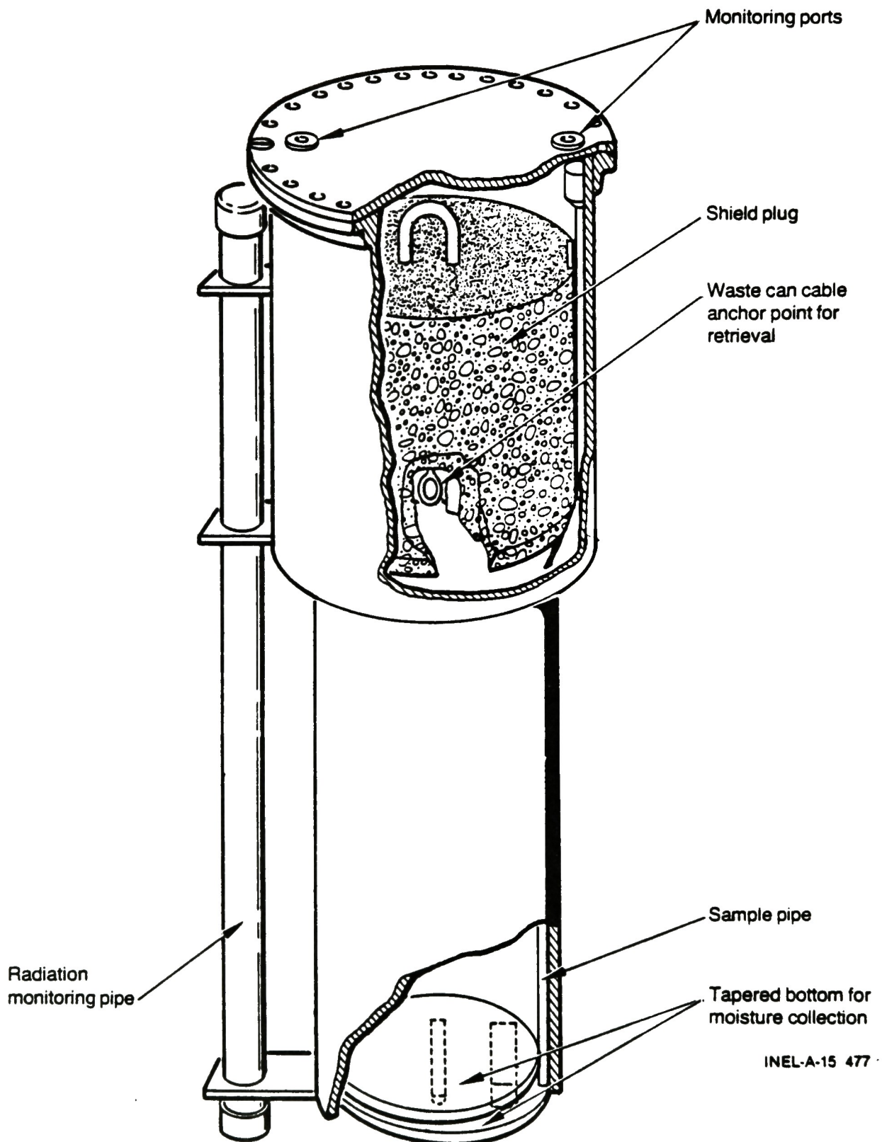
Figure 6. Typical 24-inch diameter intermediate level TRU waste vault at the RWM.
