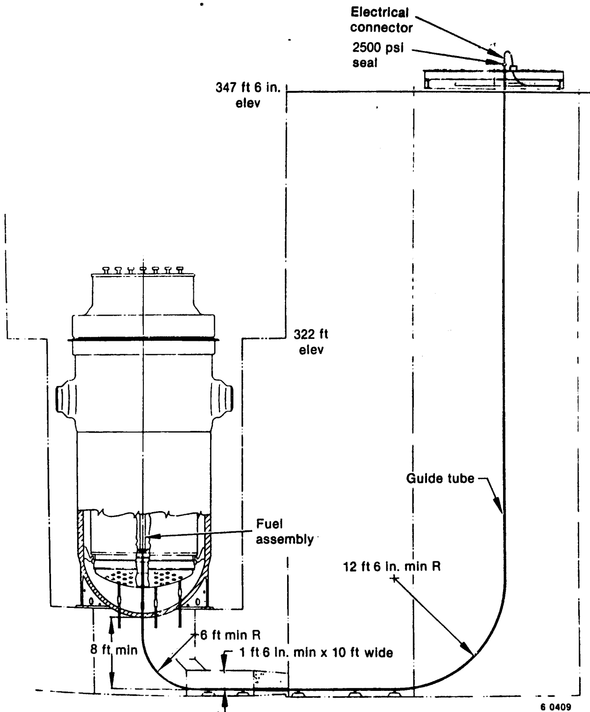
Figure 2. Schematic of typical incore instrument assembly.
