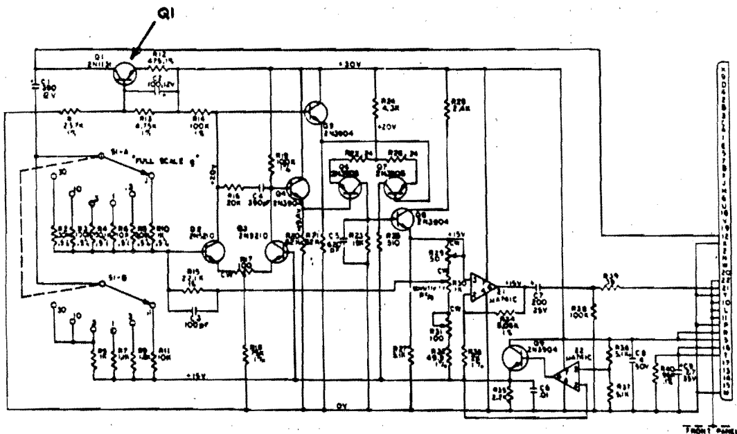
4. Model 4479.1 Line Driver Conditioner Schematic. Transistor Q1 is configured as a constant current generator providing the bias current to the Remote Charge Converter through pin 12 of the connector.
