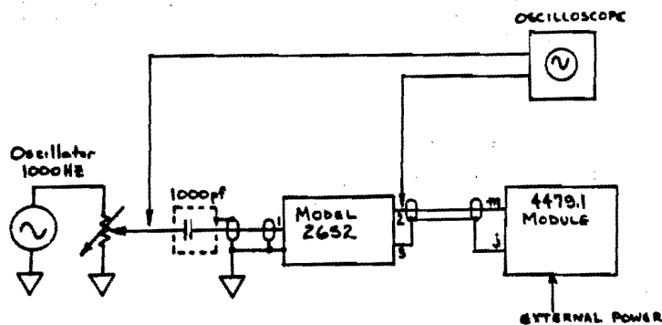
5. Model 2652 Set-up. This set-up is identical to that recommended by Endevco except that the Charge Converter output is monitored instead of the 4479.1 output. 6
