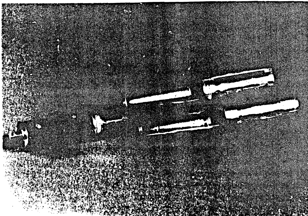
2. Disassembled Remote Charge Converter. The double shield is used to provide extra isolation from electromagnetic interference.
