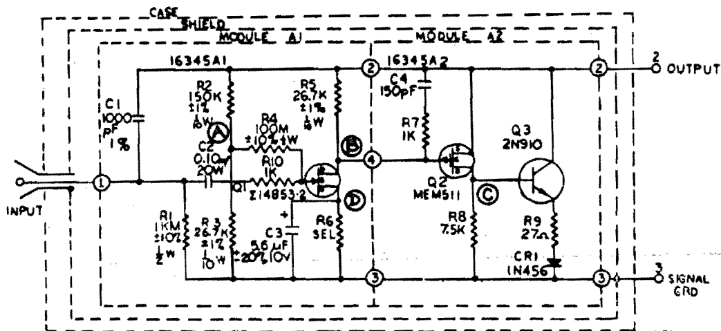
3. Charge Converter Schematic. The operating point measurements in Table 1 were made at the points indicated by letters A, B, C & D. Q2, an MEM 511 MOS transistor, was found to be degraded by radiation.
