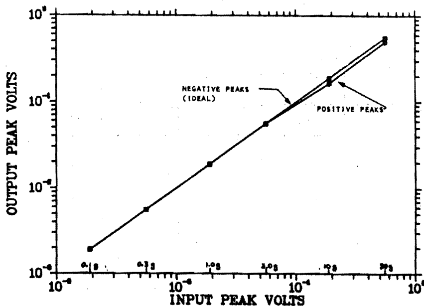
8. YM-AMP-7023 Transfer Characteristic. Unlike YM-AMP-7025 the negative going peaks are unattenuated. Only a slight attenuation is seen for positive going peaks.
