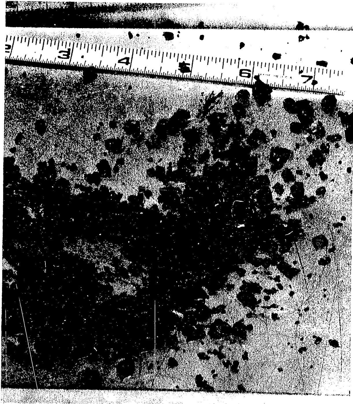
Figure 5. Photograph of TMI-2 core debris sample E9B.
