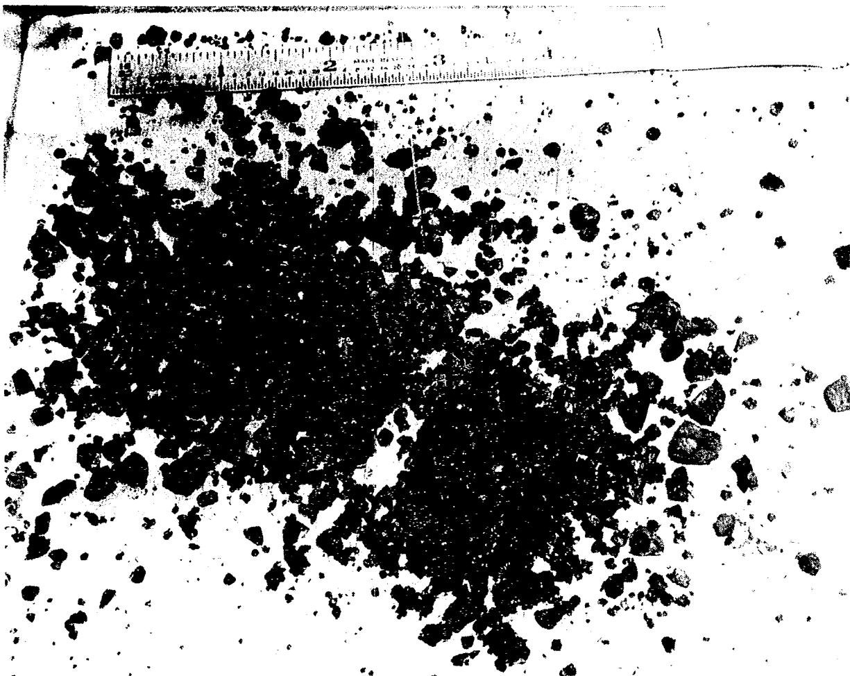
Figure 4. Photograph of TMI-2 core debris sample H8B.
