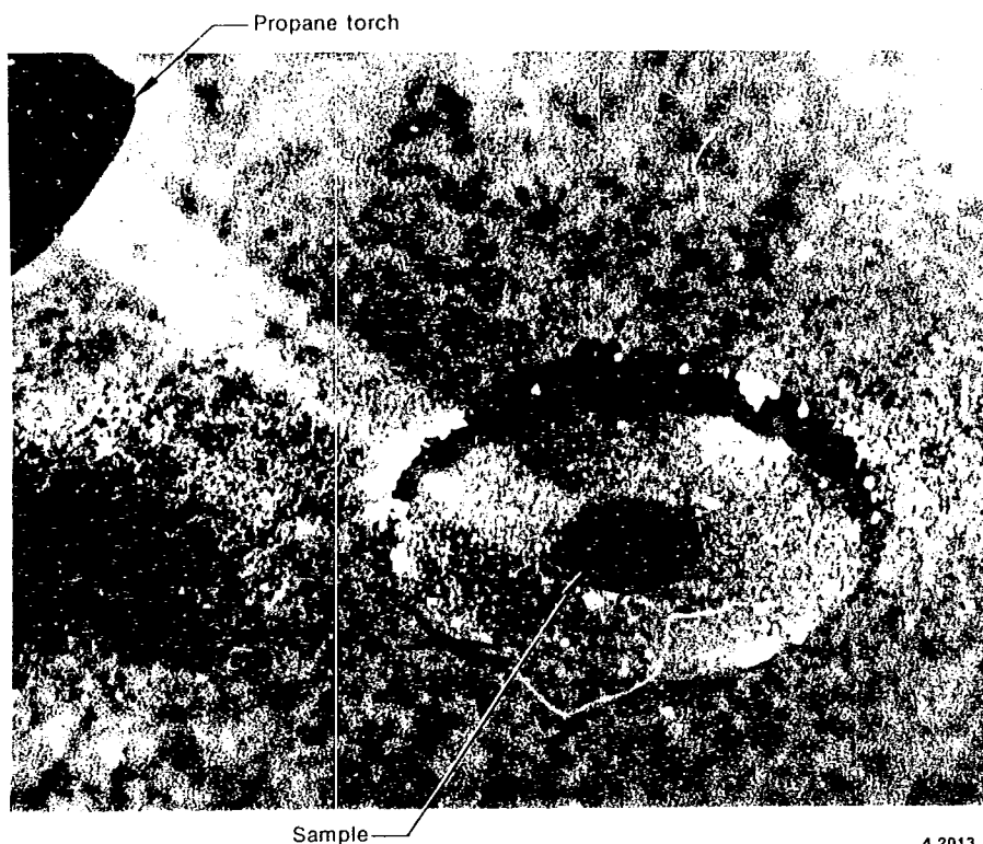
Figure 8. Photograph showing a flame pilot-ignition test.
