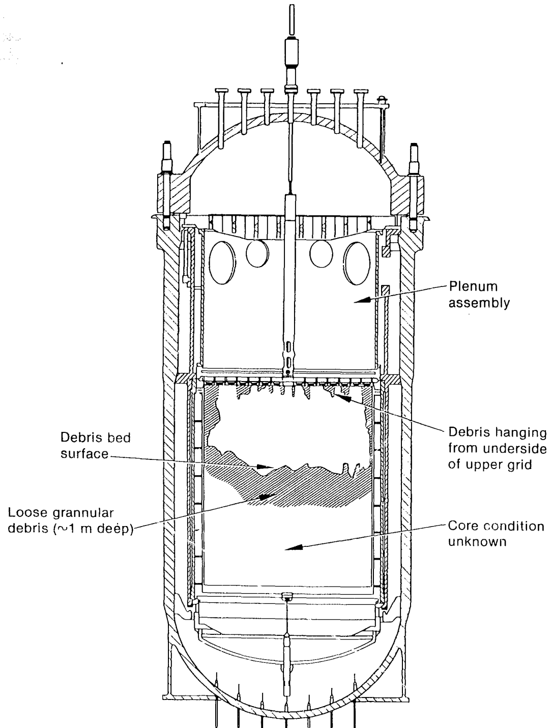
Figure 1. Schematic of the TMI-2 core damage.
