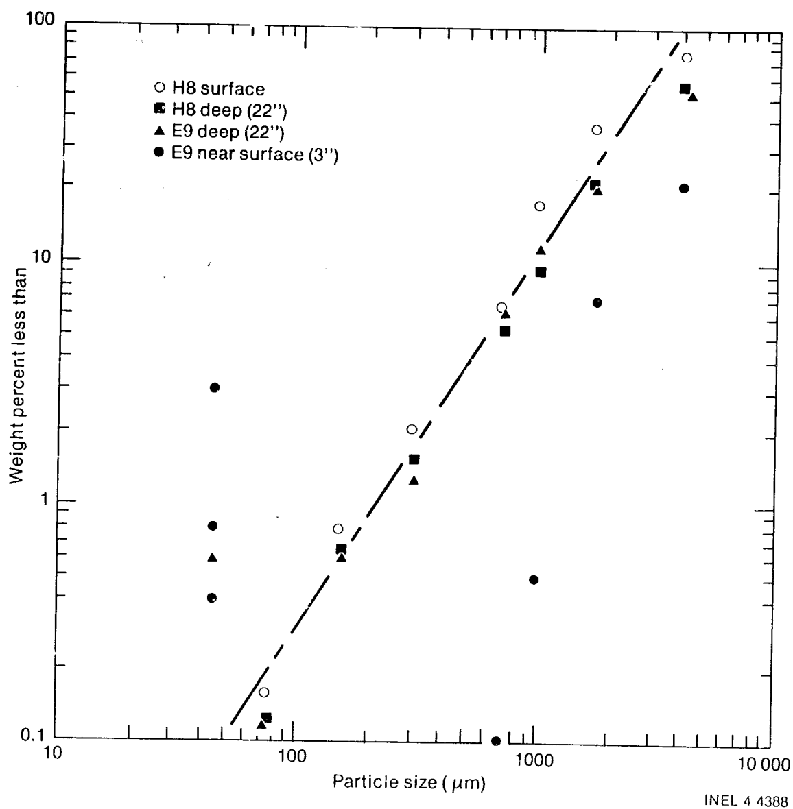
Figure 6. TMI-2 core debris particle size distribution.
