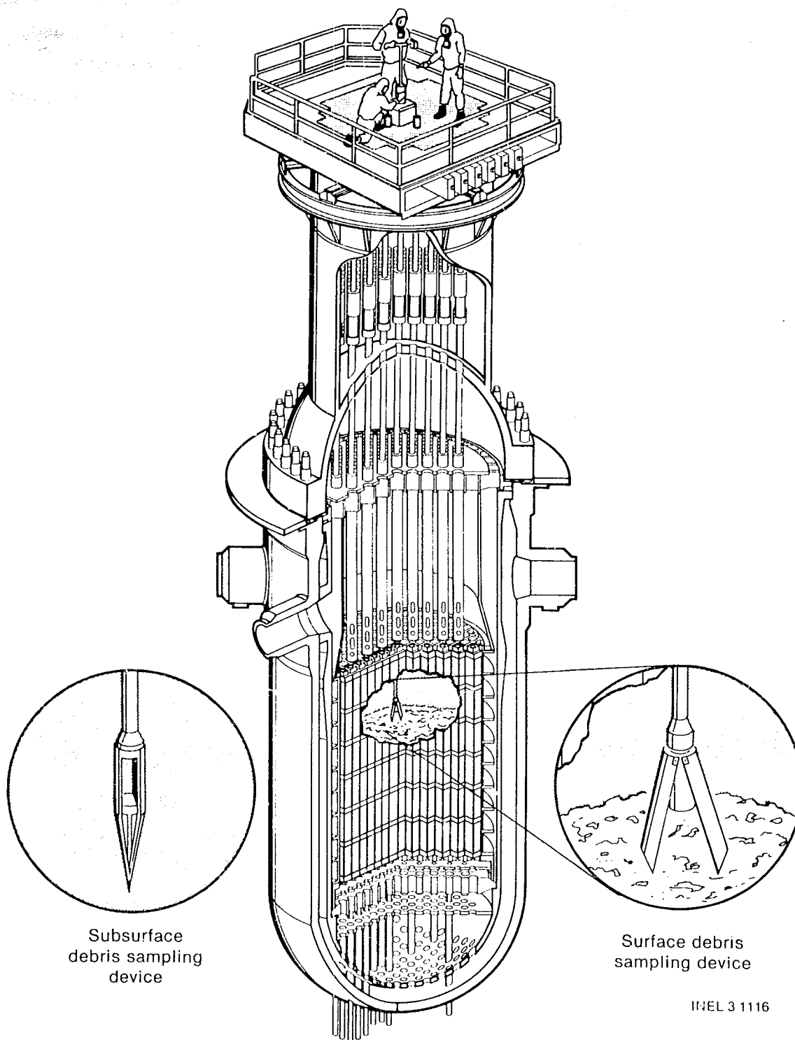
Figure 3. Schematic showing acquisition of the TMI-2 core debris samples.
