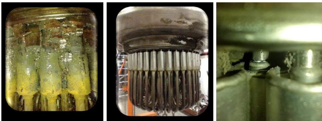
Figure 21. Images showing (left) oxide build-up on Stirling engine HX tubes, (center) Stirling engine HX tubes after cleaning, and (right) Stirling engine HX tube failure.
