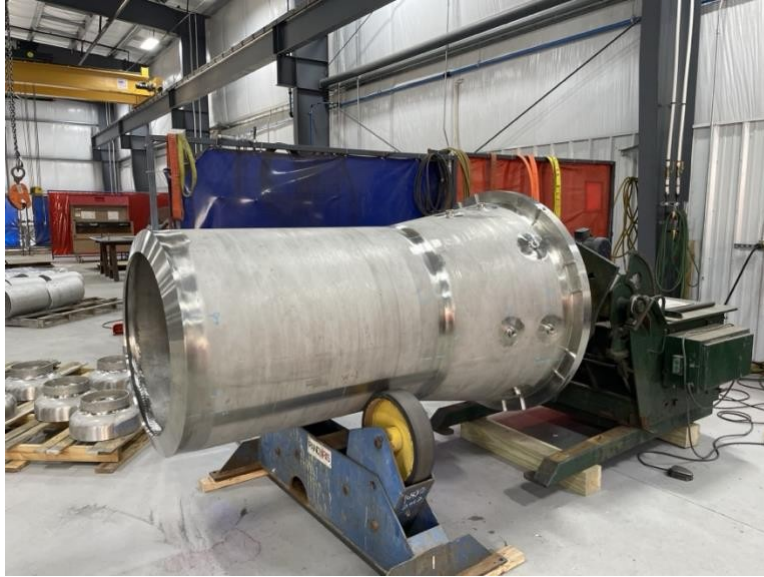
Figure 14. Completed MARVEL guard vessel.
