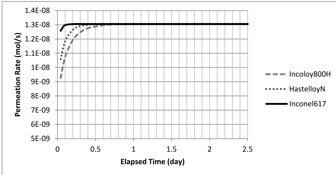
Figure 2. Selected alloys' permeation rate at 600^{\circ}\text{C} .
