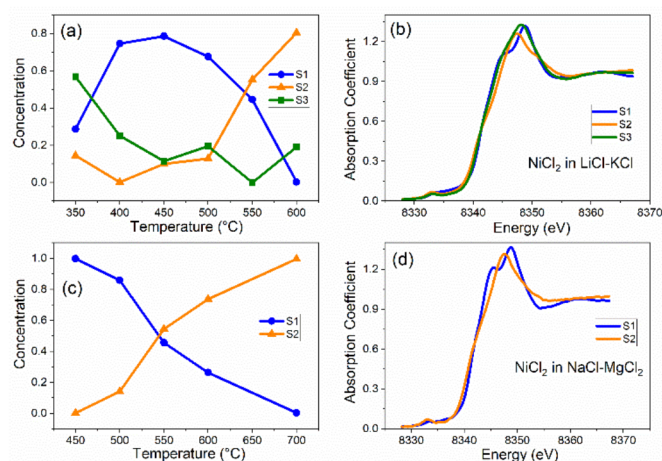
Fig. 3 XANES spectra corresponding to the three component states of Ni(II) (S1, S2, and S3, respectively) obtained by MCR-ALS analysis and their mixing fractions f for Ni(II) in LiCl-KCl (a,b) and in NaCl-MgCl 2 (c,d).
