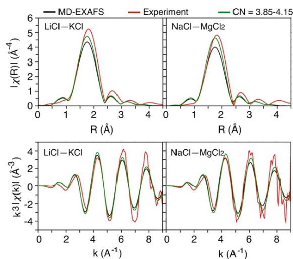
Fig. 8. Comparison of the experimental EXAFS spectra with the computed ones at 600 °C based on the statistical mechanical ensemble of all possible states sampled by AIMD simulations (MD-EXAFS) and a selection of states with coordination number around 4 (CN = 3.85-4.15).
