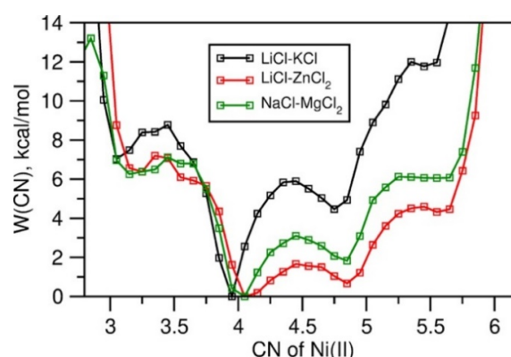
Fig. 6. Free energy plots of the coordination numbers of Ni(II) determined from the AIMD simulations at 600 °C as defined previously, 9 highlighting the influence of the polarizing power of the solvent salt cations on the distribution of the Ni(II) coordination geometries.
