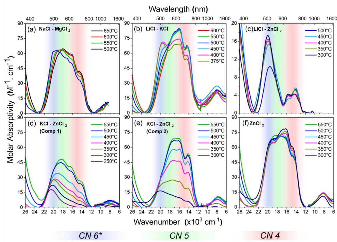
Fig. 4. Optical absorption spectra in UV-Vis-NIR range for Ni(II) species in: (a) 56:44 mol% NaCl-MgCl 2 , (b) 58:42 LiCl-KCl, (c) 22:78 LiCl-ZnCl 2 (note different vertical scale), (d) 45.3:55.7 KCl-ZnCl 2 , (e) 52.5:47.5 KCl-ZnCl 2 , and (f) neat ZnCl 2 as functions of temperature. Color-coded bands in each graph indicate the spectral regions where different coordination states have predominant absorption bands, as discussed in the text and labeled at the bottom of the figure. The regions are broadly defined and overlap to some extent.
