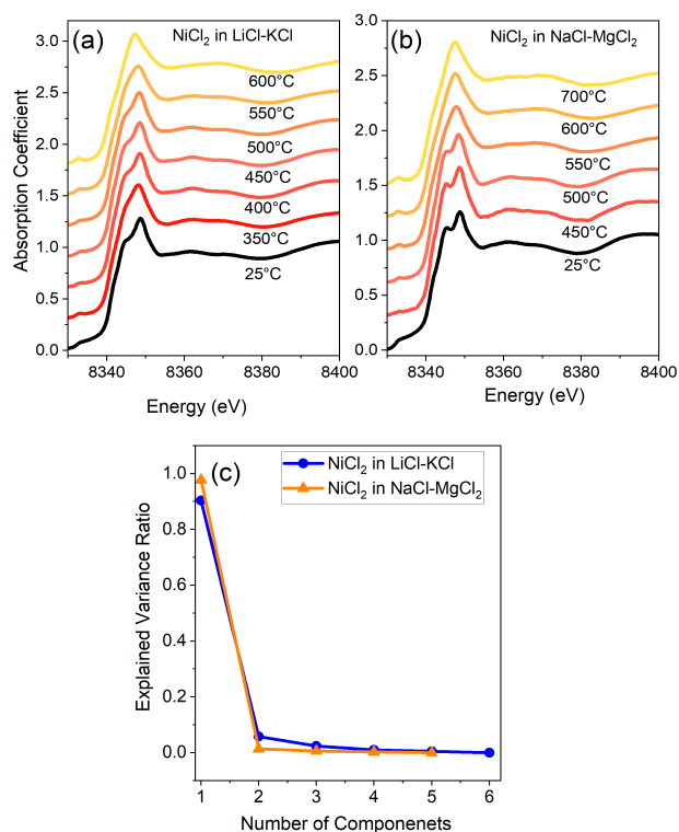
Fig. 2 XANES spectra of NiCl 2 in (a) LiCl-KCl and (b) NaCl-MgCl 2 at different temperatures. The scree plot of the PCA analysis of the XANES spectra above the respective melting points in a) and b) is shown in c).
