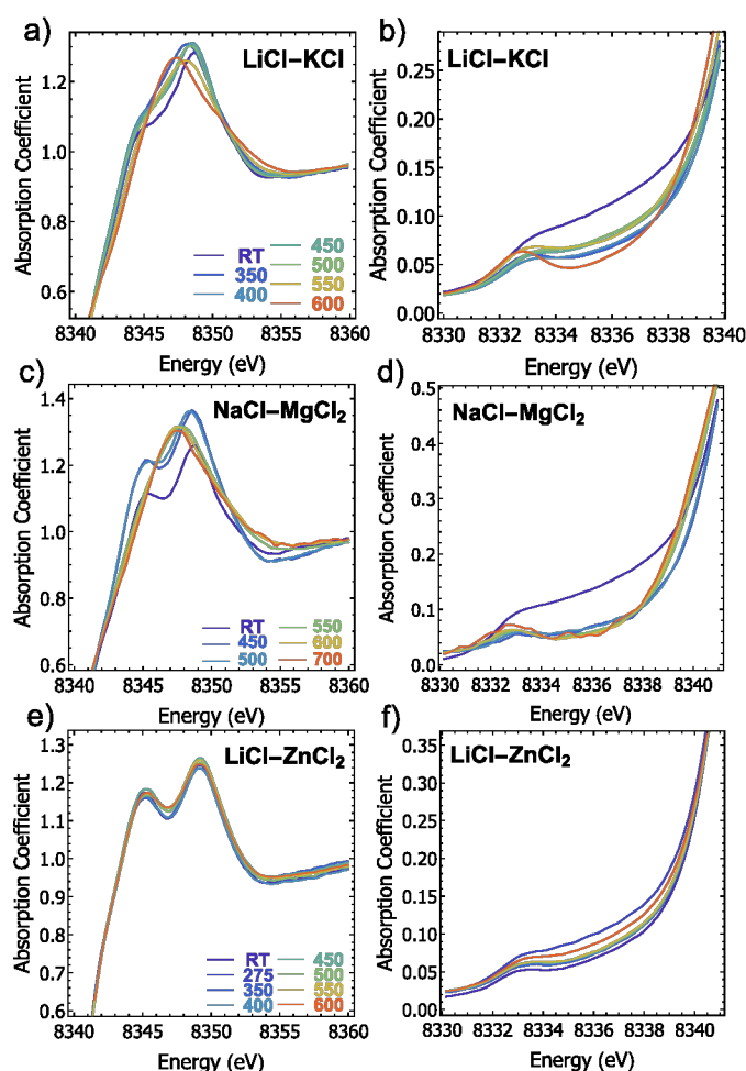
Fig. 1 XANES features in the main edge and pre-edge regions at the Ni K edge of NiCl 2 in LiCl-KCl (a,b), NaCl-MgCl 2 (c,d) and LiCl-ZnCl 2 (e,f). The colors correspond to different temperatures (in °C).
