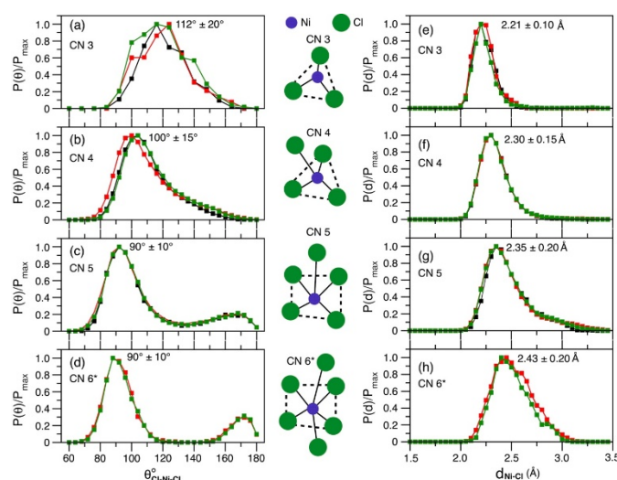
Fig. 7. Normalized probability distributions of Cl-Ni-Cl bond angles (a-d) and Ni-Cl distances (e-h) for nominal chloride coordination numbers CN 3, 4, 5 and 6* surrounding Ni(II), obtained from the AIMD simulations at 600 °C in the LiCl-KCl (black), ZnCl 2 -LiCl (red), and NaCl-MgCl 2 (green) mixtures. The most-likely bond angles and distances with standard deviations for each CN are given next to the peak heights. It should be noted that CN 6* is rarely sampled in the LiCl-KCl mixture, and therefore, the corresponding angle/distance distributions are not included in parts d and h.
