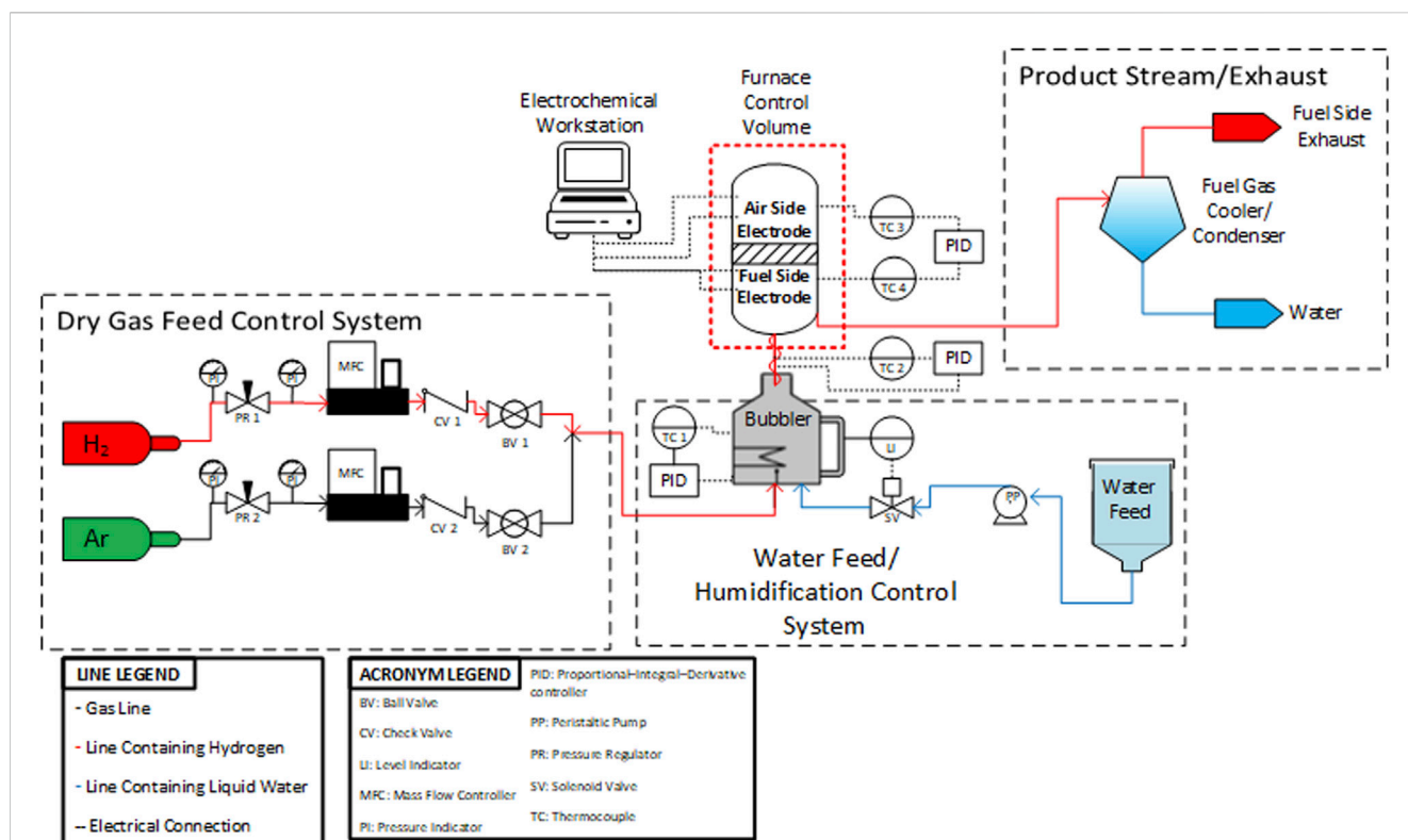
FIGURE 8 Full PID for an o-SOEC testing stand at INL.
