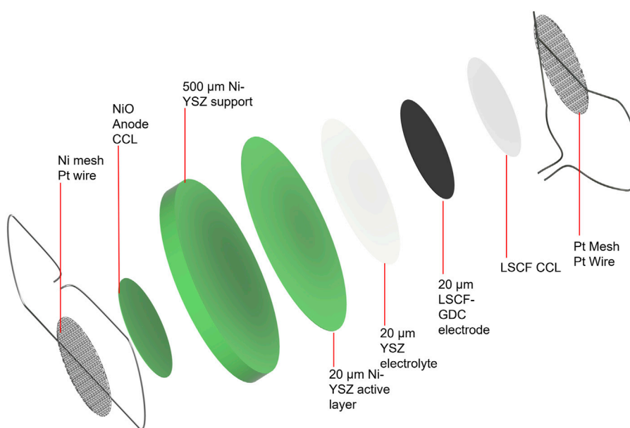
FIGURE 4 Exploded view of o-SOEC cell configuration with current collectors.
