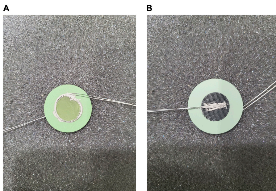
FIGURE 3 Current collectors attached on the (A) fuel electrode and (B) air electrode of a 1-inch o-SOEC cell.
