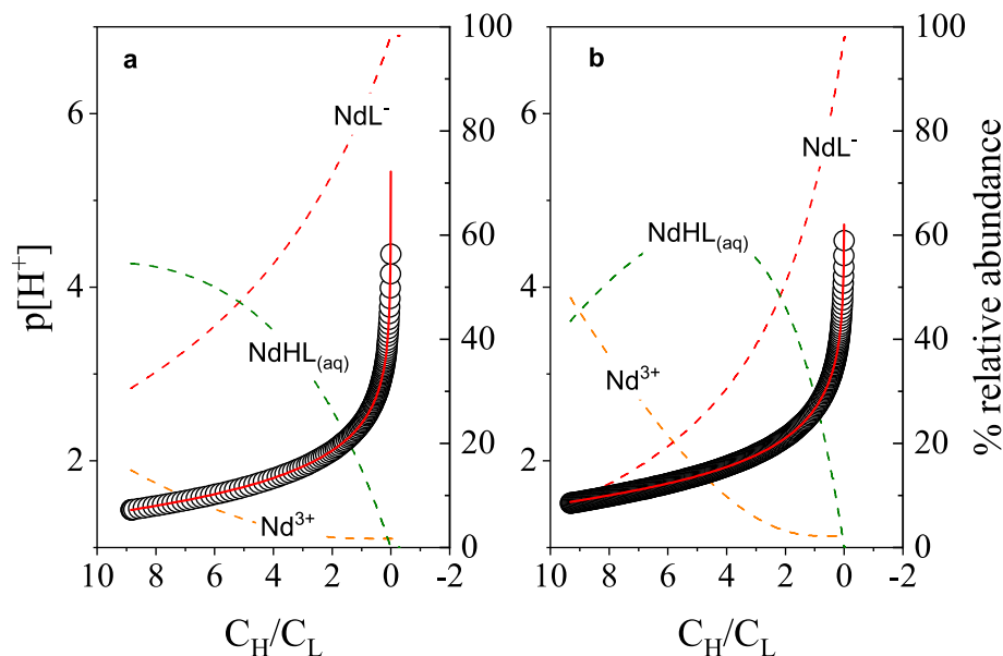
Figure 4. Potentiometric \text{p}[\text{H}^+] trends collected for complexometric titrations between \text{Nd}^{3+} and (A) \text{H}_4\text{octa} at T = 25.0 \pm 0.1 °C and I = 2.00 \pm 0.01 M (\text{Na}^+/\text{H}^+) \text{NO}_3 and (B) \text{H}_4\text{pya-peg} at T = 25.0 \pm 0.1 °C and I = 2.00 \pm 0.01 M (\text{Na}^+/\text{H}^+) \text{ClO}_4 . (A) Titrand: V_{\text{initial}} = 25.244 mL, C_{\text{H}_4\text{octa}} = 4.803 mM, C_{\text{H}^+} = 0.043 M, C_{\text{Nd}^{3+}} = 4.887 mM. Titrant: 0.397 M NaOH and 1.60 M \text{NaNO}_3 . (O) Experimental \text{p}[\text{H}^+] , (red solid line) calculated \text{p}[\text{H}^+] , (orange dashed line) \text{Nd}^{3+} , (green dashed line) \text{NdHL}_{(\text{aq})} , (red dashed line) \text{NdL}^- . (B) Titrand: V_{\text{initial}} = 10.153 mL, C_{\text{H}_4\text{pya-peg}} = 4.700 mM, C_{\text{Nd}^{3+}} = 4.841 mM, C_{\text{H}^+} = 0.044 M. Titrant: 0.125 M NaOH in 1.875 M \text{NaClO}_4 . (O) Experimental \text{p}[\text{H}^+] , (red solid line) calculated \text{p}[\text{H}^+] , (orange dashed line) \text{Nd}^{3+} , (green dashed line) \text{NdHL}_{(\text{aq})} , (red dashed line) \text{NdL}^- .
