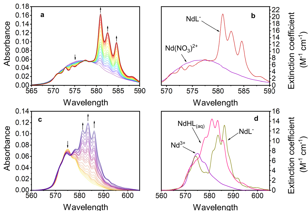
Figure 5. Changes in the optical absorption spectra for neodymium ion induced by (A) H_4octapa in 2.00 M (Na^+/H^+)NO_3 and (C) H_4pypa-peg in 2.00 M (Na^+/H^+)ClO_4 at T = 20 \pm 1 °C. (A) Titrand conditions: V_{initial} = 0.809 mL, C_{Nd^{3+}} = 7.62 mM, p[H^+]_{initial} = 1.40 . Titrant conditions: V_{titrant\ added} = 0.529 mL, C_{Nd^{3+}} = 7.65 mM, C_{H_4octapa} = 9.75 mM, p[H^+] \approx 6 . (C) Titrand conditions: V_{initial} = 0.801 mL, C_{Nd^{3+}} = 9.817 mM, p[H^+] = 1.61 . Titrant: C_{H_4pypa-peg} = 24.584 mM, C_{Nd^{3+}} = 9.913 mM, p[H^+] = 3.59 . The calculated molar absorptivities ( \epsilon_A ) are shown in panels (B) for H_4octapa species and (D) for H_4pypa-peg species.
