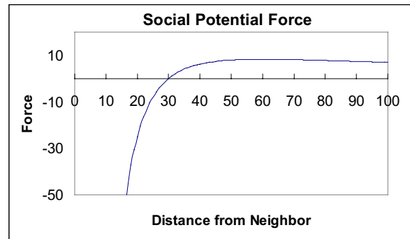
Figure 4: Social Potential Force Function
