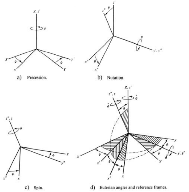
Fig. 5. Euler Angle Rotation from [1].
