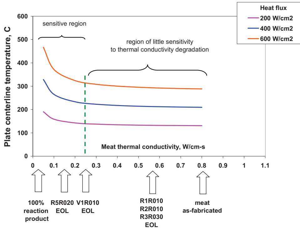
Figure 1. Effect of the meat thermal conductivity degradation on RERTR plate temperature at various heat flux levels. Note that the curves remain nearly flat until thermal conductivity falls to 0.25 W/cm-s (arbitrary threshold is marked with the green dashed line). Thermal conductivities of 100% reaction product (lower limit), as fabricated fuel meat (upper limit), and EOL thermal conductivities of selected plates from RERTR-6 experiment are shown for the reference with arrows on X-axis.
