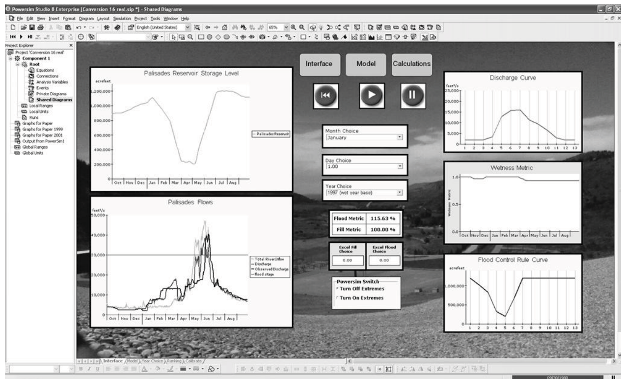
Figure 11: Illustration of the interface during simulation
