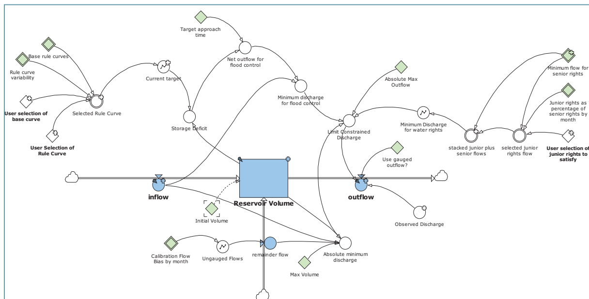
Figure 4: Diagram of the reservoir model.
