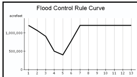
Figure 6: Initial Flood Rule Curve for one year
