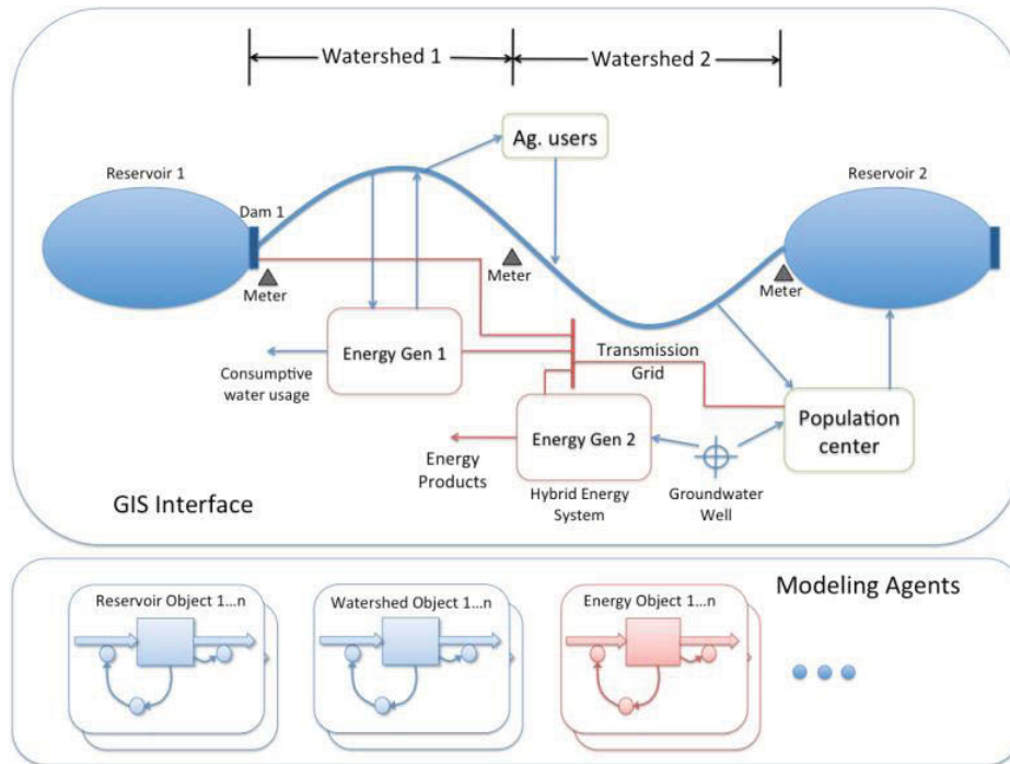
Figure 1: Concept diagram of energy and water system aggregation using system dynamics and object-oriented modeling.
