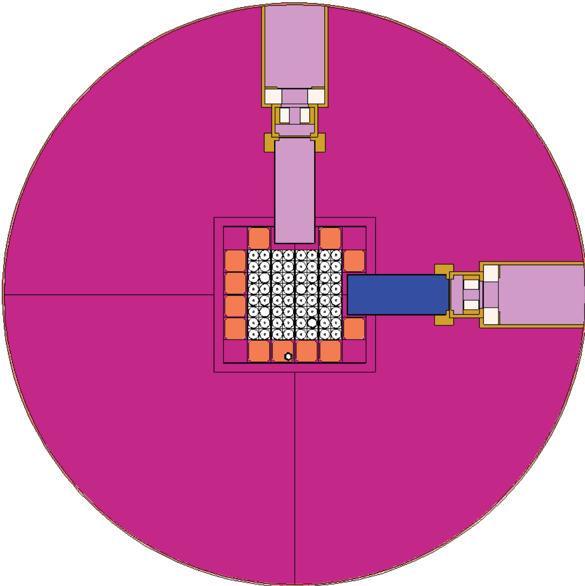
Figure C.2. Horizontal Cross Section of Detailed NRAD Model at Fuel Midplane (60-Fuel-Element Core).
