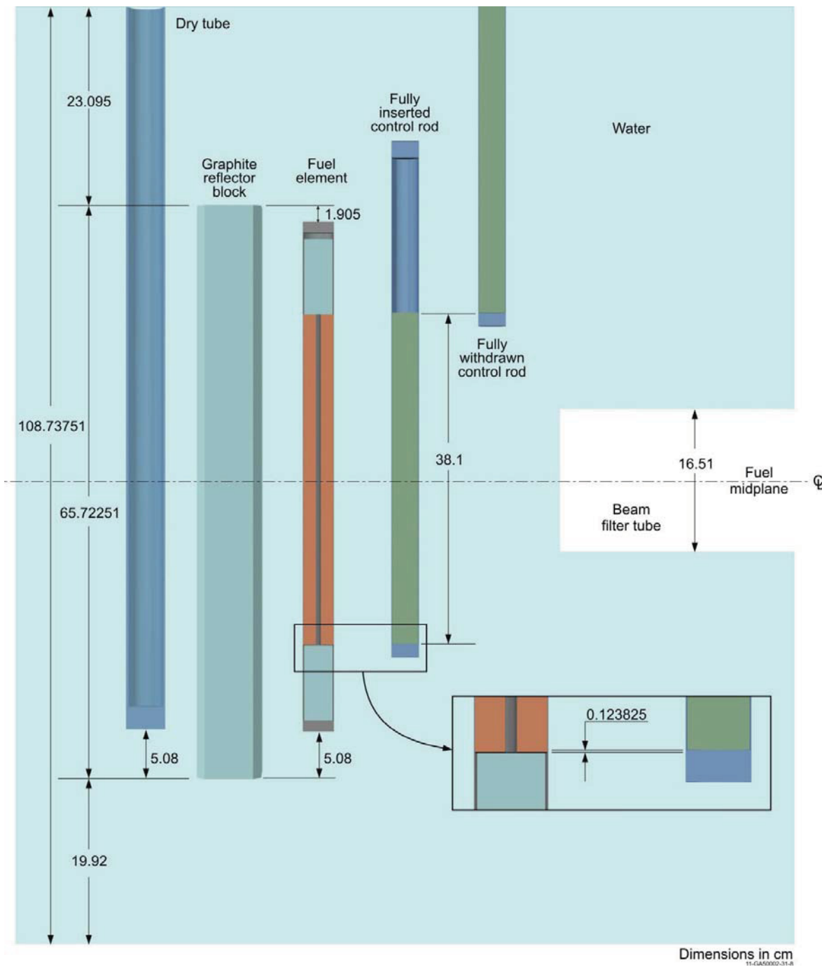
Figure 3.19. NRAD Reactor Core Reference Vertical Placement with Experiment Dry Tube.
