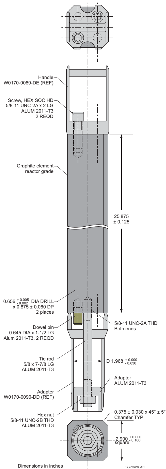
Figure 1.36. NRAD Graphite Reflector Assembly.
