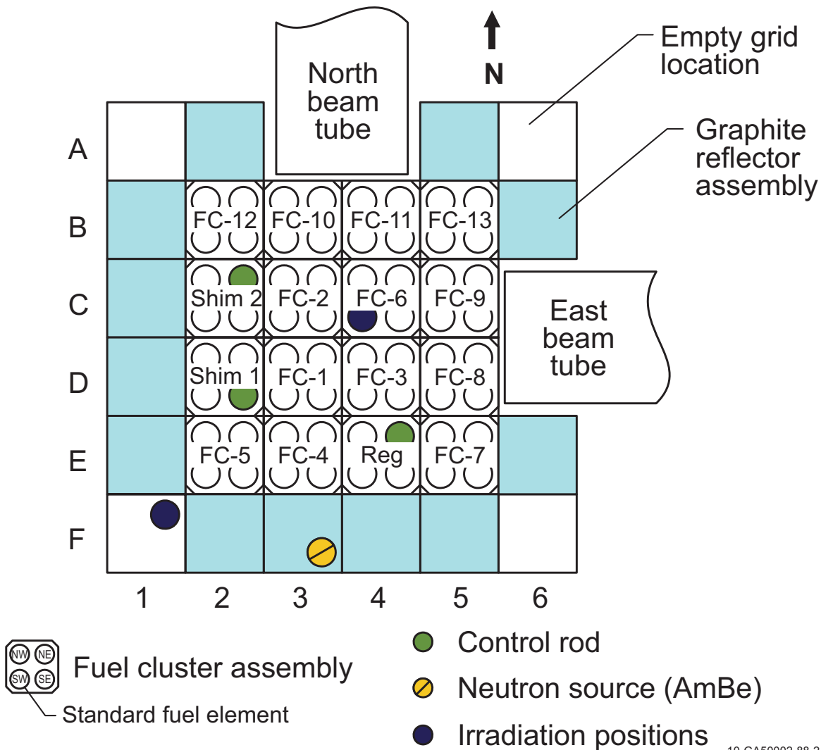
Figure 1.58. Fully Loaded Core Critical Configuration (60 Fuel Elements).
