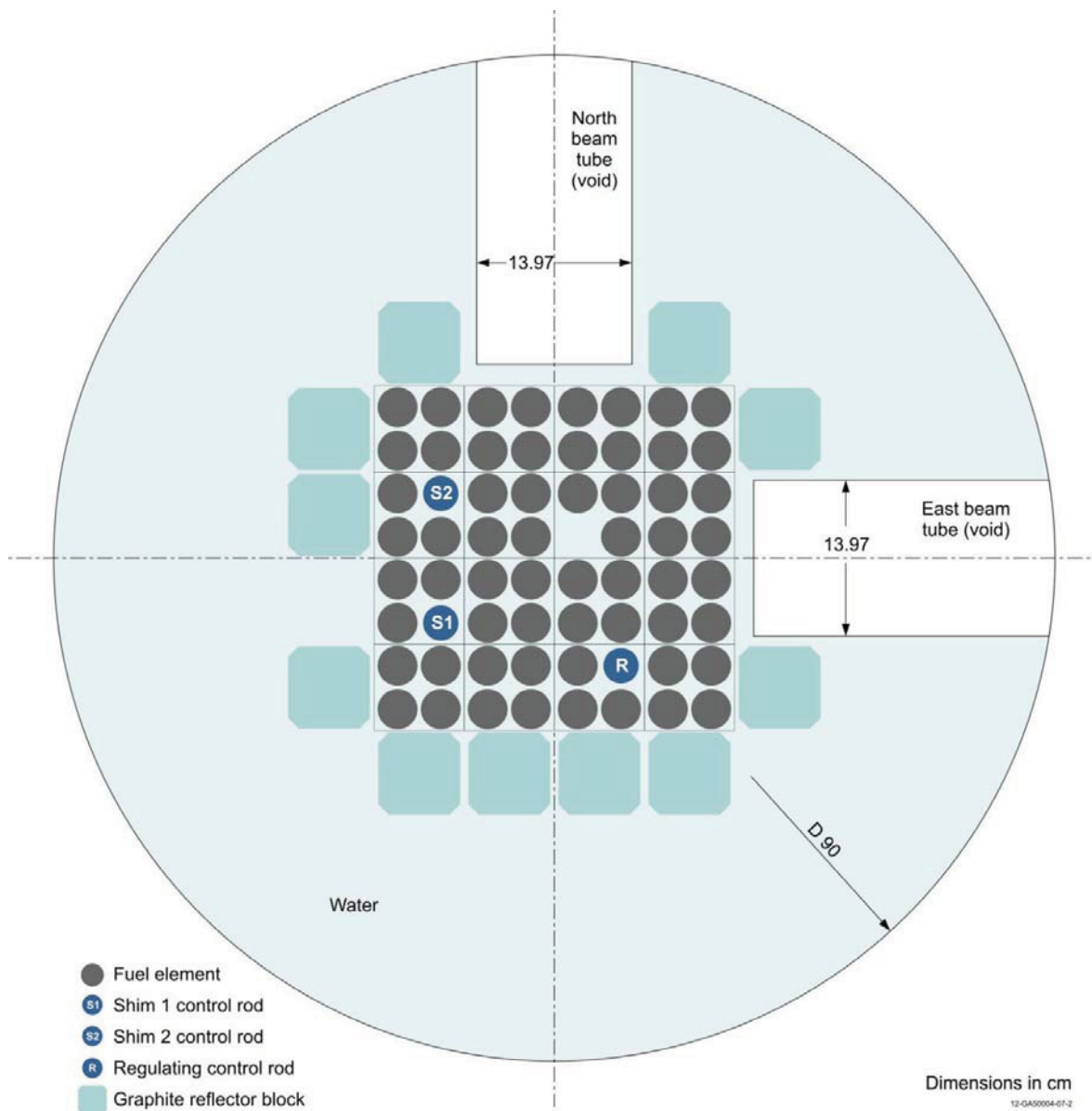
Figure 3.14. Midplane Cross Section View of NRAD Reactor Core without Block in Position D-1.
