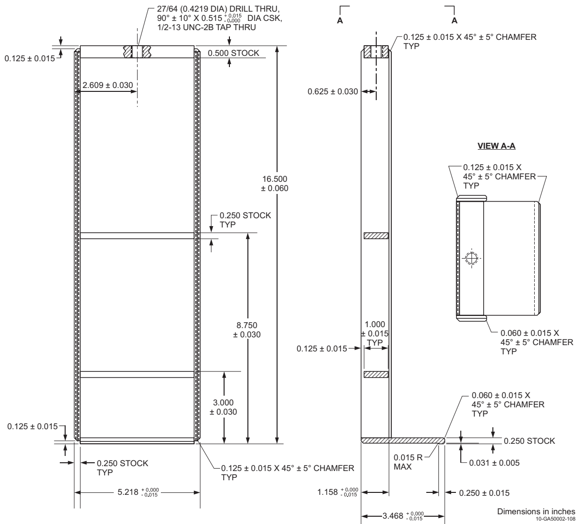
Figure 1.46. Aperture Block Guide.
