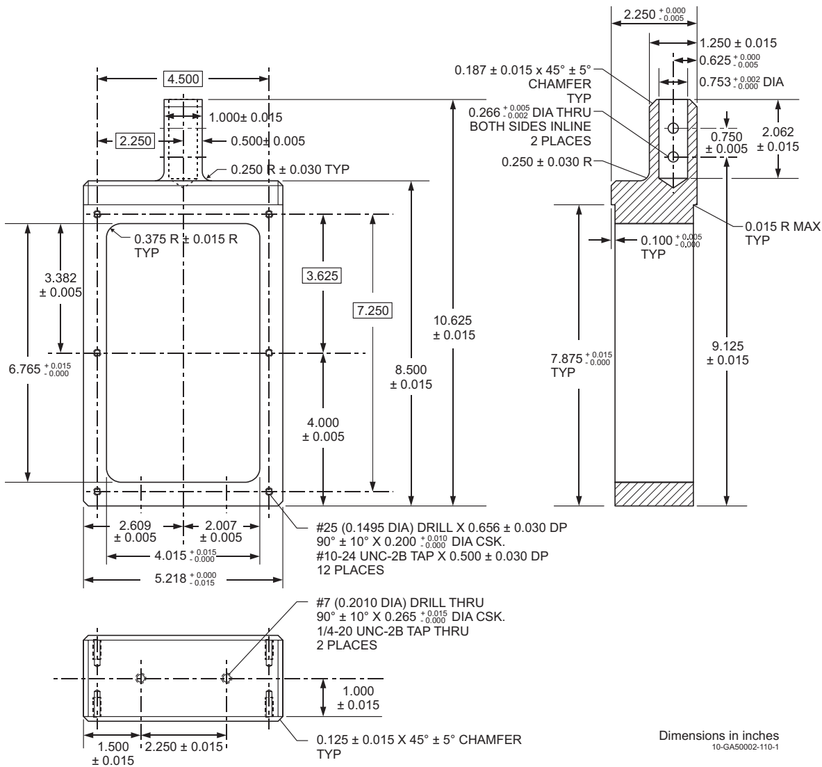
Figure 1.45a. Aperture Block Frame.
