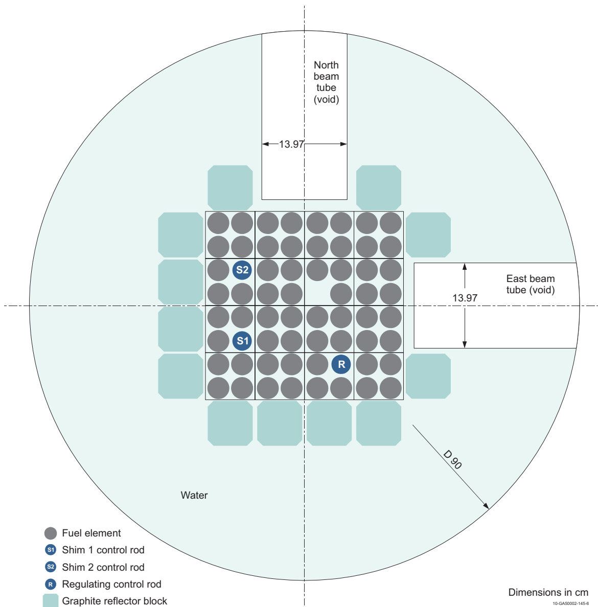
Figure 3.8b. Midplane Cross Section View of NRAD Reactor Core (Case 2).
