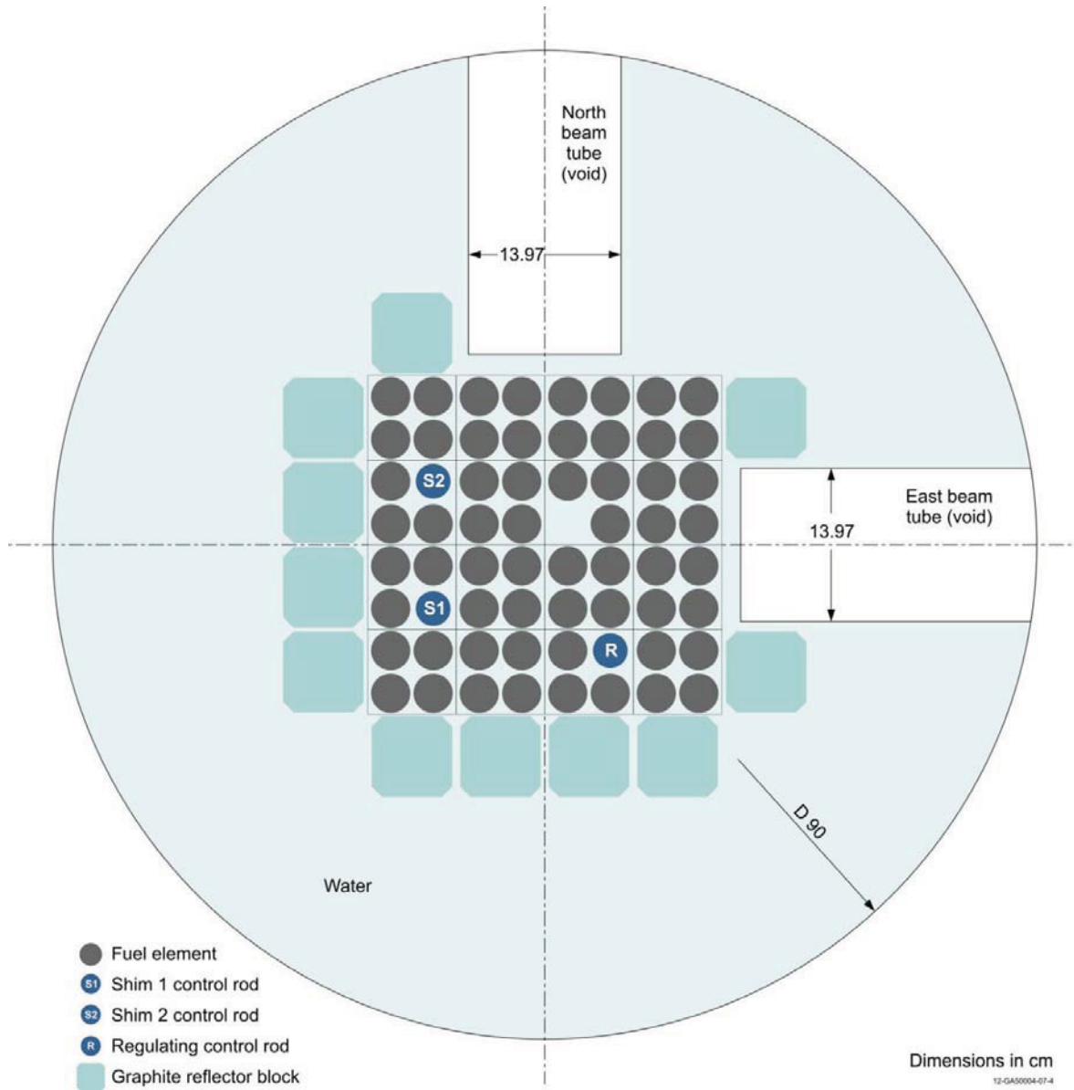
Figure 3.12. Midplane Cross Section View of NRAD Reactor Core without Block in Position A-5.
