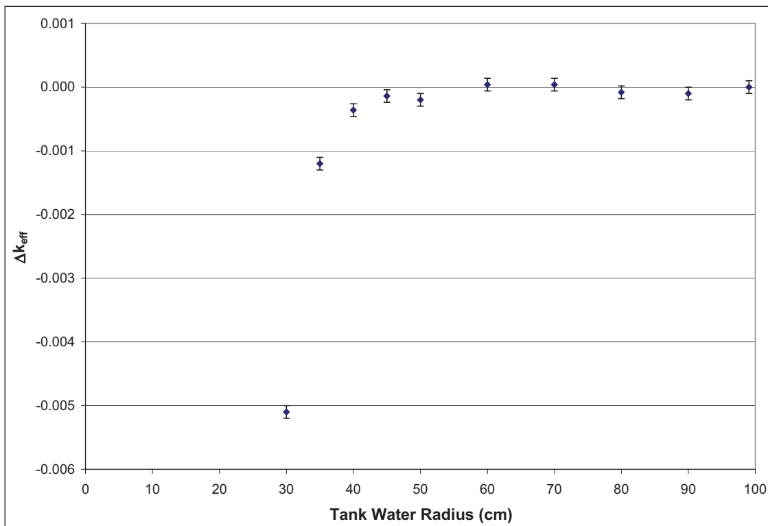
Figure 3.1. Effective Bias Due to Tank Water Radial Boundary (Case 2).
