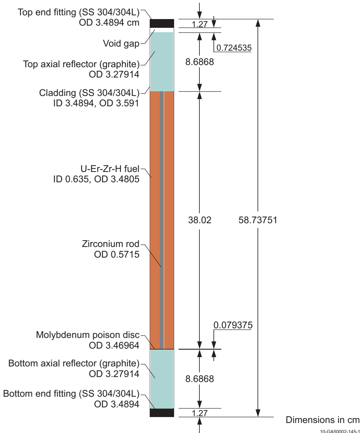
Figure 3.4. TRIGA Fuel Element.
