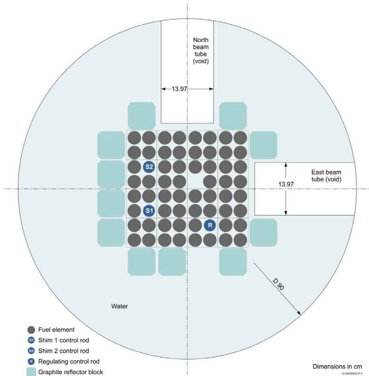
Figure 3.15. Midplane Cross Section View of NRAD Reactor Core without Block in Position F-4.
