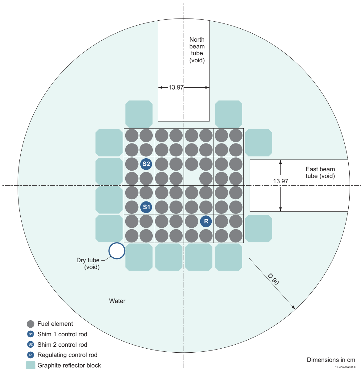
Figure 3.17. Midplane Cross Section View of NRAD Reactor Core with Experiment Dry Tube.
