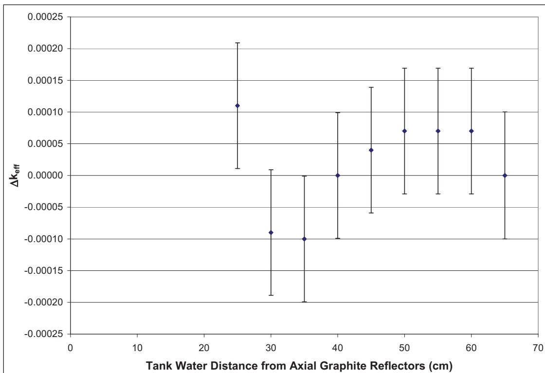
Figure 3.2. Effective Bias Due to Tank Water Axial Boundary (Case 2).
