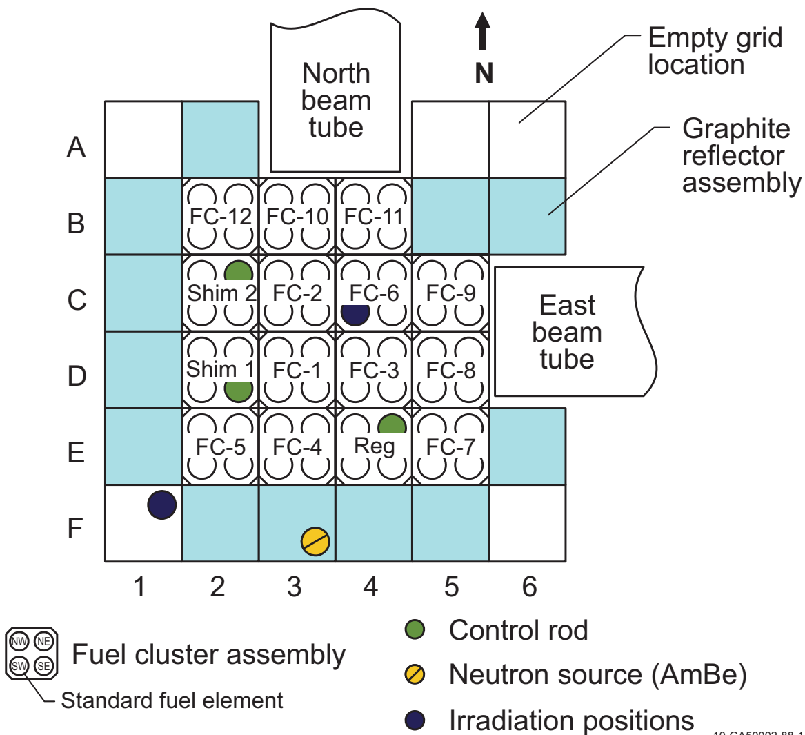
Figure E.3. Initial Core Critical Configuration (56 Fuel Elements).
