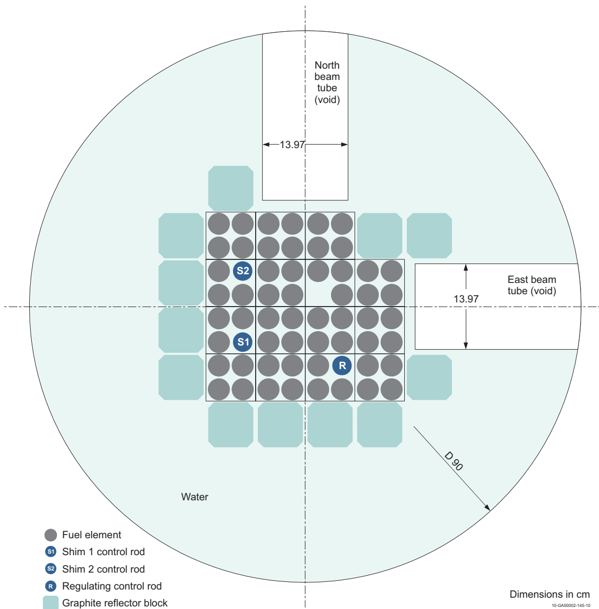
Figure 3.8a. Midplane Cross Section View of NRAD Reactor Core (Case 1).
