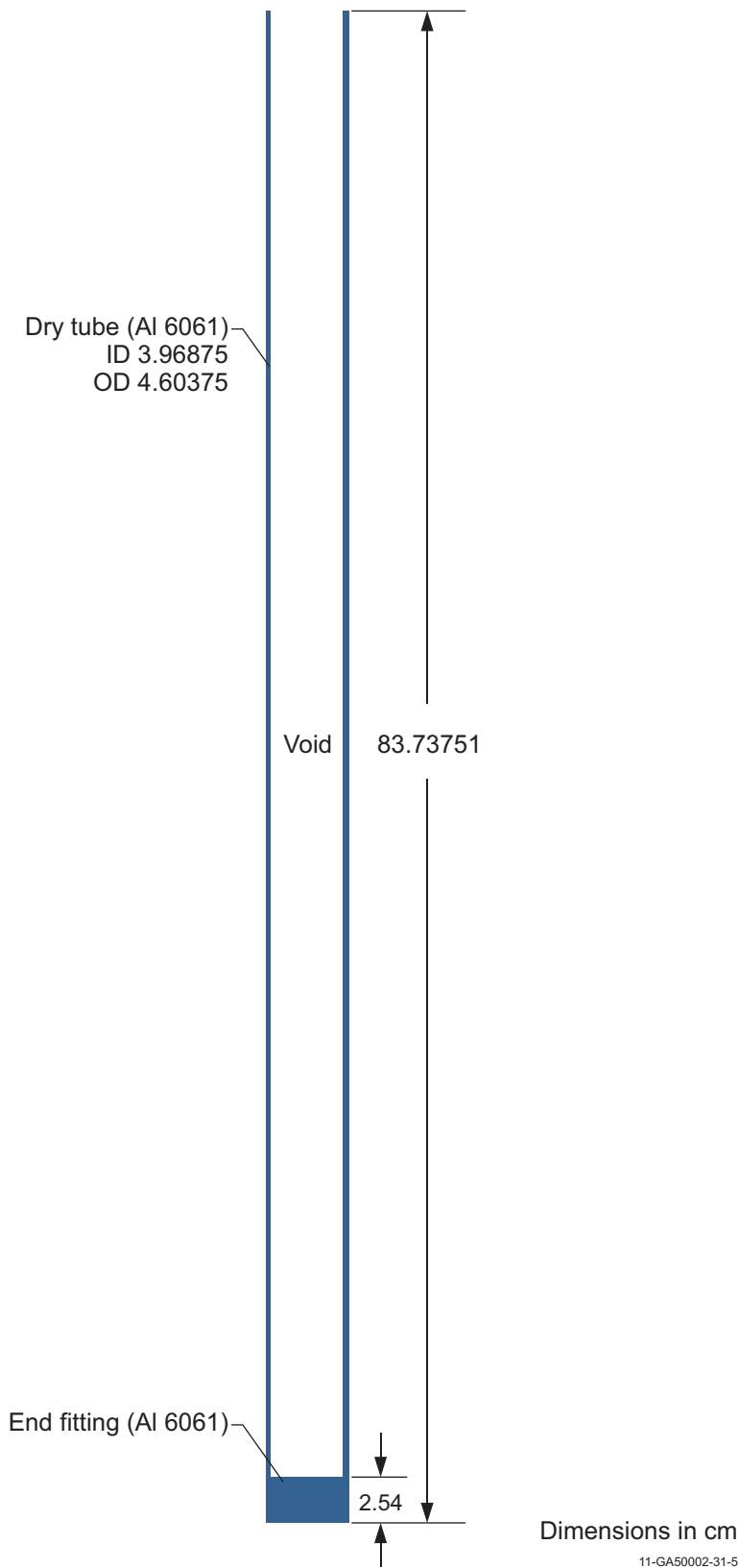
Figure 3.16. Experiment Dry Tube.
