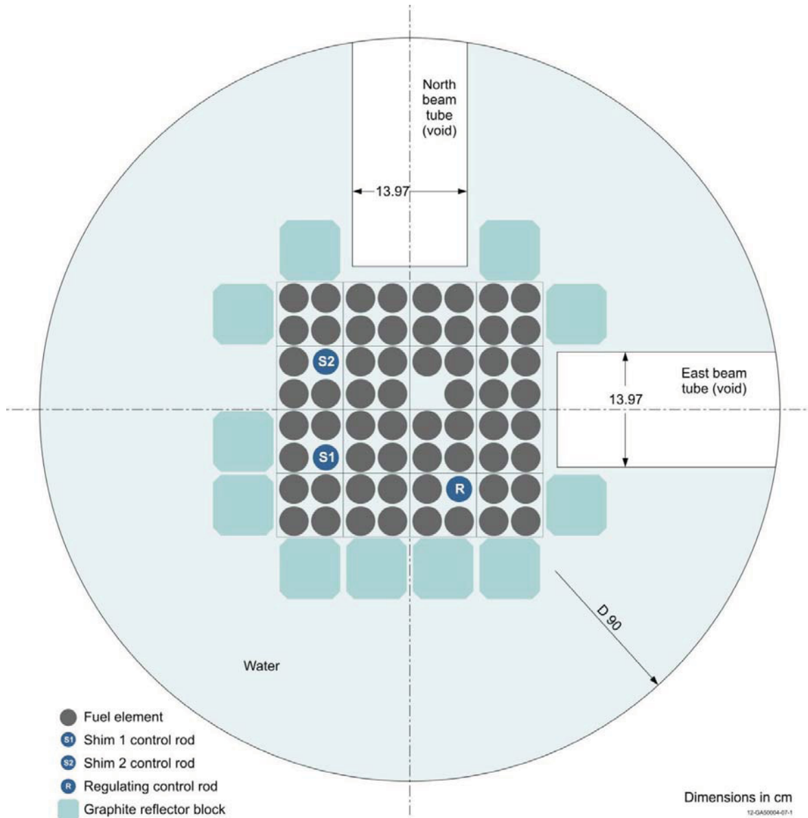
Figure 3.13. Midplane Cross Section View of NRAD Reactor Core without Block in Position C-1.
