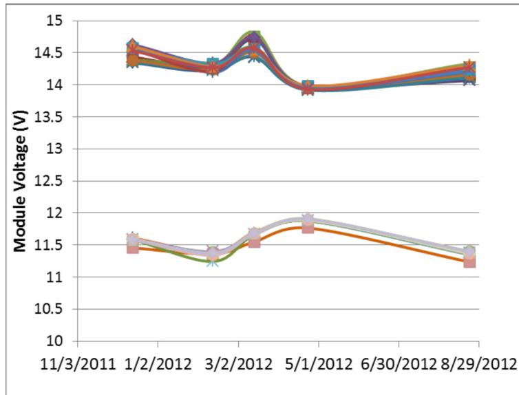
Figure 52. Maximum and minimum battery module voltage obtained for the road test from December 2011 to August 2012.
