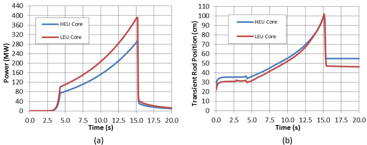
Figure 3. (a) Power-time History of the M8CAL HEU Core Bounding Shaped Transient Case (5.95% Reactivity) and Corresponding LEU Shaped Transient Needed for the Same TED and (b). Transient Rod Motion during the M8CAL HEU Core Bounding Shaped Transient (5.95% Reactivity) and Corresponding LEU Shaped Transient Needed for the Same TED.
