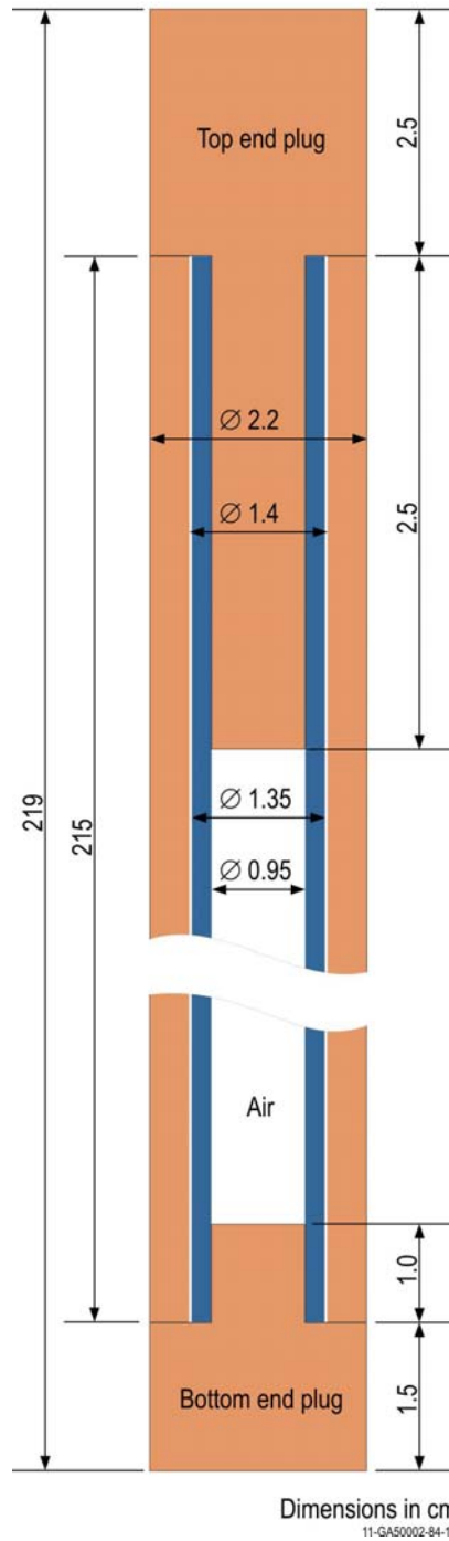
Figure 3.1-10. Axial View of Withdrawable Control Rod.
