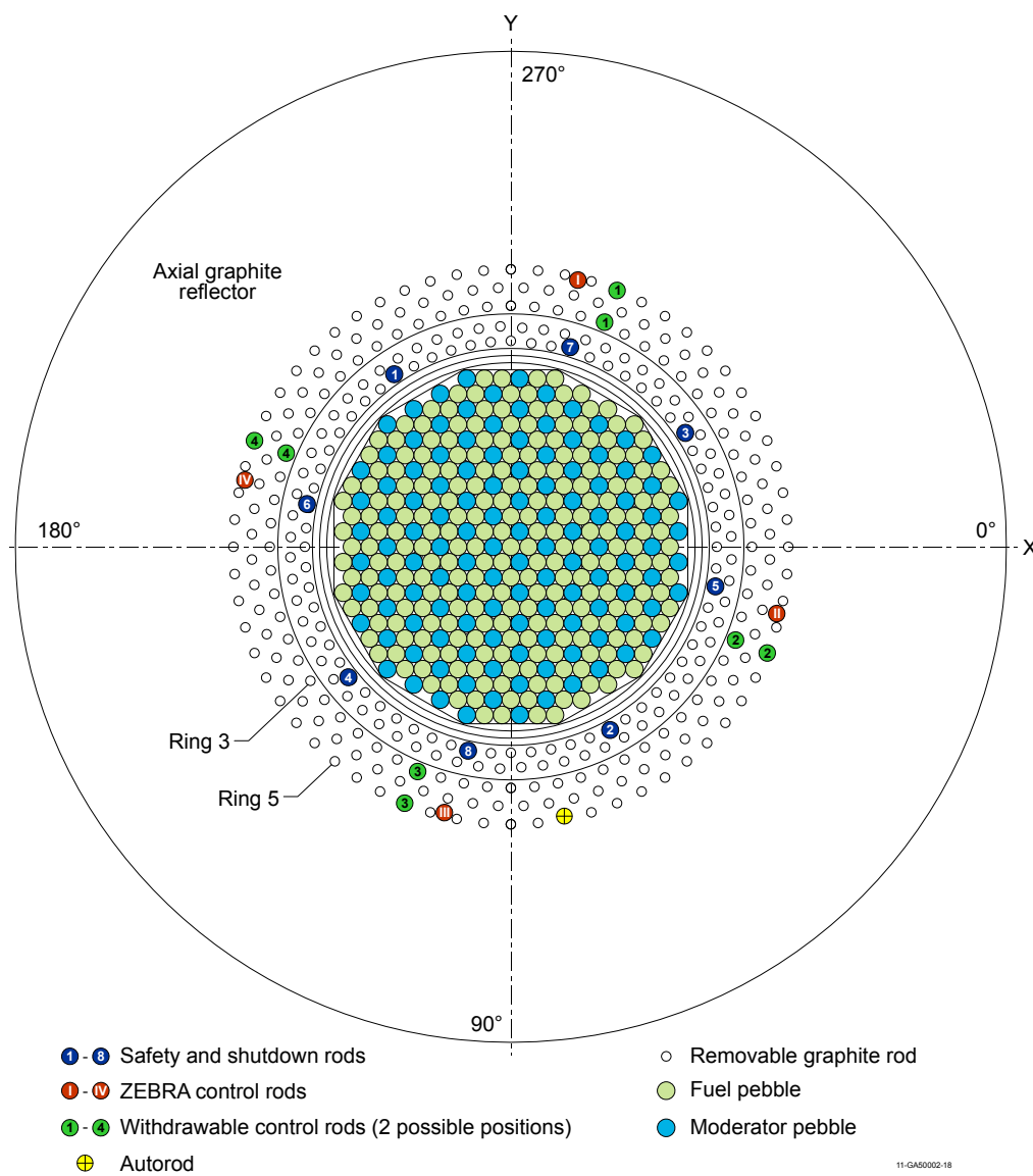
Figure 1.1-2a. HTR-PROTEUS control rod positions and bore hole locations (derived from Ref. 2).
