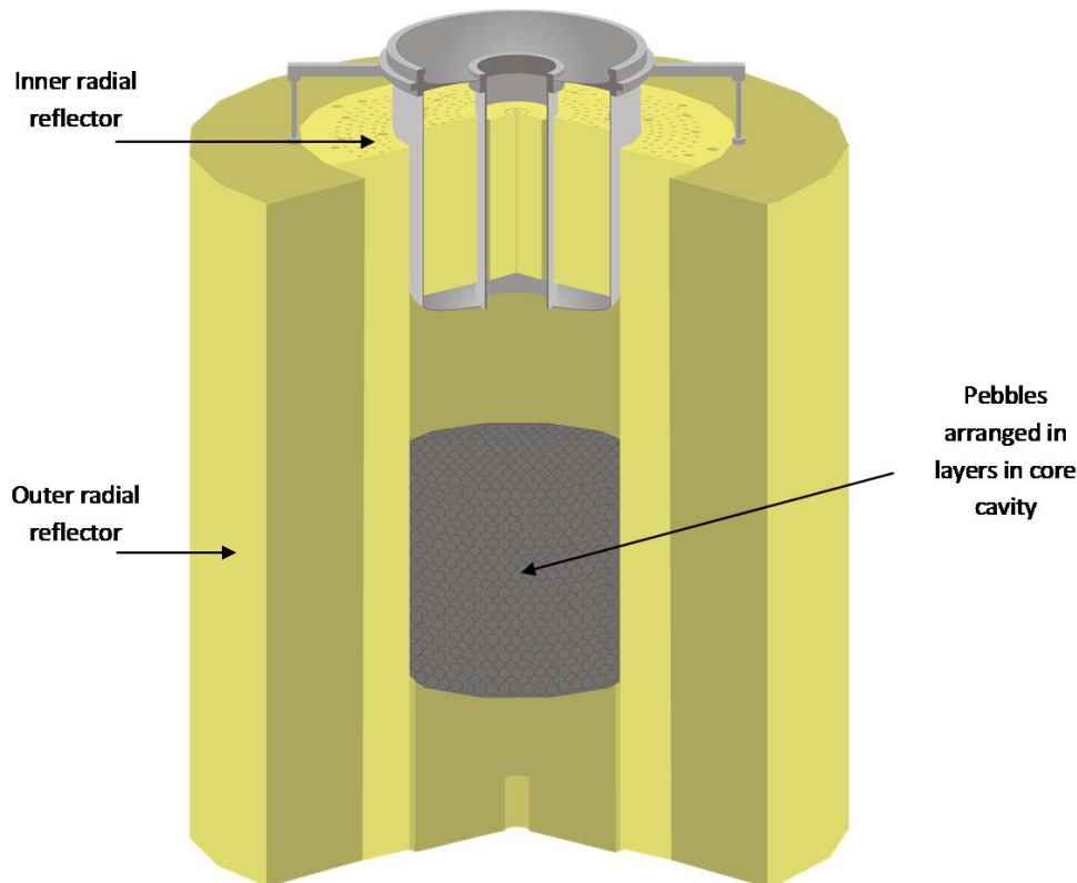
Figure 1.0-1. Generic HTR-PROTEUS configuration (derived from Ref. 2).
