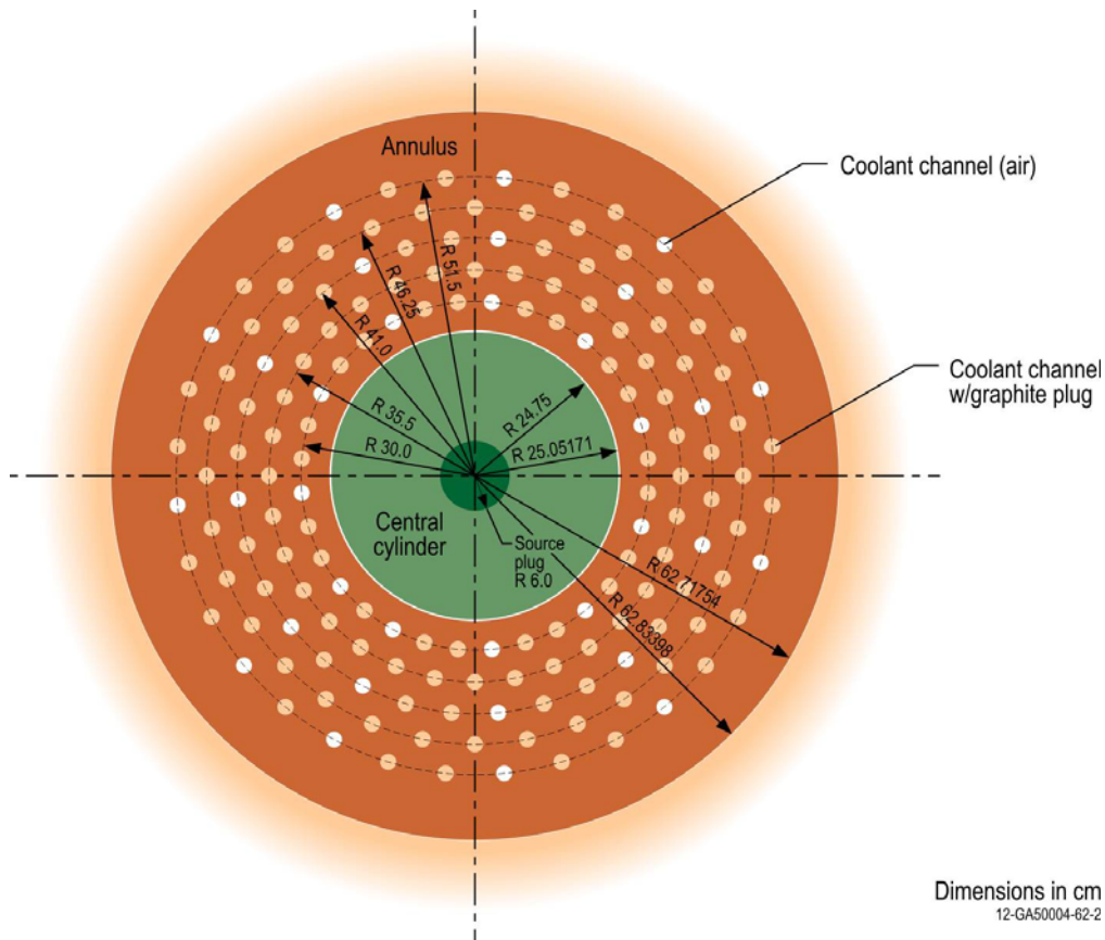
Figure 3.1-5. Lower Axial Reflector for Case 4 (Core 8).
