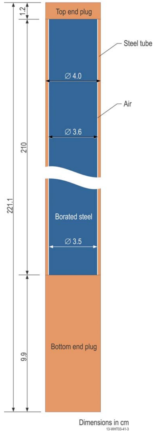
Figure 3.4-2. Axial View of Safety/Shutdown Rod.
