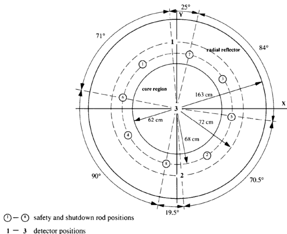
Figure 1.4-6. Horizontal Cross Section Indicating Radial and Azimuthal Locations of the Shutdown Rods and Detectors in the Various Cores. a
