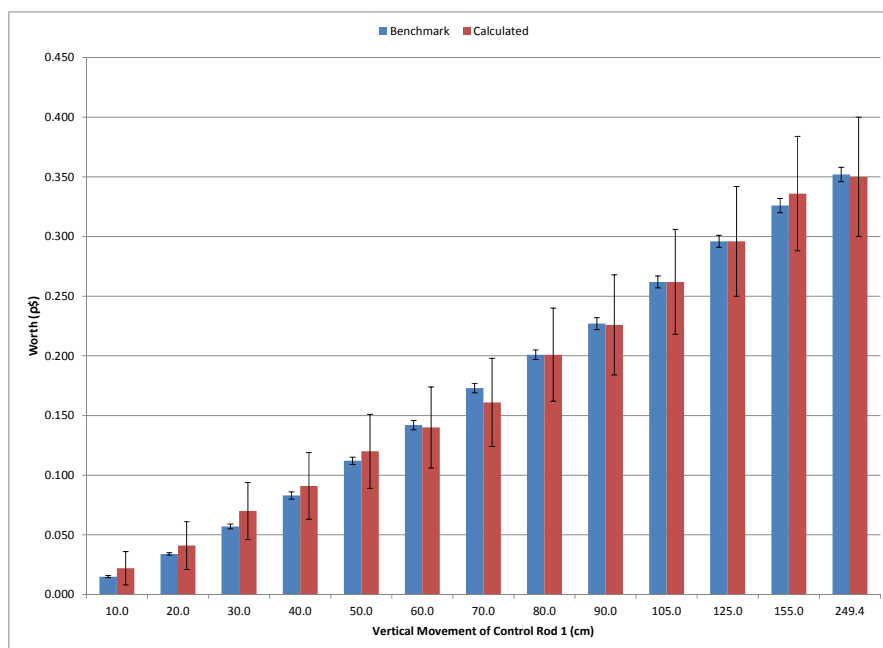
Figure 4.4-2. Control Rod 1 Cumulative Worth Results for Core 5.
