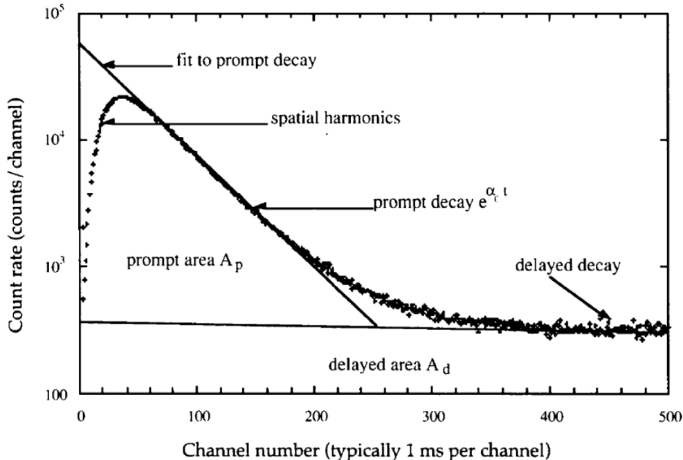
Figure 1.4-2. Example Count Rate Response for a Pulsed Neutron Source Measurement. a
