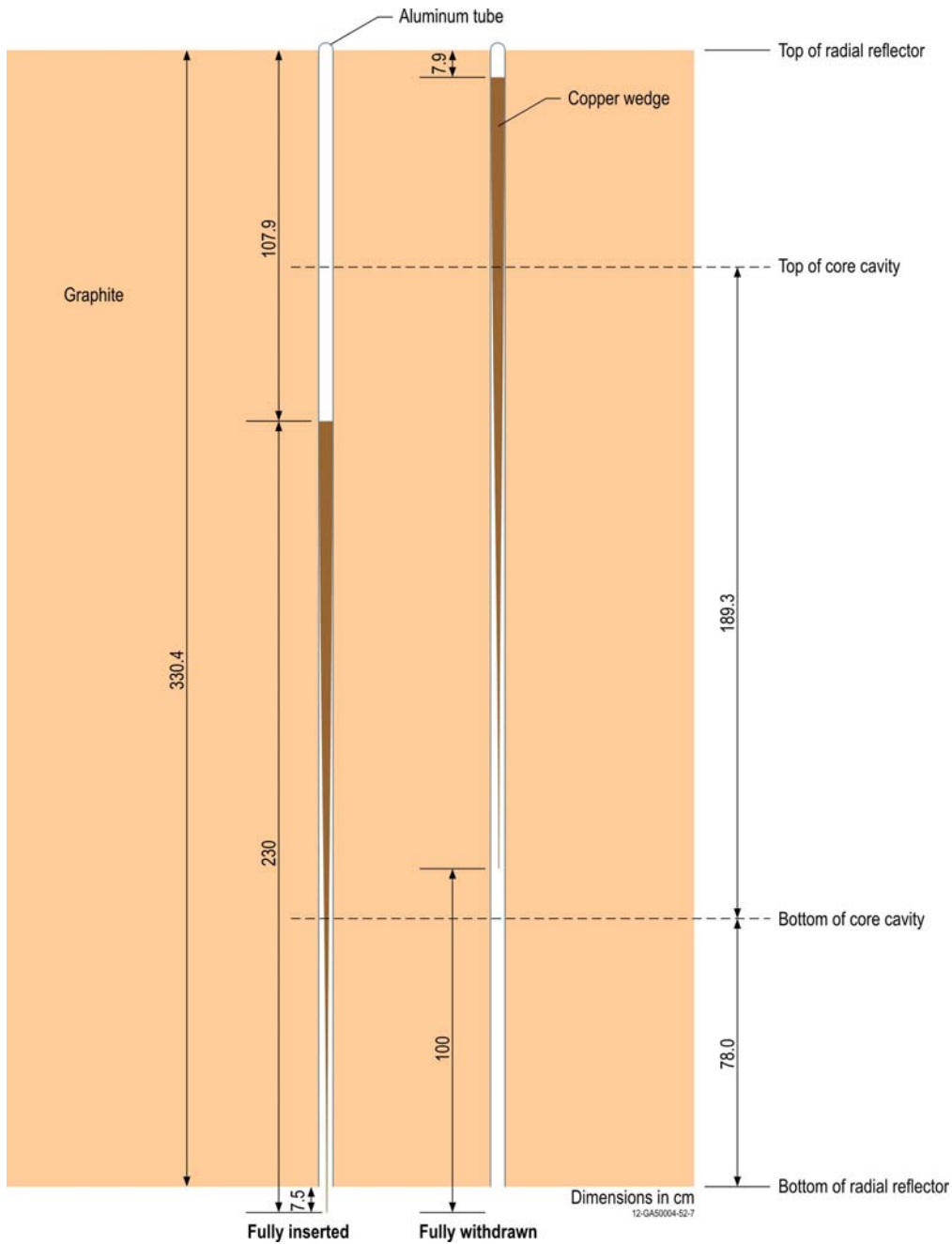
Figure 3.1-7. Autorod Vertical Position within Axial Reflector.
