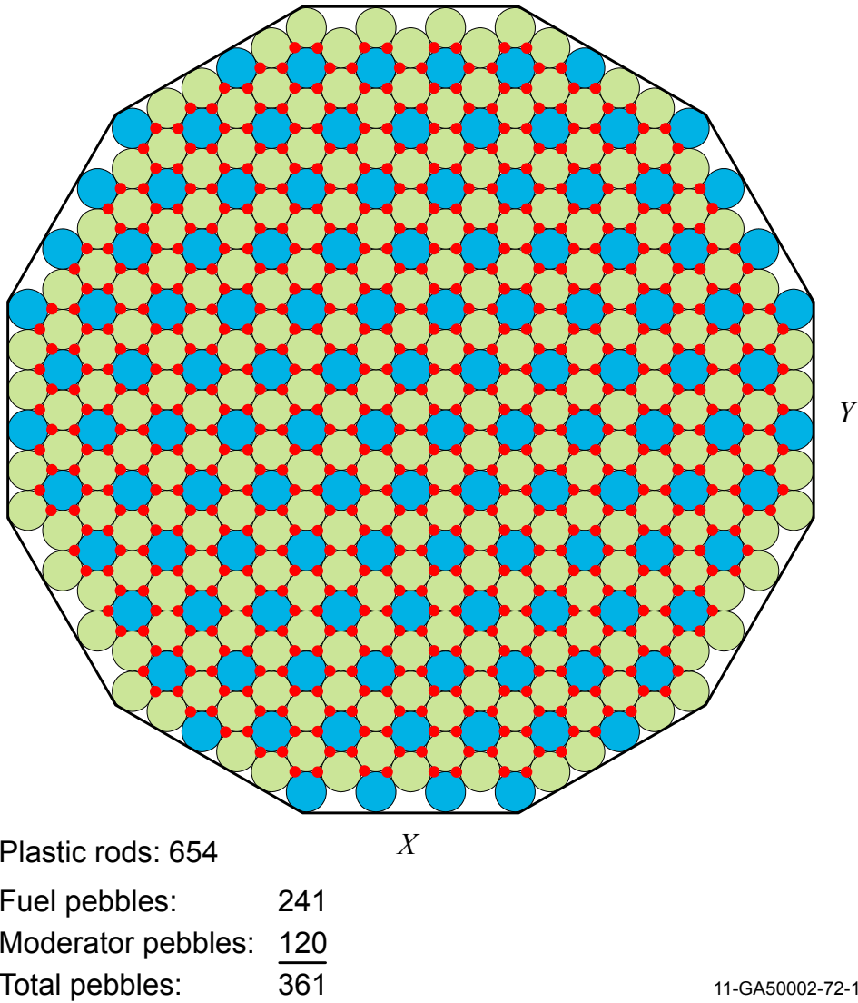
Figure 3.1-22. Layers 3, 6, 9, etc., of Cases 2 and 3 (Cores 6 and 7) and Layer 3 of Case 4 (Core 8).
