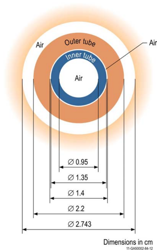
Figure 3.1-9. Top View of Withdrawable Control Rod.
