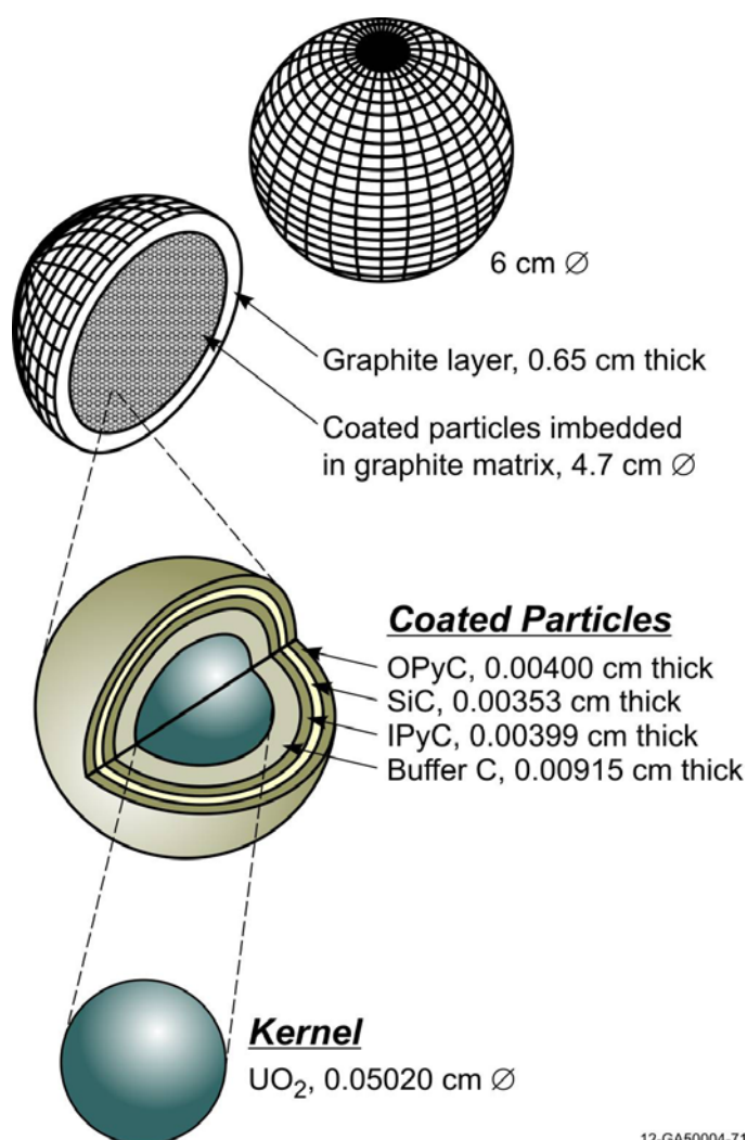
Figure 3.1-8. Fuel Pebble and TRISO Particle.
