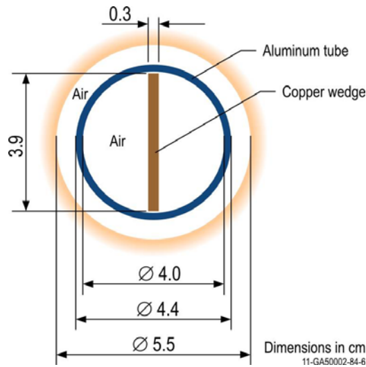
Figure 3.1-6. Top View of Autorod.
