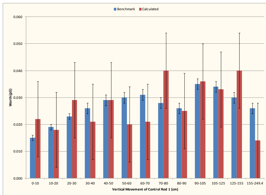
Figure 4.4-1. Control Rod 1 Differential Worth Results for Core 5.
