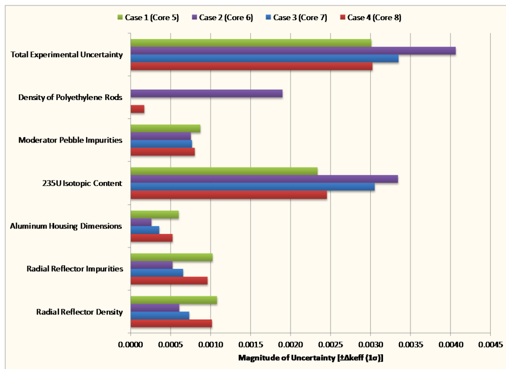
Figure 2.1-1. Graphical Representation of Primary Uncertainties in HTR-PROTEUS.
