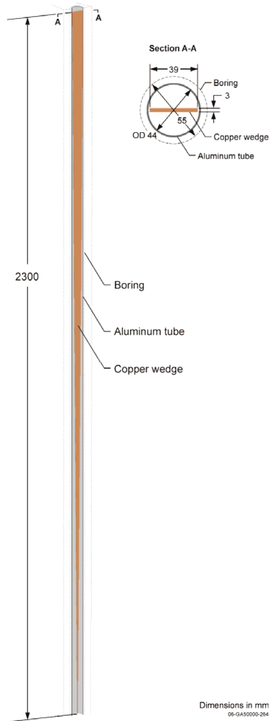
Figure 1.1-10. Automatic control rod (derived from Ref. 2).
