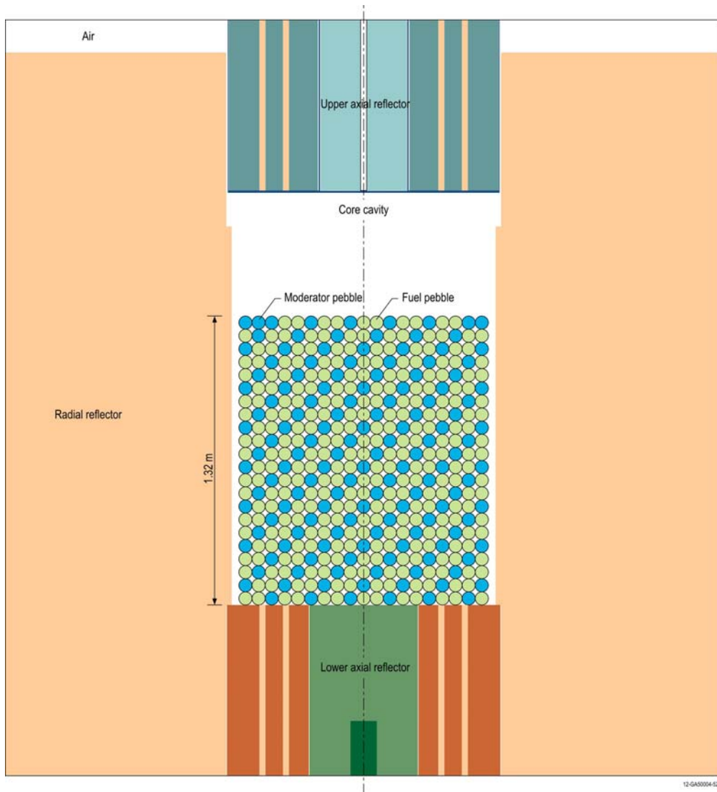
Figure 3.1-19. Vertical Profile of Case 2 (Core 6).
