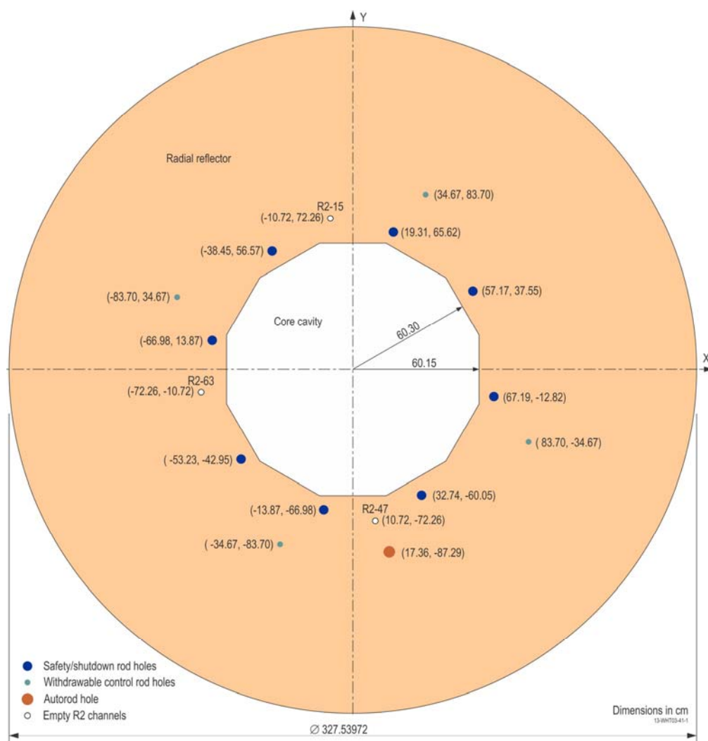
Figure 3.4-4. Radial Reflector Surrounding Core Cavity Region Including Empty R2 Channel Positions.
