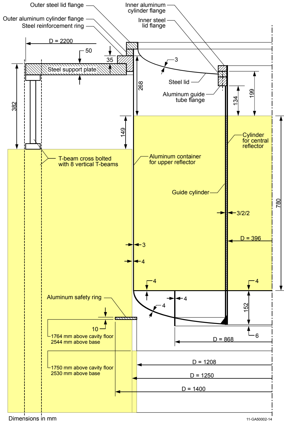
Figure 1.1-4. Placement of the upper axial reflector (Ref. 2).
