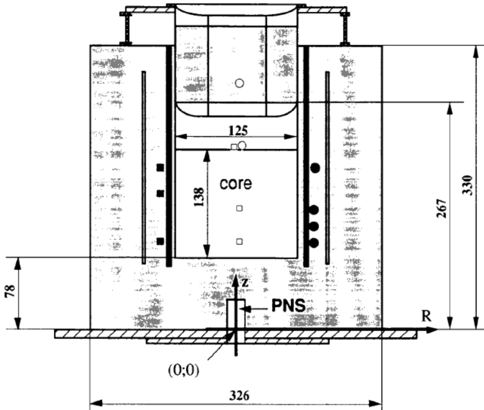
Figure 1.4-7. Schematic View Showing Positions of the Detectors and the PNS in Core 5. Circles and squares denote epithermal and thermal detector positions, respectively. Dimensions are in cm. a
