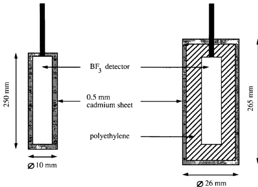
Figure 1.4-5. Schematic View of \text{BF}_3 Detectors Shielded with Cd. a
