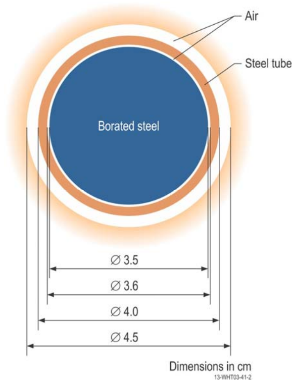
Figure 3.4-1. Top View of Safety/Shutdown Rod.
