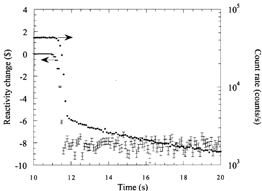
Figure 1.4-1. Example Count Rate and Reactivity Change Following Absorber Rod Insertion in Core 10. a
