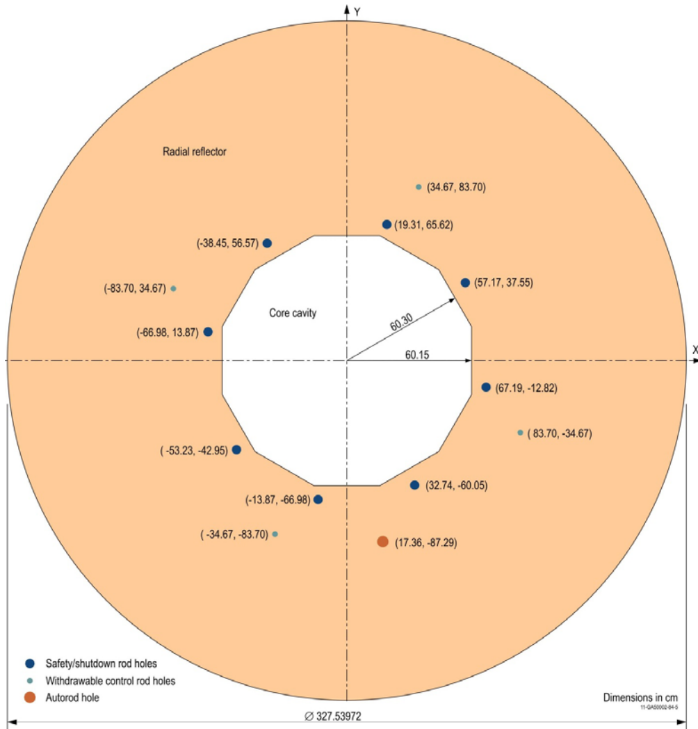
Figure 3.1-2. Radial Reflector Surrounding Core Cavity Region.
