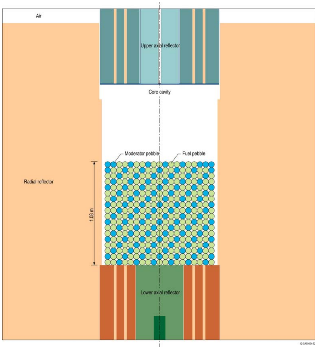
Figure 3.1-24. Vertical Profile of Case 3 (Core 7).
