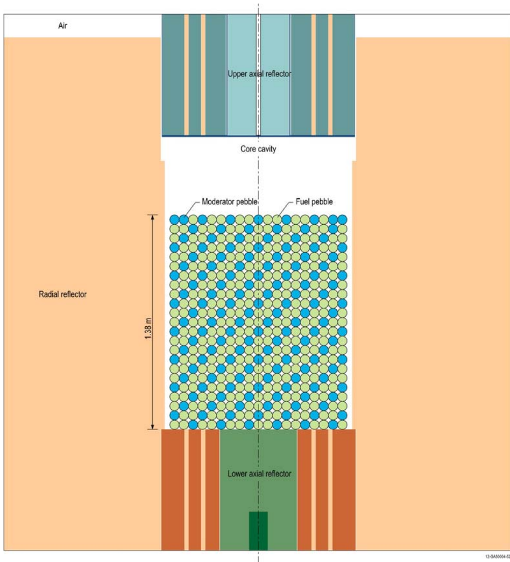
Figure 3.1-14. Vertical Profile of Cases 1 and 4 (Cores 5 and 8).
