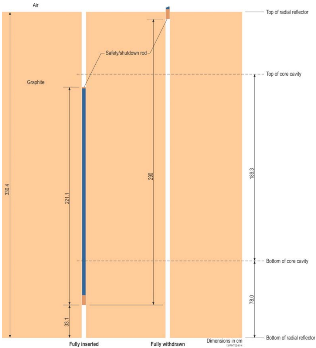
Figure 3.4-3. Safety/Shutdown Rod Vertical Position within Radial Reflector.
