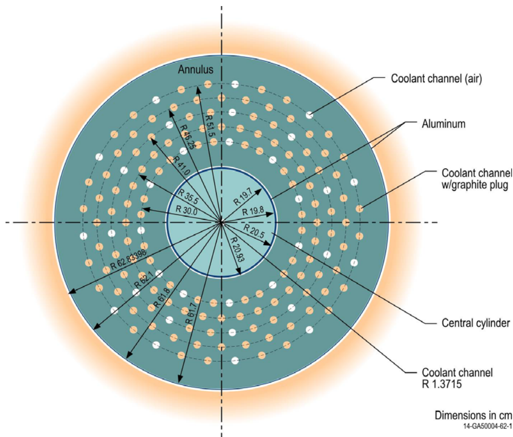
Figure 3.1-3. Upper Axial Reflector.
