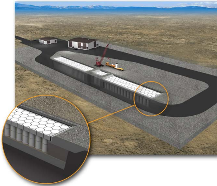
Figure 2. Example layout for the Remote-Handled Low-Level Waste Disposal Facility.
