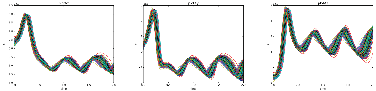
Figure 45. Time series generated by RAVEN projected in each of the three axis ( x(t) , y(t) and z(t) ).
