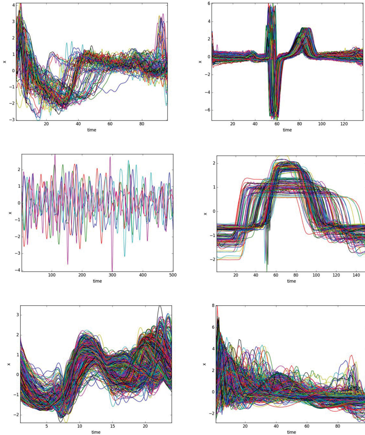
Figure 43. Plot of the ECG , ECG_5days , ford , gun_point , power_demand and medical_images data sets [32].
