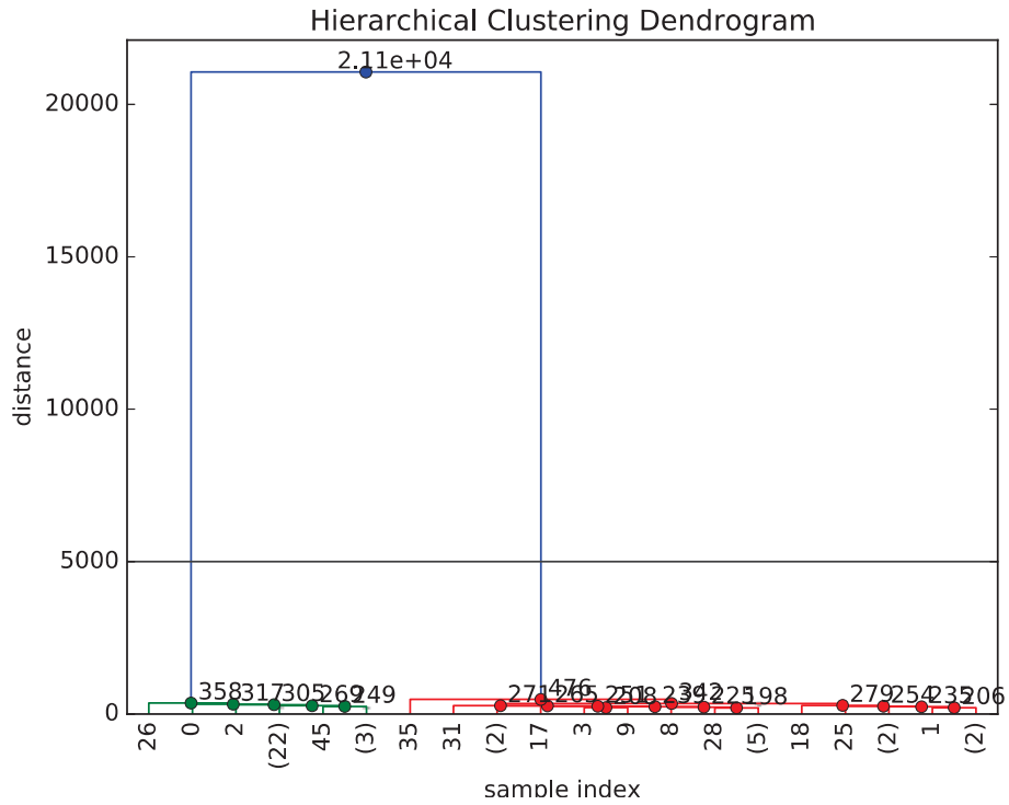
Figure 40. Dendrogram obtained from the data set shown in Figure 39.
