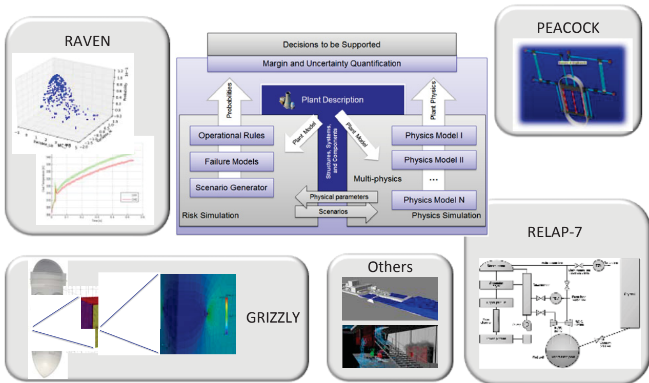
Figure 4. Overview of the RISMIC toolkit.
