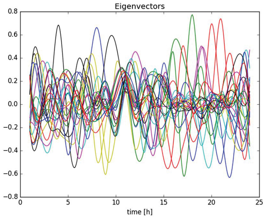
Figure 26. Plot of the eigenvectors of the data set shown in Figure 25.
