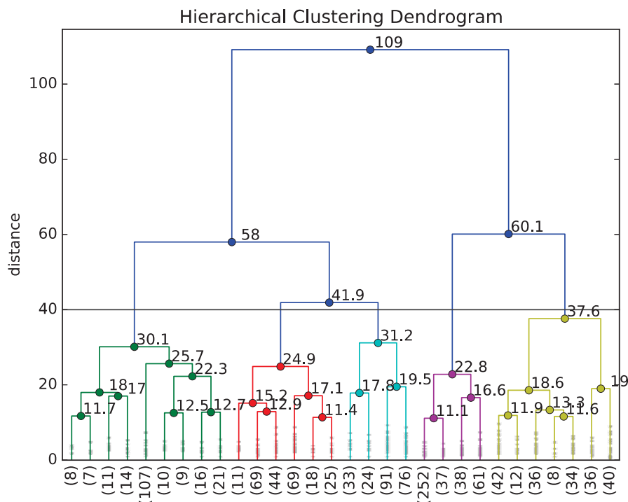
Figure 69. Dendrogram obtained using hierarchical clustering (euclidean distance) for the Cluster 1 dataset shown in Figure 66.
