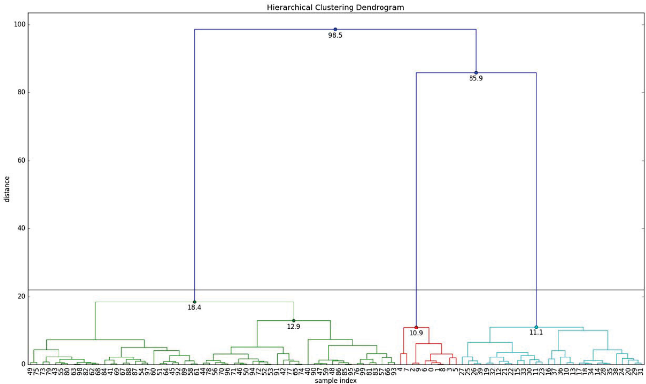
Figure 9. Dendrogram obtained by RAVEN for the data set shown in Figure 8.
