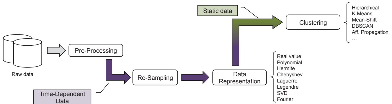
Figure 16. Analysis of time-dependent data using static representation conversion.
