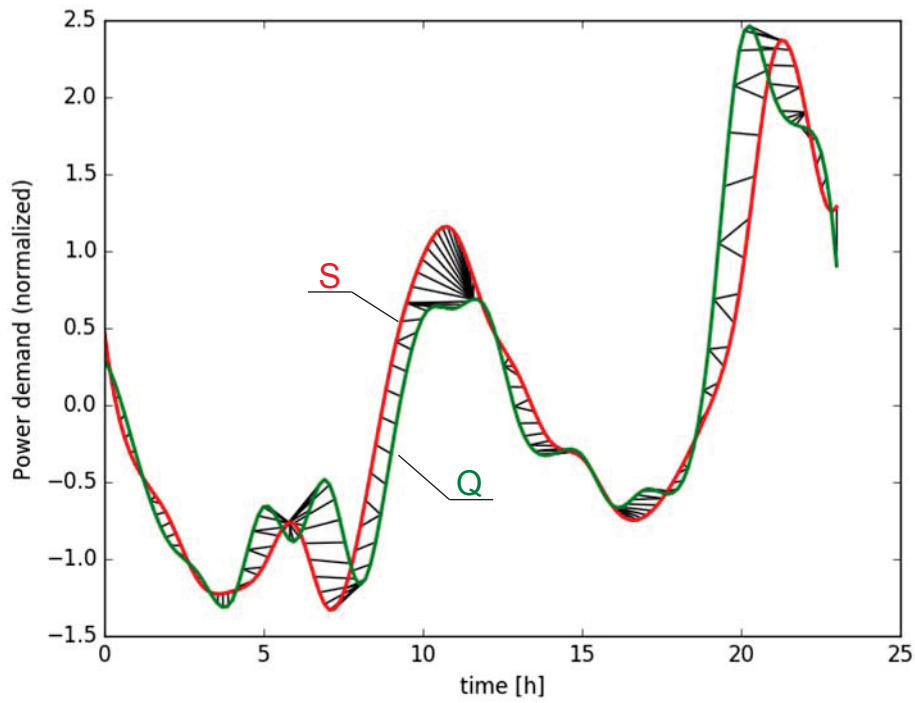
Figure 34. DTW distance metric for two time series S and Q . Each black segment represents an element w_k = (d_{i,j})_k of the warp path shown in Figure 33.
