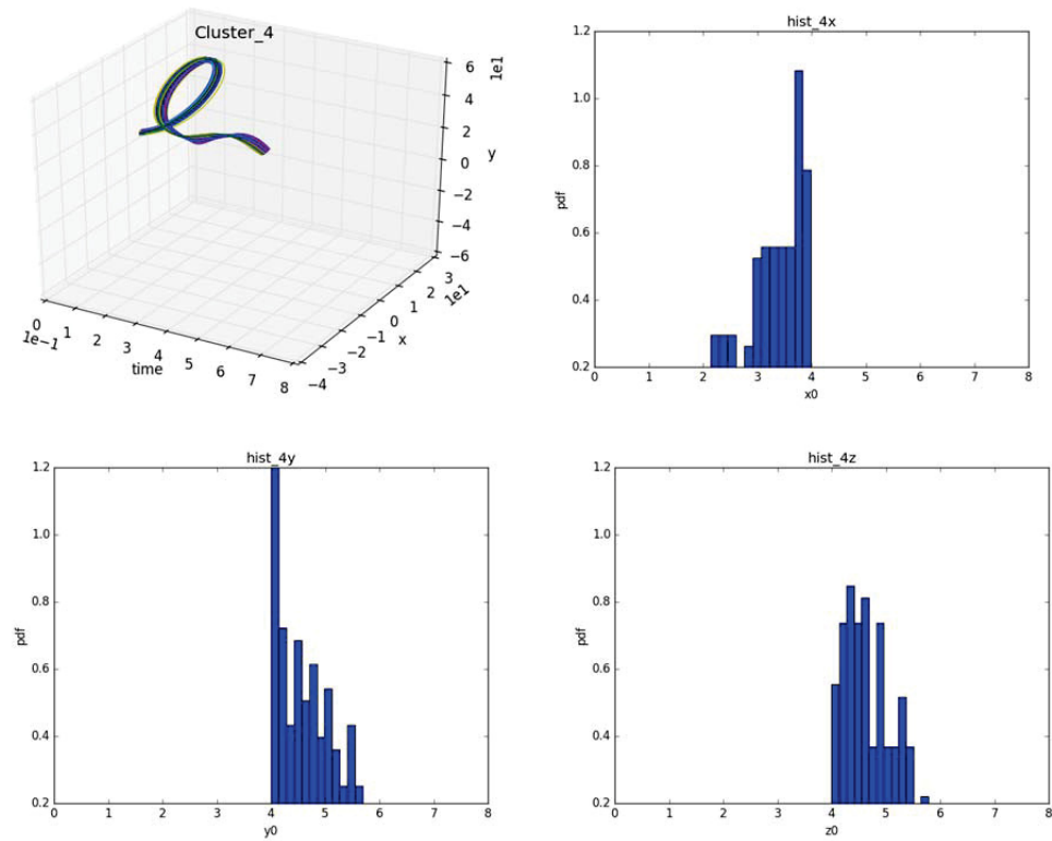
Figure 54. Analytical model analysis - Cluster 4 information: time series and histograms for the sampled values ( x(0) , y(0) and z(0) ).
