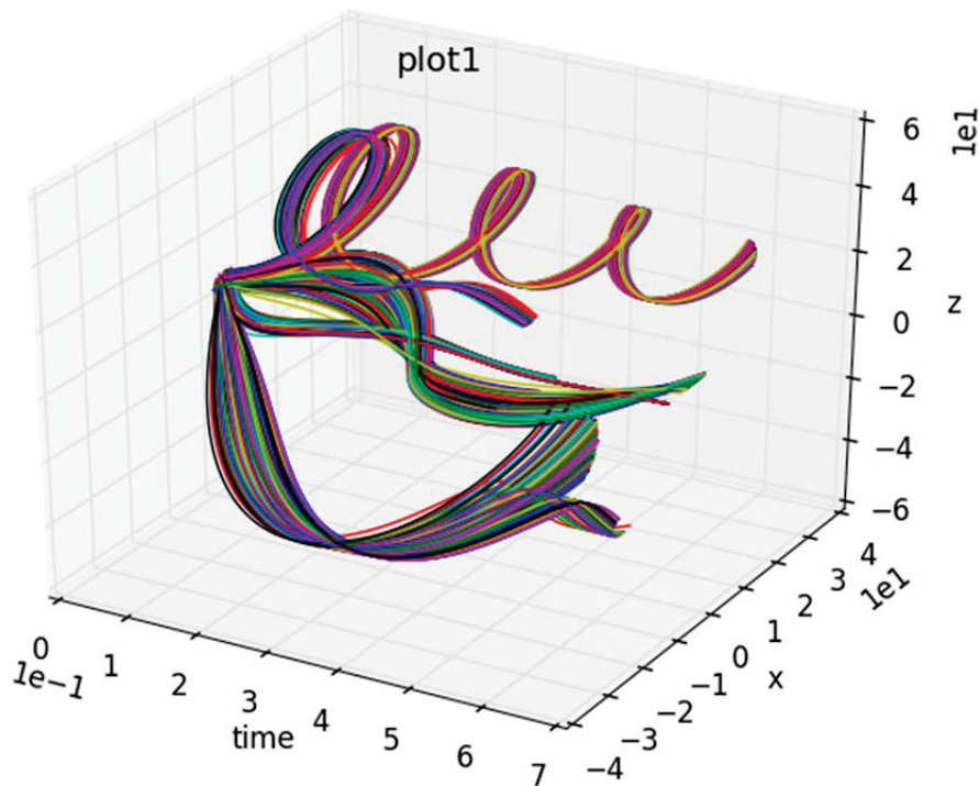
Figure 46. Data set generated by RAVEN containing multiple discountuities and having variable time length.
