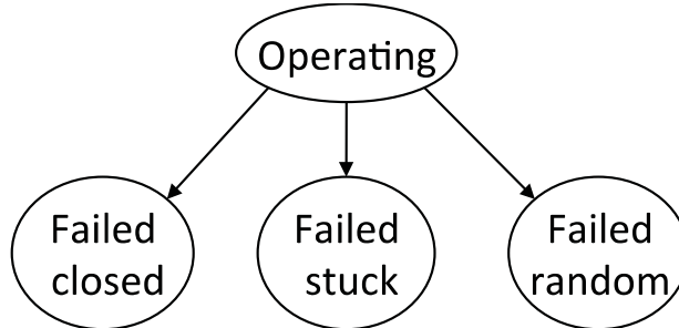
Figure 59. Continuous time Markov model for the pump controller.
