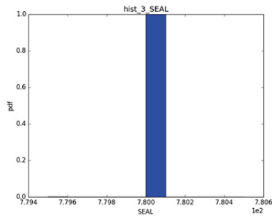
Figure 83. PWR Station Black-Out: analysis of Cluster 3.
