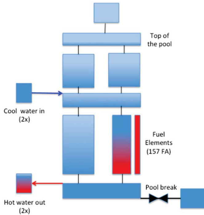
Figure 88. RELAP5-3D SFP model.
