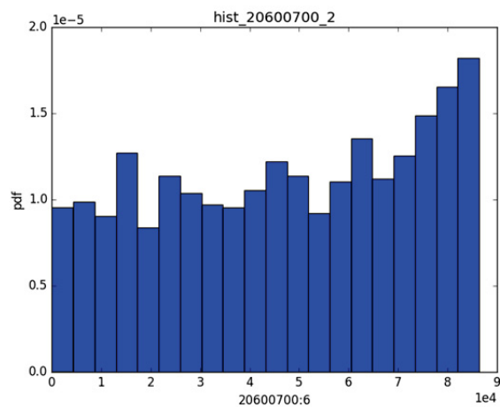
Figure 97. SFP test case: Cluster 2 data analysis. Plot of the time histories contained in this cluster and histograms of the sampled variables.
