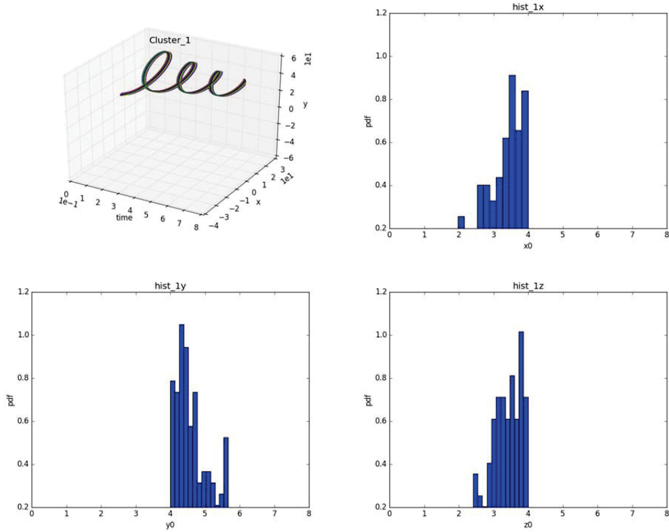
Figure 51. Analytical model analysis - Cluster 1 information: time series and histograms for the sampled values ( x(0) , y(0) and z(0) ).
