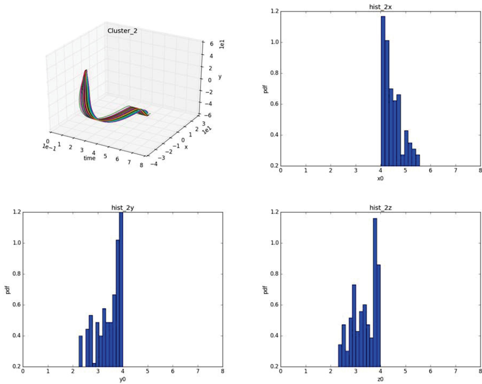
Figure 52. Analytical model analysis - Cluster 2 information: time series and histograms for the sampled values ( x(0) , y(0) and z(0) ).
