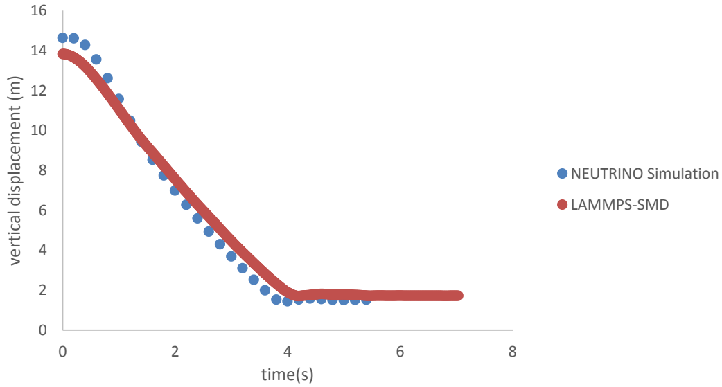
Figure 19. Comparison of vertical displacement of falling block simulated by LAMMPS and NEUTRINO.
