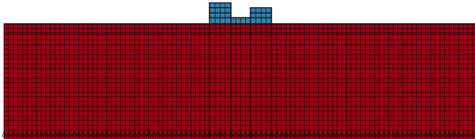
Figure 6. Node set for ground motion input.
