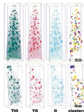
Figure 1. LEAP images showing elemental distribution maps at near-atomic level for the as-received (top row) and neutron irradiated (bottom row) ODS steels.
