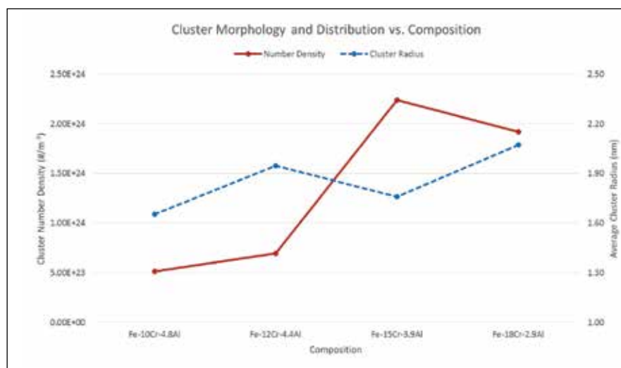
Figure 3. Trends in calculated cluster number density and average spherical equivalent cluster radius for \alpha' precipitates in 7 dpa Fe-Cr-Al for the four model alloy compositions.
