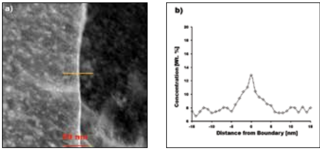
Figure 4. Segregation profile of Cr across a high angle grain boundary ( \theta=49^{\circ}\text{C} ) of the neutron irradiated specimen. (a) STEM image, (b) segregation profile obtained from EDS analysis.
