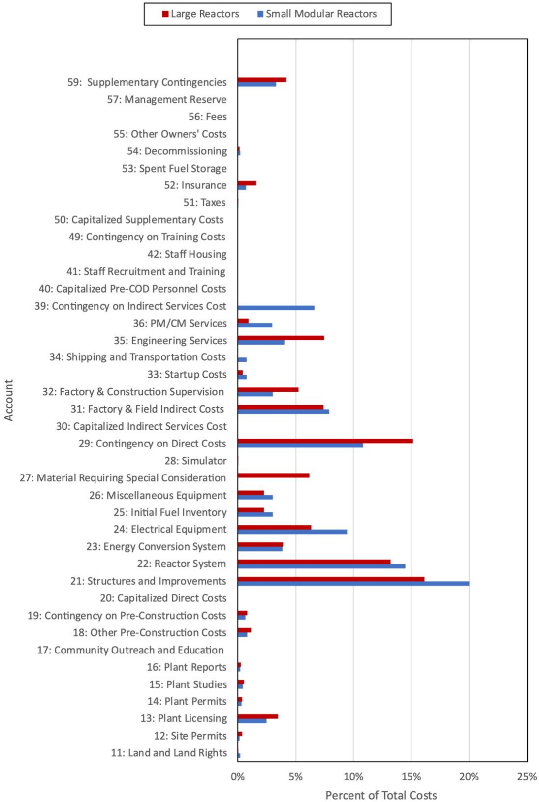
Figure 23. Comparison of Level 2 costs between the large and small modular reactors.
