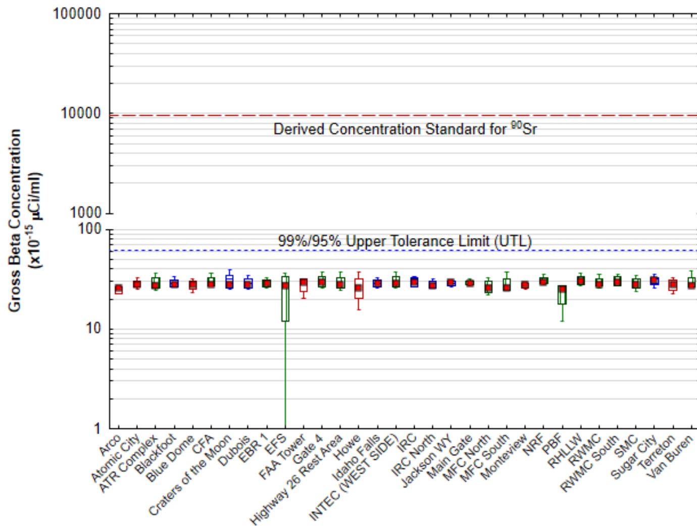
Figure 8. July 2023 gross beta concentrations in air at onsite, boundary, and offsite locations. The DCS is the concentration of ^{90}\text{Sr} in air which, if inhaled for a year, would result in a dose of 100 mrem/yr. Because the measurements include naturally-occurring radionuclides (such as ^{40}\text{K} , ^{228}\text{Ra} , and ^{210}\text{Pb} ) in uncertain proportions, a meaningful DCS cannot be constructed for gross beta concentrations. The DCS for ^{90}\text{Sr} is shown because it is the most restrictive human-made beta emitter. The UTL represents the value below which 99% of the population values are expected to fall with 95% confidence.
