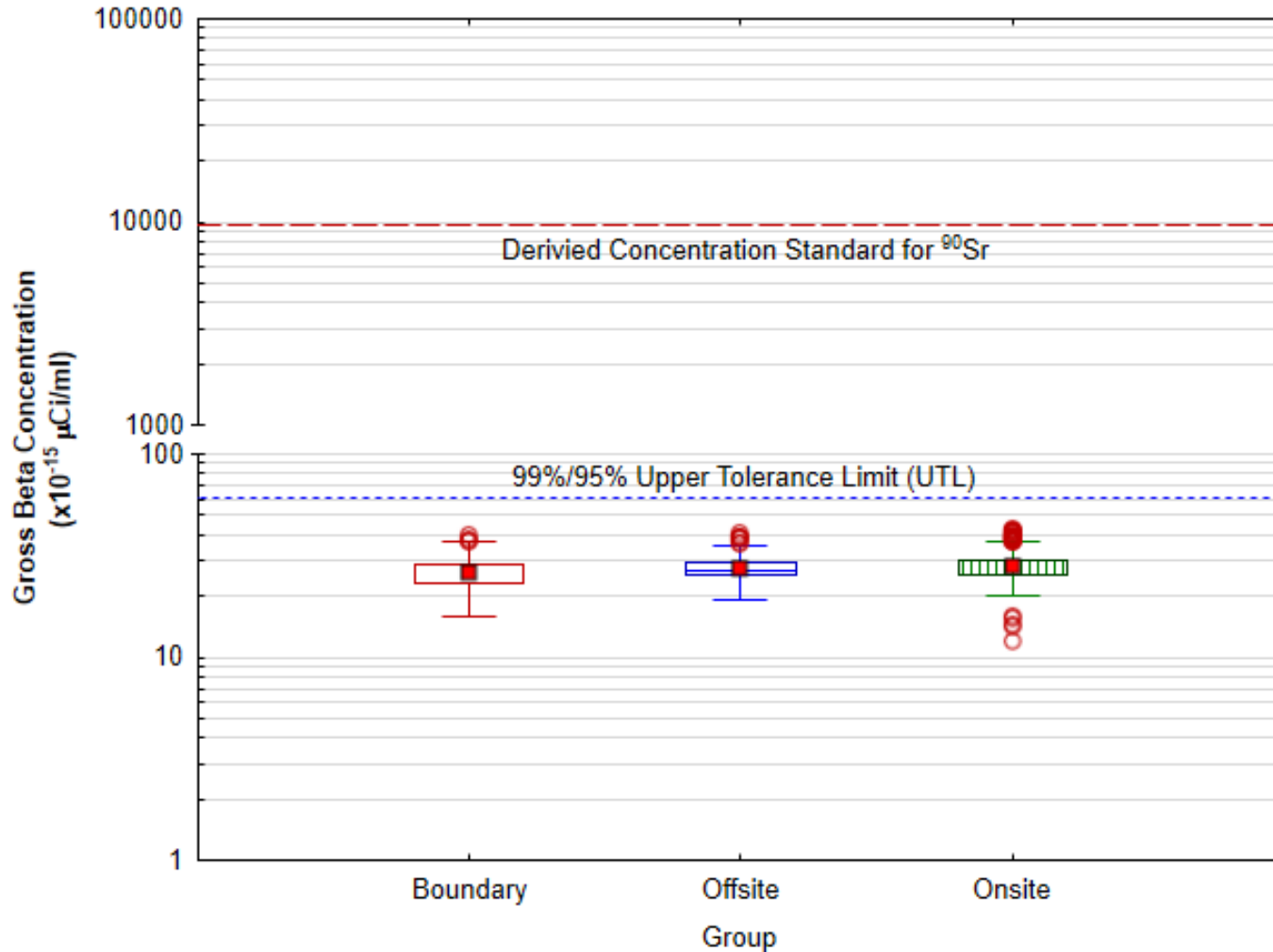
Figure 7. Gross beta concentrations in air at onsite, boundary, and offsite locations for the third quarter of 2023. The DCS is the concentration of ^{90}\text{Sr} in air which, if inhaled for a year, would result in a dose of 100 mrem/yr. Because the measurements include naturally-occurring radionuclides (such as ^{40}\text{K} , ^{228}\text{Ra} , and ^{210}\text{Pb} ) in uncertain proportions, a meaningful DCS cannot be constructed for gross beta concentration. The DCS for ^{90}\text{Sr} is shown because it is the most restrictive human-made beta emitter. The UTL represents the value below which 99% of the population values are expected to fall with 95% confidence.
