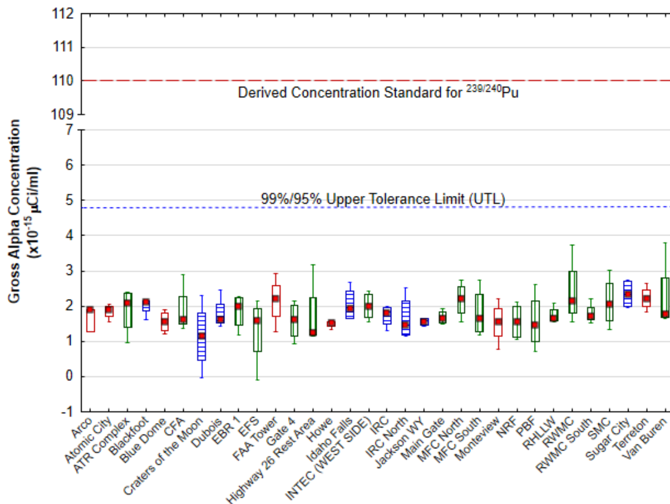
Figure 4. July 2023 gross alpha concentrations in air at onsite, boundary, and offsite locations. The DCS is the concentration of ^{239/240}\text{Pu} in air which, if inhaled for a year, would result in a dose of 100 mrem/yr. Because the measurements include naturally-occurring radionuclides (such as ^{238}\text{U} , ^{234}\text{U} , ^{232}\text{Th} , ^{226}\text{Ra} , and ^{210}\text{Po} ) in uncertain proportions, a meaningful DCS cannot be constructed for gross alpha concentrations. The DCS for ^{239/240}\text{Pu} is shown because it is the most restrictive human-made alpha emitter. The UTL represents the value below which 99% of the population values are expected to fall with 95% confidence.
