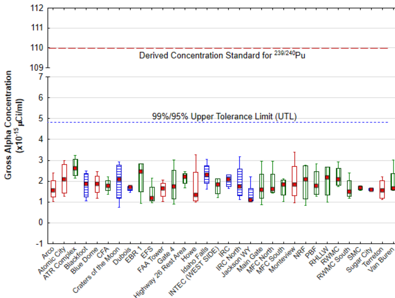
Figure 6. September 2023 gross alpha concentrations in air at onsite, boundary, and offsite locations. The DCS is the concentration of 239/240 Pu in air which, if inhaled for a year, would result in a dose of 100 mrem/yr. Because the measurements include naturally-occurring radionuclides (such as 238 U, 234 U, 232 Th, 226 Ra, and 210 Po) in uncertain proportions, a meaningful DCS cannot be constructed for gross alpha concentrations. The DCS for 239/240 Pu is shown because it is the most restrictive human-made alpha emitter. The UTL represents the value below which 99% of the population values are expected to fall with 95% confidence.
