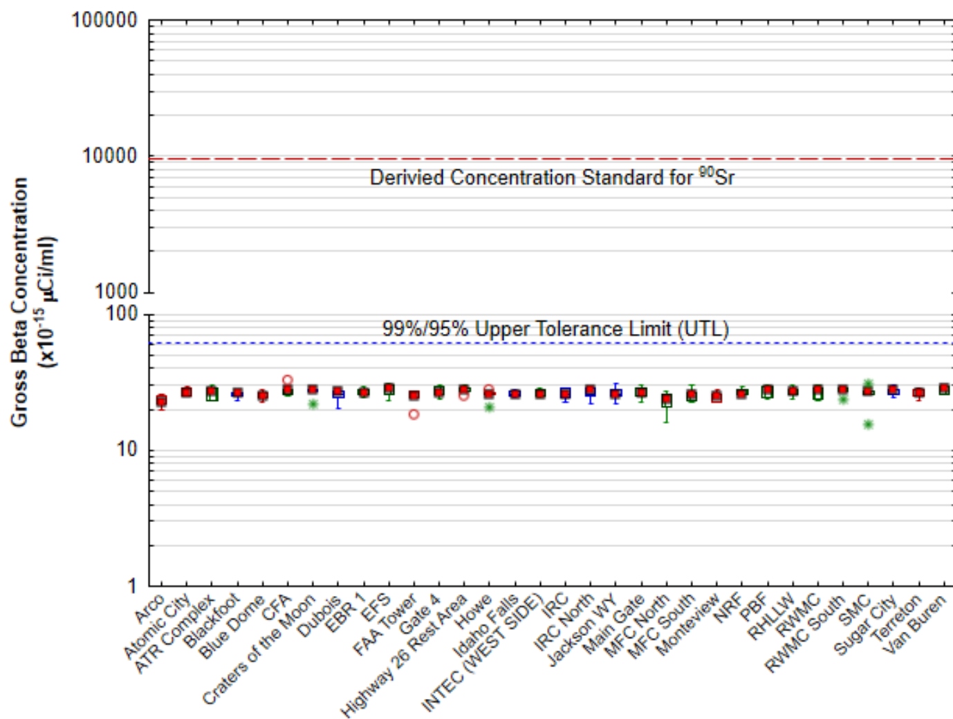
Figure 9. August 2023 gross beta concentrations in air at onsite, boundary, and offsite locations. The DCS is the concentration of ^{90}\text{Sr} in air which, if inhaled for a year, would result in a dose of 100 mrem/yr. Because the measurements include naturally-occurring radionuclides (such as ^{40}\text{K} , ^{228}\text{Ra} , and ^{210}\text{Pb} ) in uncertain proportions, a meaningful DCS cannot be constructed for gross beta concentrations. The DCS for ^{90}\text{Sr} is shown because it is the most restrictive human-made beta emitter. The UTL represents the value below which 99% of the population values are expected to fall with 95% confidence.
