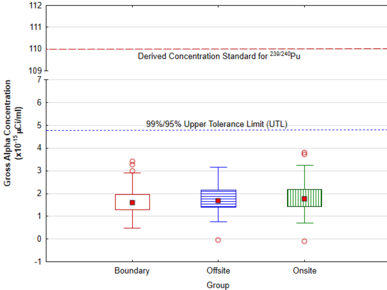
Figure 3. Gross alpha concentrations in air at onsite, boundary, and offsite locations for the third quarter of 2023. The DCS is the concentration of ^{239/240}\text{Pu} in air which, if inhaled for a year, would result in a dose of 100 mrem/yr. Because the measurements include naturally-occurring radionuclides (such as ^{238}\text{U} , ^{234}\text{U} , ^{232}\text{Th} , ^{226}\text{Ra} , and ^{210}\text{Po} ) in uncertain proportions, a meaningful DCS cannot be constructed for gross alpha concentrations. The DCS for ^{239/240}\text{Pu} is shown because it is the most restrictive human-made alpha emitter. The UTL represents the value below which 99% of the population values are expected to fall with 95% confidence.
