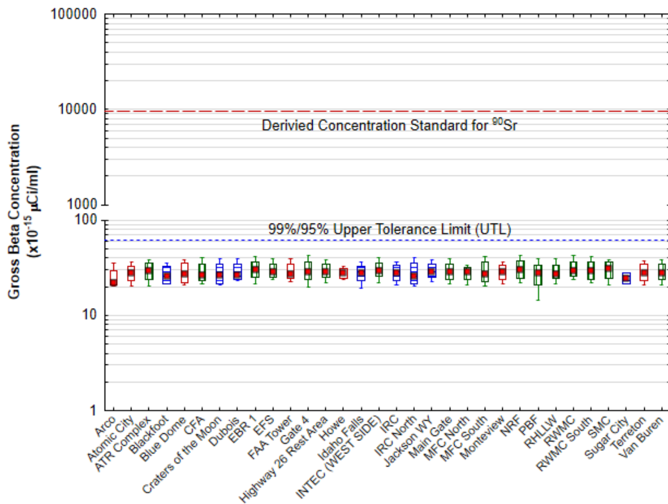
Figure 10. September 2023 gross beta concentrations in air at onsite, boundary, and offsite locations. The DCS is the concentration of 90 Sr in air which, if inhaled for a year, would result in a dose of 100 mrem/yr. Because the measurements include naturally-occurring radionuclides (such as 40 K, 228 Ra, and 210 Pb) in uncertain proportions, a meaningful DCS cannot be constructed for gross beta concentrations. The DCS for 90 Sr is shown because it is the most restrictive human-made beta emitter. The UTL represents the value below which 99% of the population are expected to fall with 95% confidence.
