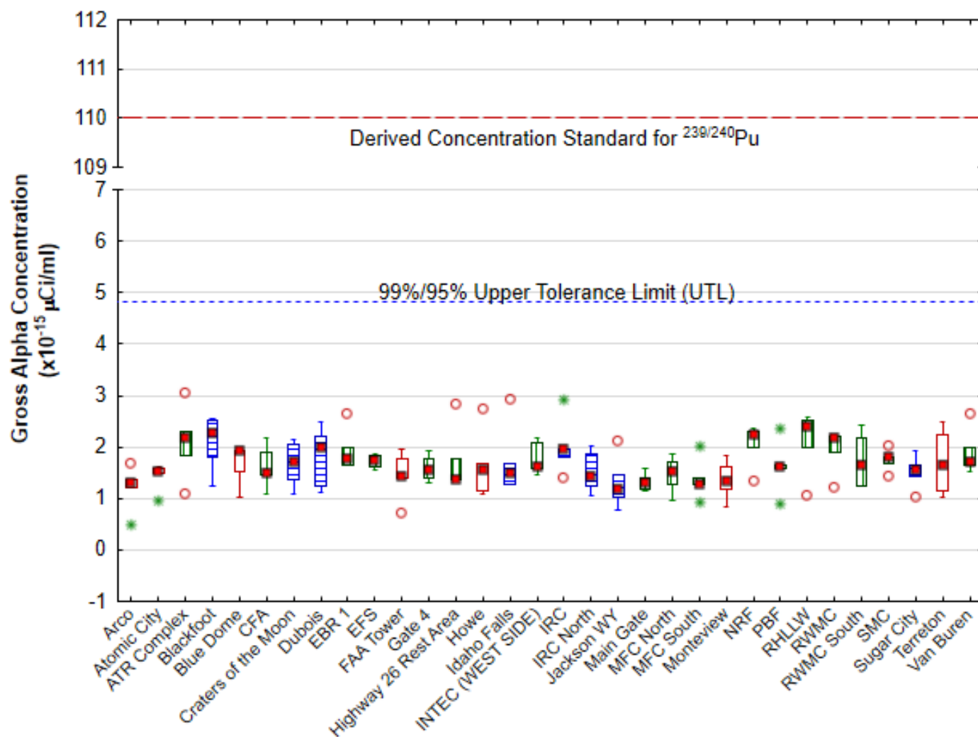
Figure 5. August 2023 gross alpha concentrations in air at onsite, boundary, and offsite locations. The DCS is the concentration of 239/240 Pu in air which, if inhaled for a year, would result in a dose of 100 mrem/yr. Because the measurements include naturally-occurring radionuclides (such as 238 U, 234 U, 232 Th, 226 Ra, and 210 Po) in uncertain proportions, a meaningful DCS cannot be constructed for gross alpha concentrations. The DCS for 239/240 Pu is shown because it is the most restrictive human-made alpha emitter. The UTL represents the value below which 99% of the population values are expected to fall with 95% confidence.
