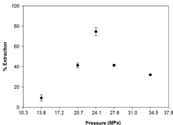
Figure 7. The percent extraction of Eu from 1000 mg/kg Eu 8 M HCl solution with TBDGA in CO 2(l) modified with 2 mol% 1-octanol as a function of pressure (13.8–34.5 MPa) at 23 °C.
