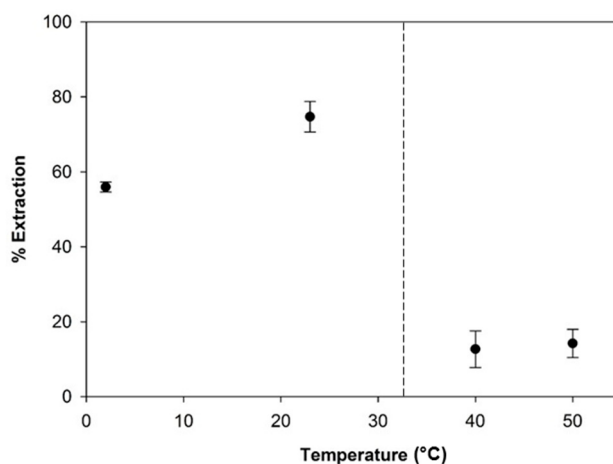
Figure 6. The percent extraction of Eu from a 1000 mg/kg in 8 M HCl solution with TBDGA in \text{CO}_2 modified with 2 mol% 1-octanol as the temperature is varied from 2 °C–50 °C at 34.5 MPa. At temperatures less than 31 °C \text{CO}_2 is a liquid, and above 31 °C the \text{CO}_2 is in the supercritical phase. This point is shown with a dotted line.
