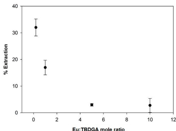
Figure 8. The percent extraction Eu from 8 M HCl with TBDGA in \text{CO}_{2(l)} modified with 2 mol% 1-octanol at 34.5 MPa and 23 °C where the starting Eu concentration in the HCl phase is varied from 1000 to 50,000 mg/kg.
