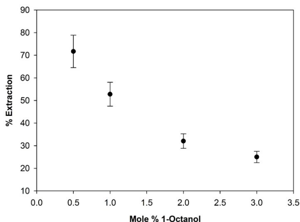
Figure 5. The percent extraction of Eu from 10 mL 1000 mg/kg Eu in 8 M HCl with TBDGA in 1-octanol at 23 °C and 34.5 MPa in \text{CO}_{2(l)} . The mol% of 1-octanol was varied by the flow rate as listed in Table 1.
