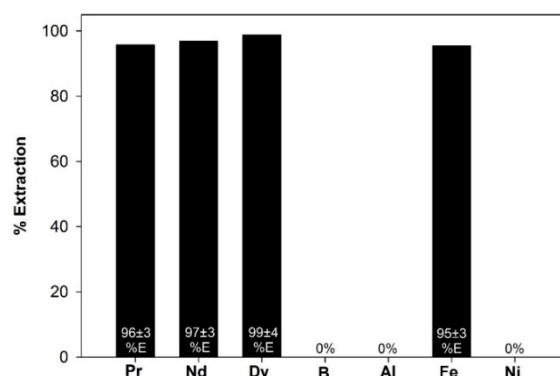
Figure 13. Extraction from neodymium iron boron magnet materials with 0.5 mol% 1-octanol in \text{CO}_{2(l)} , 0.072 M TBDGA in 1-octanol TBDGA:M by mole, 23 °C, 24.1 MPa, and a flow rate of 5.0 \pm 0.5 mL/min.
