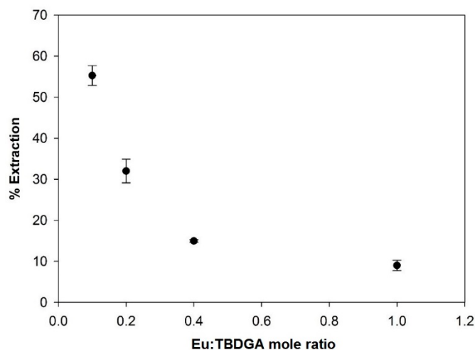
Figure 9. The percent extraction of Eu from a 1000 mg/kg 8 M HCl solution with varied TBDGA concentration in \text{CO}_{2(l)} modified with 2 mol% 1-octanol at 34.5 MPa and 23 °C. The TBDGA concentration is listed in Table 3.
