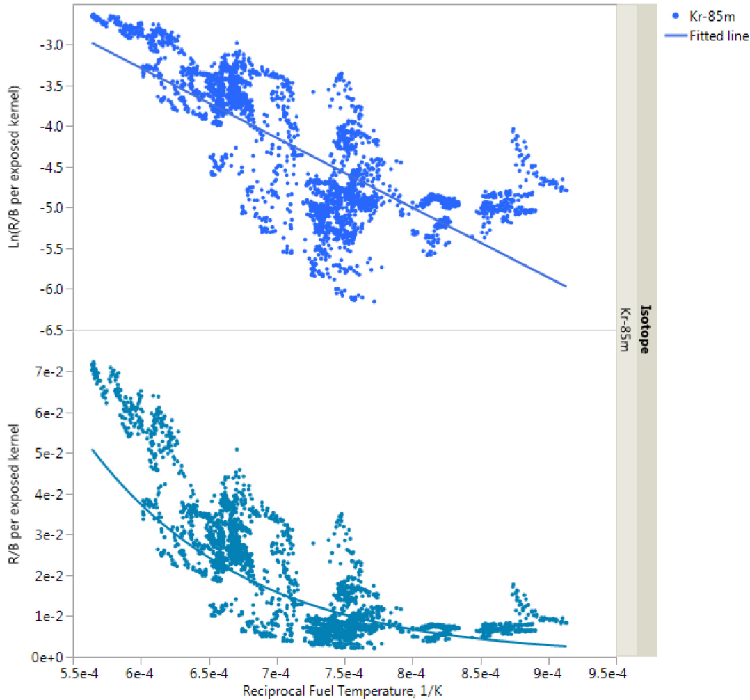
Figure 25. Kr-85m R/B per exposed kernel and the fitted line in natural logarithm scale (top panel) and in linear scale (bottom panel).
