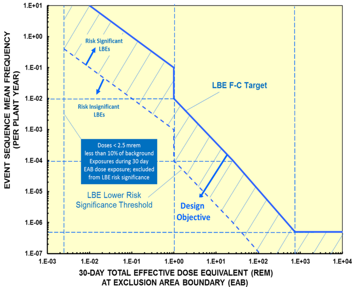
Figure 2-6. Use of F-C Target to Define Risk-Significant LBEs
