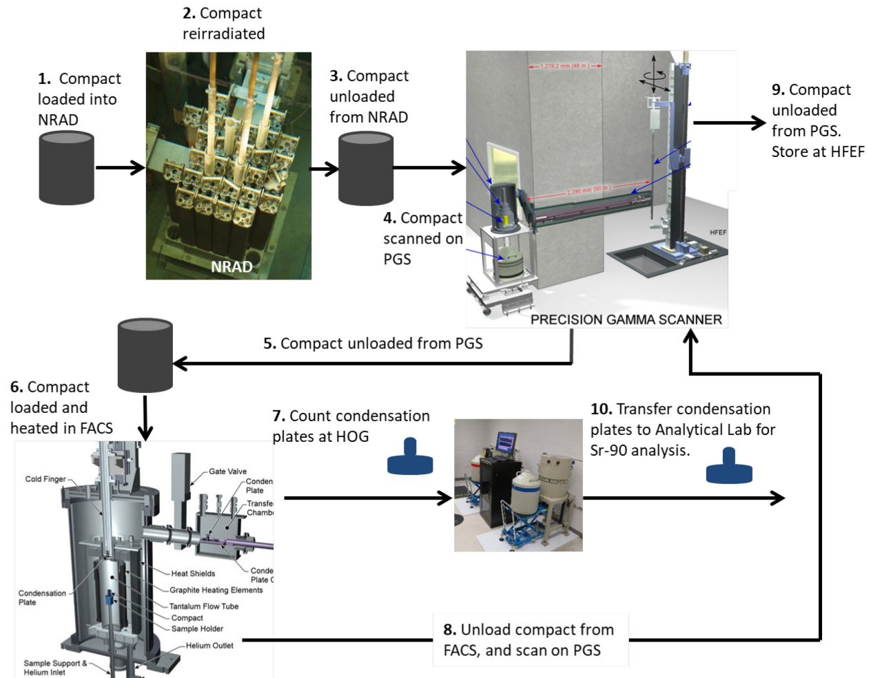
Figure 2. Flow chart of compact reirradiation, heating test and gamma scanning/counting activities.
