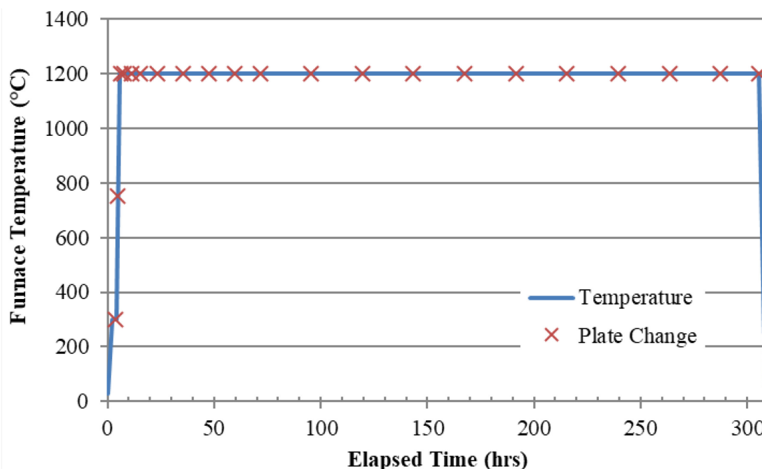
Figure 3. Temperature profile for the test, including time and temperatures of plate changes. See Table 4 for complete list of plate exchanges and timings of exchanges.
