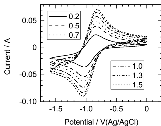
Figure 2. Cyclic voltammograms for (a) 1 wt%, (b) 2 wt% and (c) 3 wt% \text{SmCl}_3 in LiCl-KCl eutectic at 500 °C with scan rate in \text{V s}^{-1} as a parameter.
