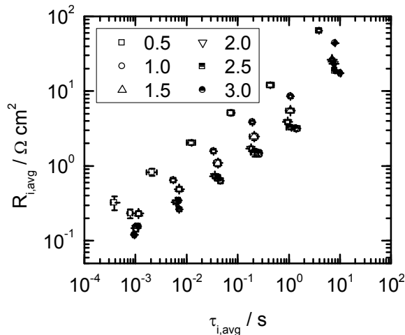
Figure 16. The R_{i,avg} value as a function of the \tau_{i,avg} value at the bias potential of -0.930 V with the concentration of SmCl_3 in wt% as a parameter.
