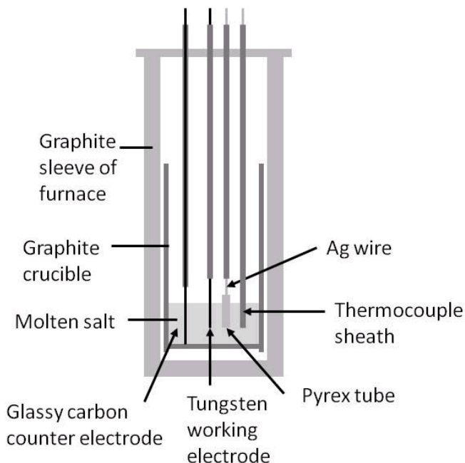
Figure 1. Schematic of the experimental setup of the three-probe electrode in the molten salt contained in the graphite crucible and placed within the sleeve of the furnace.
