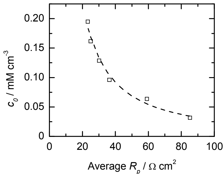
Figure 18. Experimental bulk concentration value as a function of calculated average polarization resistance. The dashed line is the fit of equation to the data.
