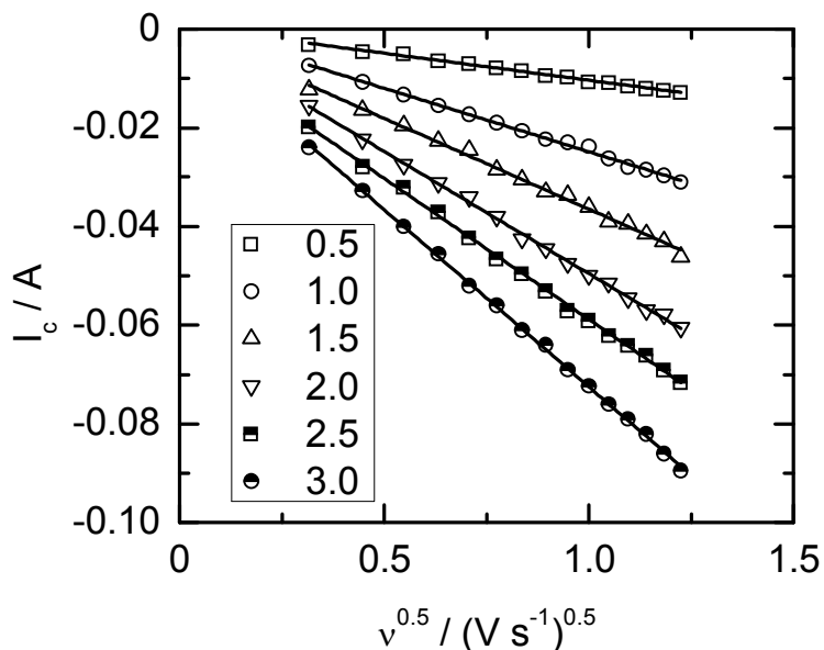
Figure 7. Plot of cathodic peak current as a function of the square root of scan rate with the concentration of \text{SmCl}_3 in wt% as a parameter.
