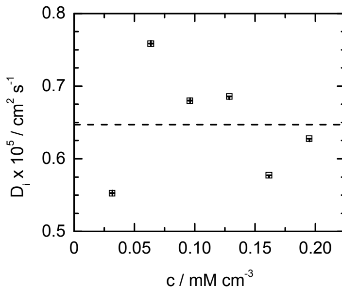
Figure 8. The diffusion coefficient of Sm 3+ as a function of the concentration of SmCl 3 in LiCl-KCl at 500 °C. The horizontal dashed line represents the average value.
