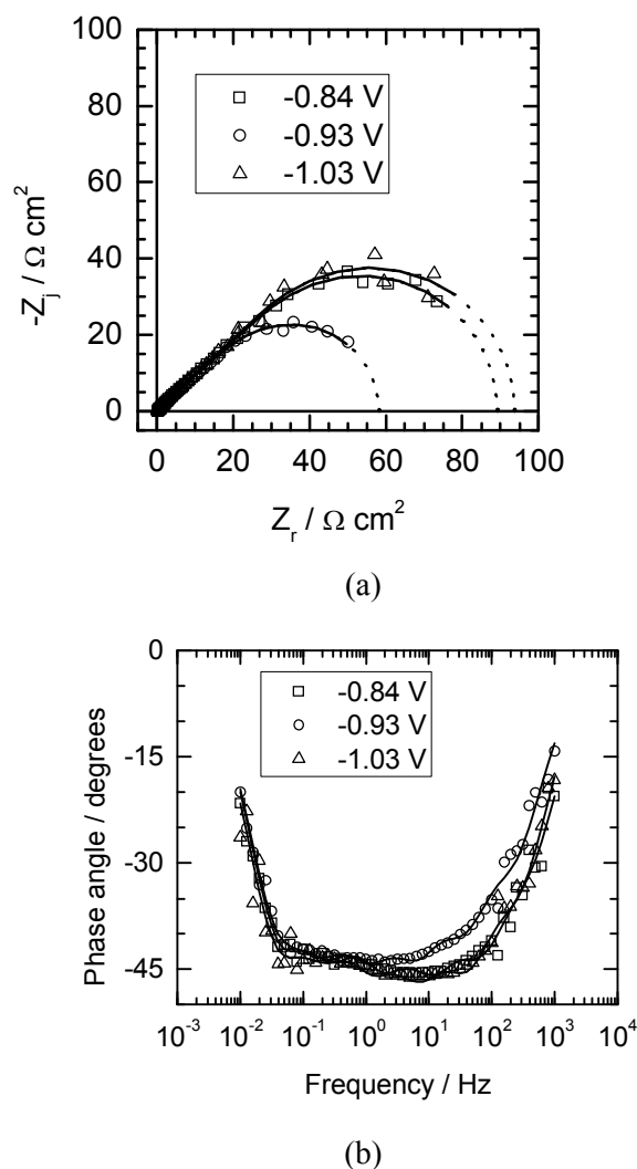
Figure 11. (a) Nyquist and (b) Bode phase angle plots of EIS data for the 1.0 wt% \text{SmCl}_3 system with bias potential as a parameter. The solid lines in (a) and (b) that overlay the data represent the fit of the six-element Voigt model to the EIS data and the dotted lines in (a) represent the extrapolation of the given fit to a 0.00001 Hz frequency where the Z_r value is the polarization resistance.
