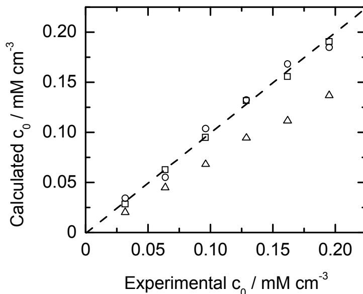
Figure 9. Calculated bulk concentration values as a function of experimental bulk concentration when using the average (square) and literature (triangle) diffusion coefficients for \text{Sm}^{3+} and the polarization resistance-concentration relationship (circle).
