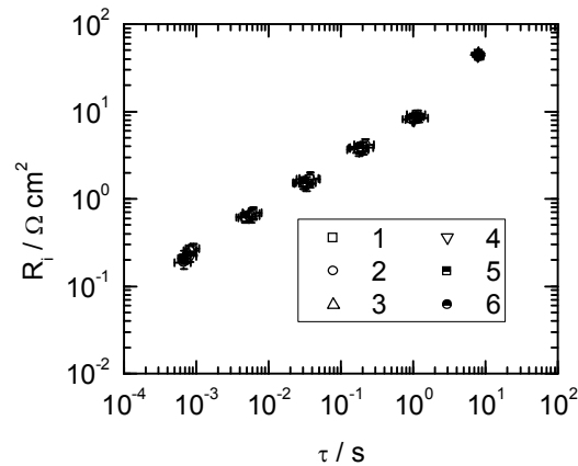
Figure 12. The R_i value as a function of the \tau_i value with the EIS spectrum as a parameter for the 1.0 wt% \text{SmCl}_3 system. These values were obtained by fitting the EIS spectra to the six-element Voigt equivalent circuit.
