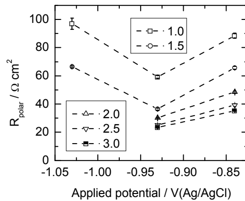
Figure 14. The average polarization resistance value as a function of bias potential with the \text{SmCl}_3 concentration in wt% as a parameter.
