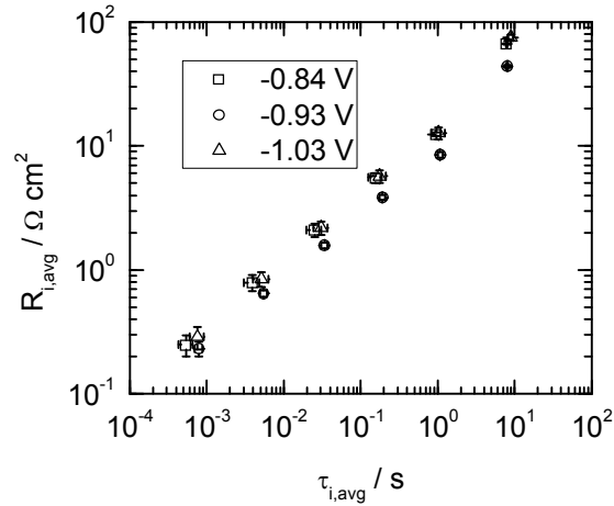
Figure 13. The R_{i,avg} value as a function of the \tau_{i,avg} value with the applied bias potential as a parameter for
