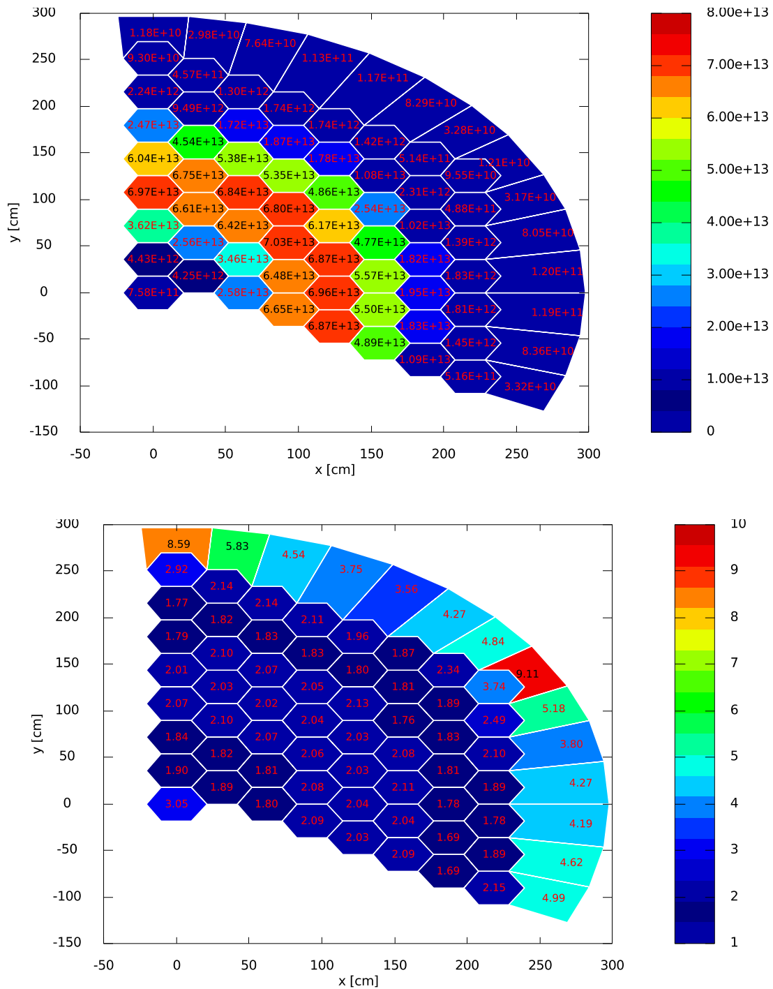
Figure B.8: Mean value and RSD for the axially averaged (active core region) epithermal flux–transport solutions
