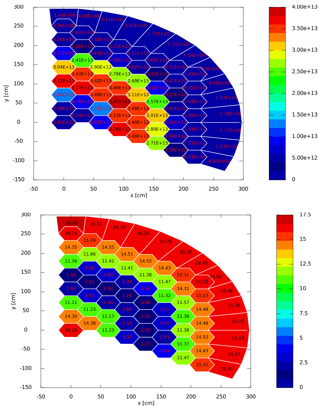
Figure B.5: Mean value and RSD for the axially averaged (active core region) fast flux–diffusion solutions
