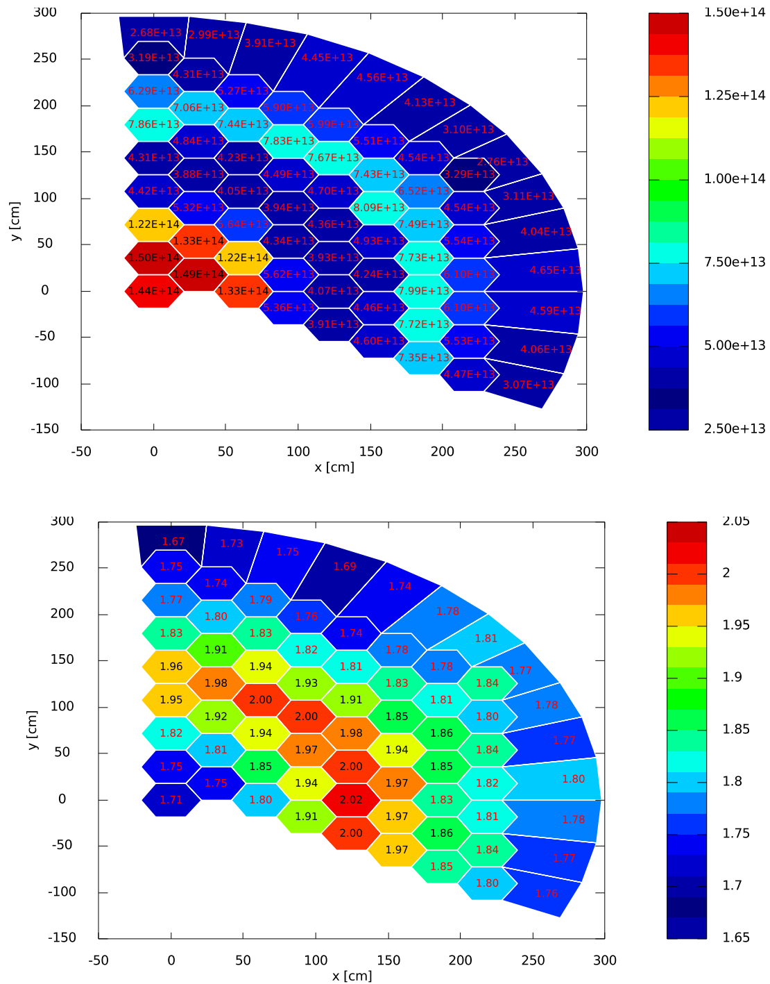
Figure A.10: Mean value and RSD for the axially averaged (active core region) thermal flux–transport solutions
