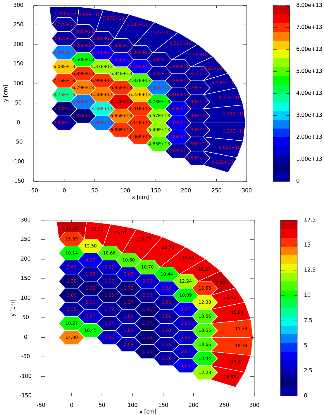
Figure B.7: Mean value and RSD for the axially averaged (active core region) epithermal flux–diffusion solutions
