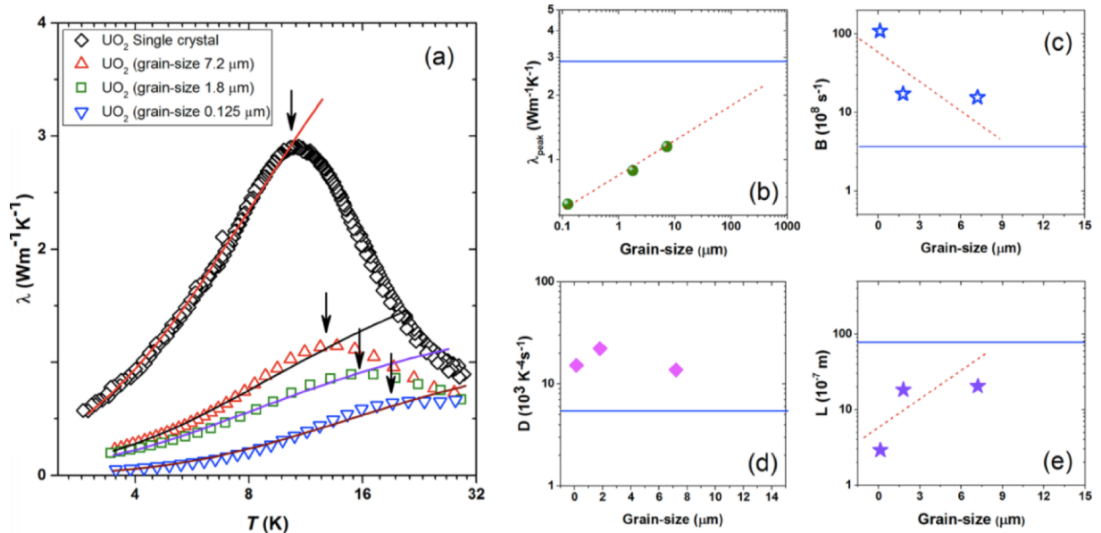
Figure 3. The low temperature thermal conductivity of \text{UO}_2 samples. The solid lines represent the least-square fits of the Callaway model to the experimental data. The grain-size dependence (obtained from the Callaway model) of the low-temperature thermal conductivity peak (b), parameters B (c), D (d), and the mean free path of phonons L (e). The corresponding values for the \text{UO}_2 single-crystal are displayed as a horizontal line in the relevant graphs. The dashed lines are guides to the eye.
