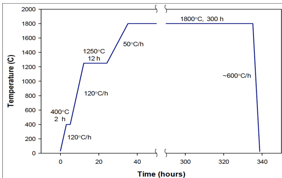
Figure 1. Temperature profile for the safety test of Compact 6-4-3. Elapsed time and ramp rates are approximate.
