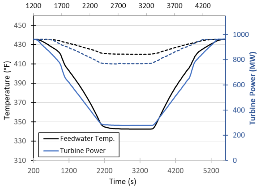
Figure 4-2. Feed water temperature and turbine power during the transition to 15% and 50% TPD.
