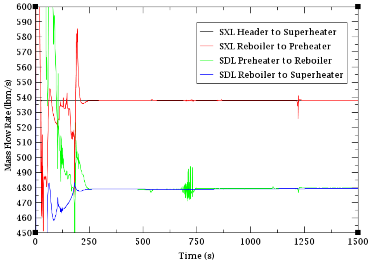
Figure 6-3. Transient results of selected mass flow rates of the steam-to-steam RELAP5-3D model.
