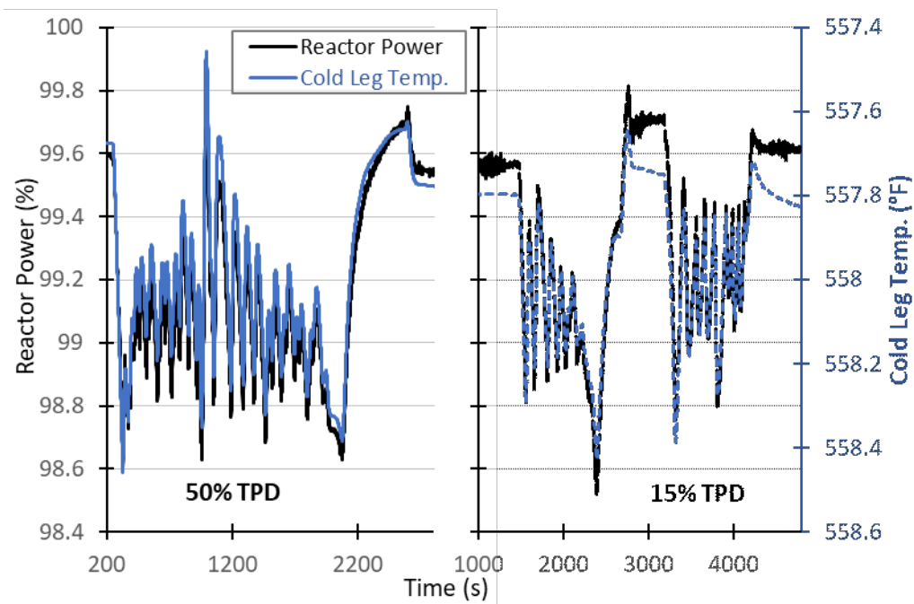
Figure 4-3. Reactor power and RCS cold leg temperature during the transition 15% and 50% TPD.
