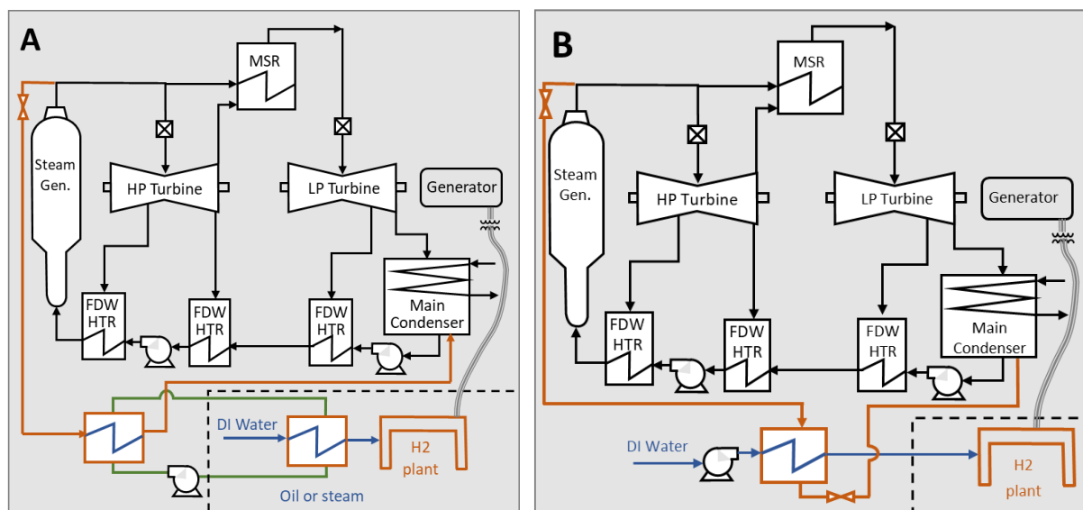
Figure 1-1. Simplified diagram of the Thermal Power Dispatch GPWR (TPD-GPWR) Simulator. Panel A: configuration for Versions #1 and #2. Panel B: configuration for Versions #3 and #4. The dashed line indicates the boundary of the NPP.
