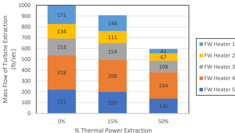
Figure 7-5. Turbine extraction flow to feed water heaters for 0%, 15%, and 50% TPD.
