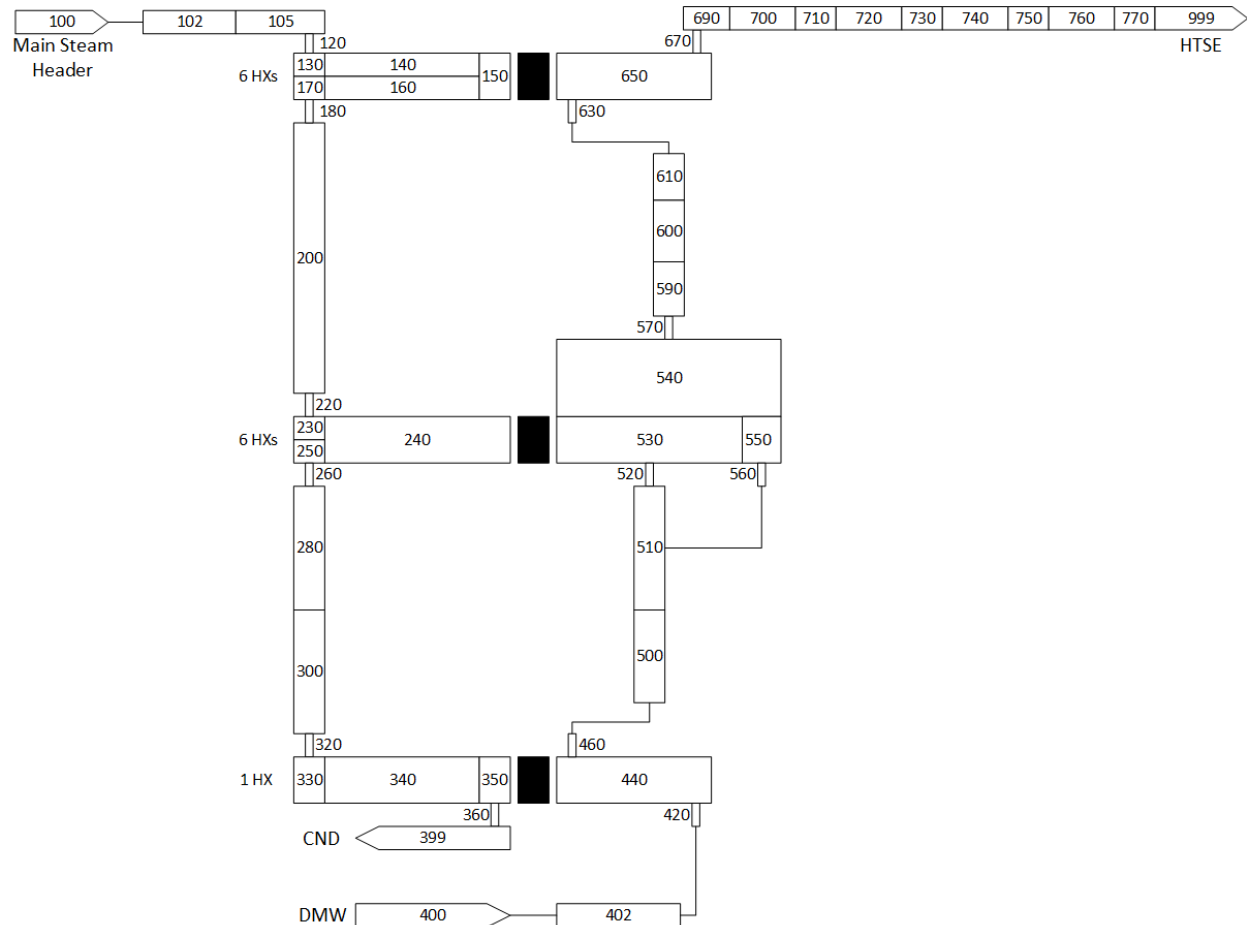
Figure 6-2. Nodalization of the RELAP5-3D for the steam to steam thermal power extraction system.
