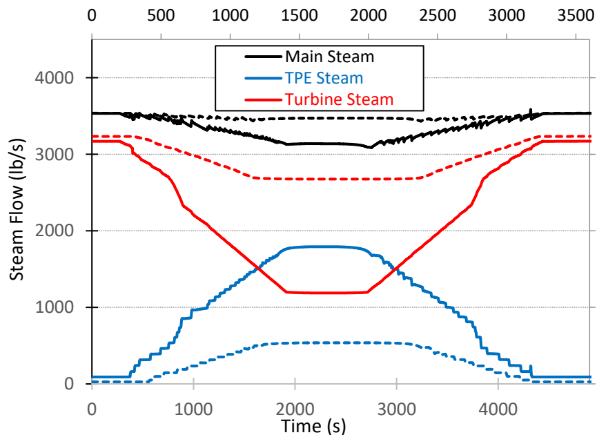
Figure 7-1. Steam flow rates for the transition to 15% and 50% TPD.
