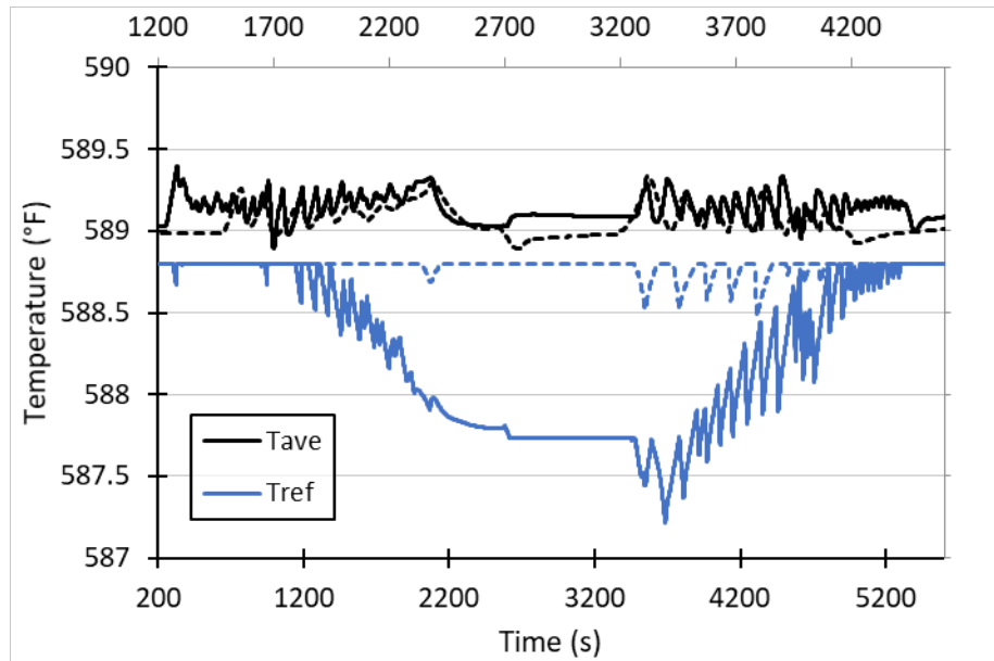
Figure 4-5. T_{ref} and T_{avg} for computing the mismatch in the control rod program during the transition to 15% and 50% TPD.
