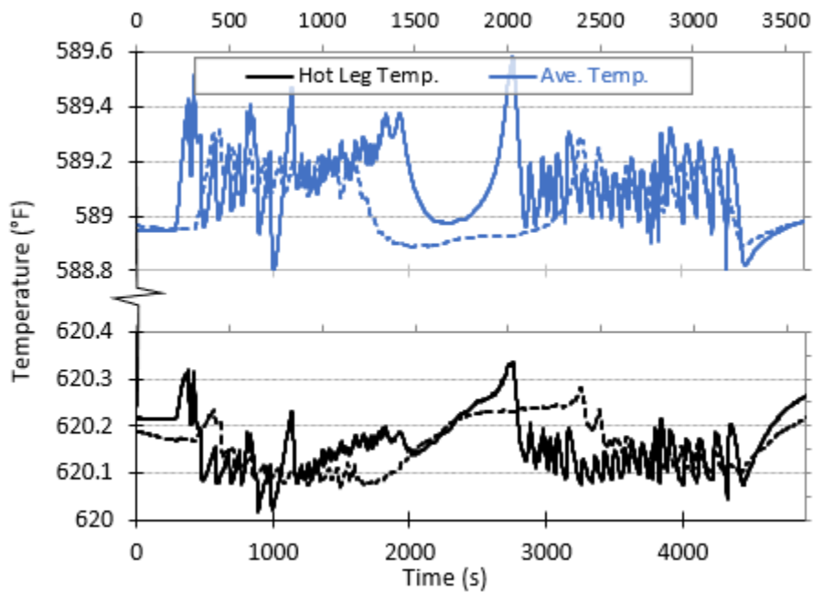
Figure 7-4. RCS hot leg temperature and RCS average temperature during the transition to 15% and 50% TPD.
