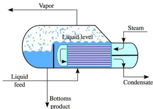
Figure 5-3. Diagram of a typical kettle reboiler.
