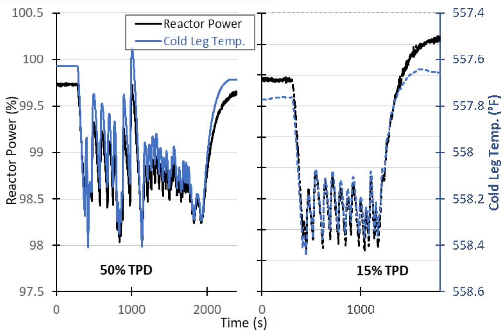
Figure 7-3. Reactor power and RCS cold leg temperature during the transition to 5% and 50% TPD.
