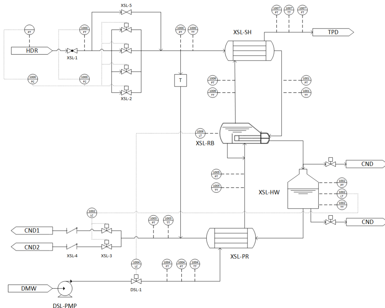
Figure 5-1. Simplified P&ID for the XSL and DSL systems.
