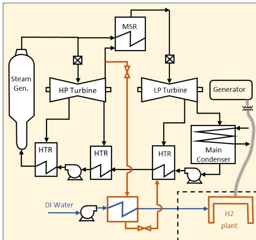
Figure 8-1. Simplified diagram of the improved thermal power dispatch from a PWR showing steam extraction from the high pressure turbine and condensate return to the feed water heater train.
