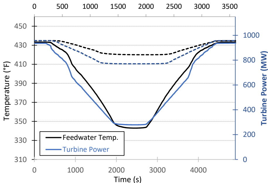
Figure 7-2. Feedwater temperature and turbine power during the transition to 15% and 50% TPD.
