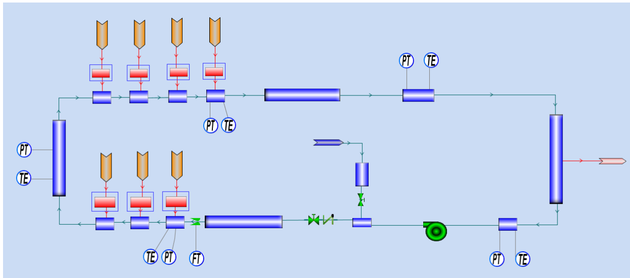
Figure 3-2. Screenshot of the delivery heat loop (DHL) piping system drawing for Versions #1 and #2 of the TPD-GPWR Simulator.
