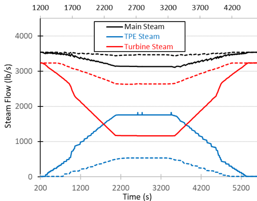
Figure 4-1. Steam flow rates for the transition to 15% and 50% TPD.
