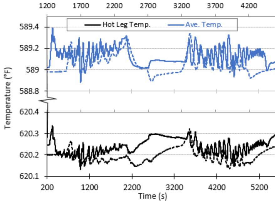
Figure 4-4. RCS hot leg temperature and RCS average temperature during the transition to 15% and 50% TPD.
