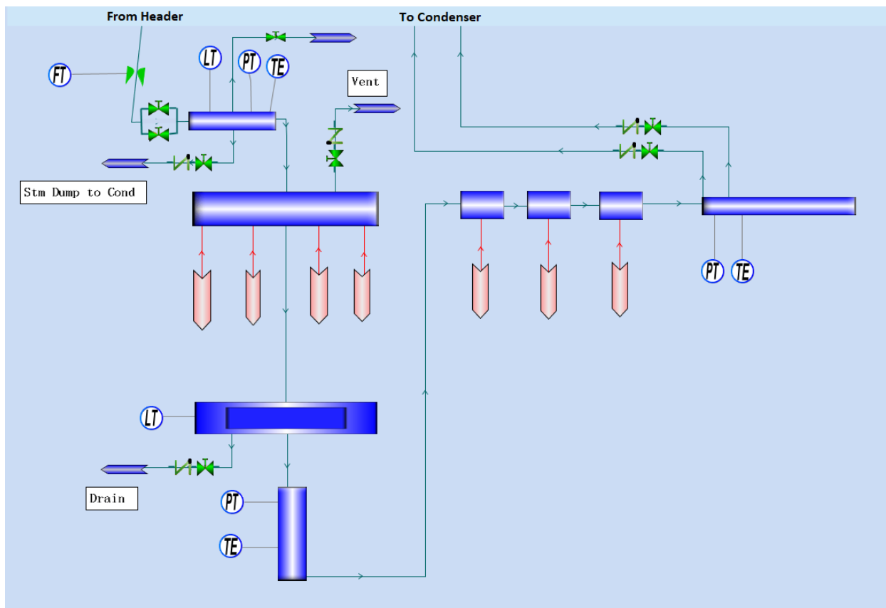
Figure 3-1. Screenshot of the extraction steam line (XSL) components added to the ms1 drawing of GPWR.
