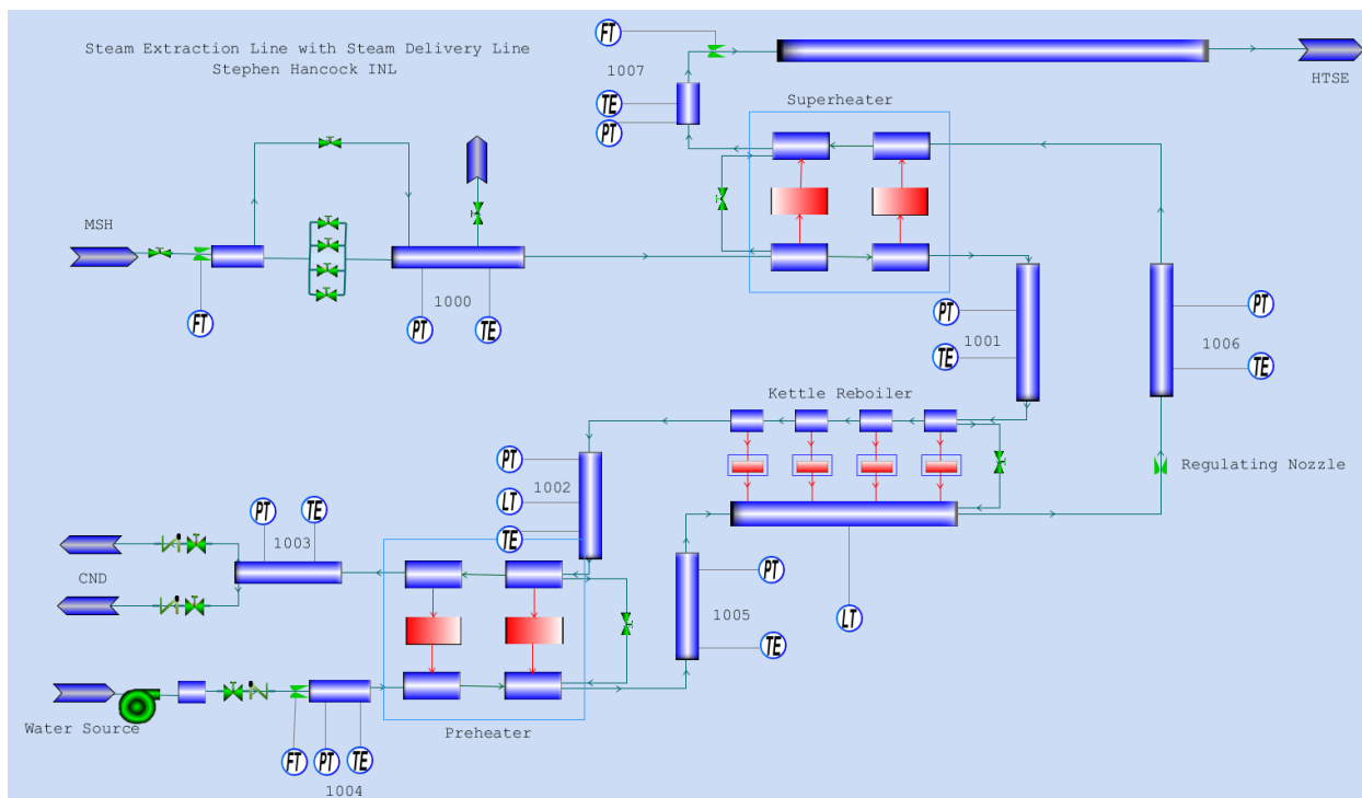
Figure 5-2. Screenshot of the tpe1 drawing containing the XSL and the DSL system in the GPWR.
