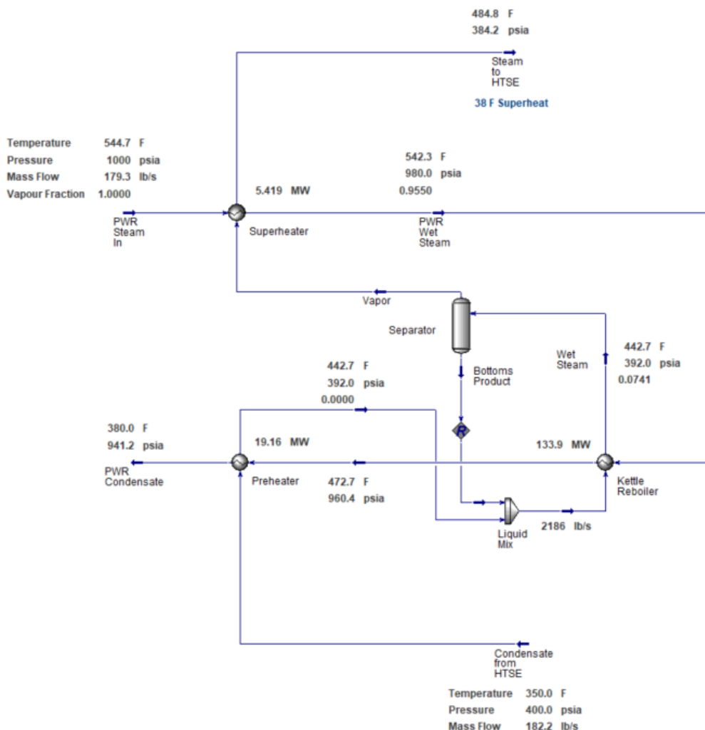
Figure 6-1. Process model in Aspen HYSYS for the TPD system with steam as the heat delivery fluid.
