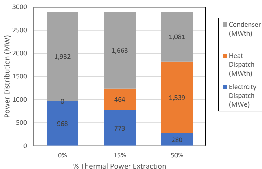
Figure 7-6. Power utilization breakdown of the TPD-GPWR simulator for 0%, 15% , and 50% TPD.
