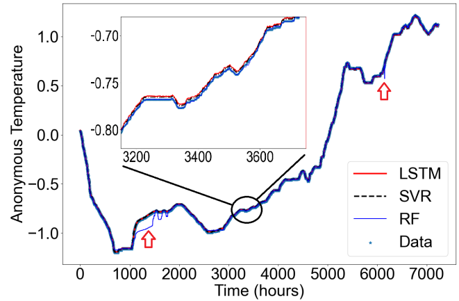
Figure 3. Predictions of pump temperature 1 hour ahead, using the SHAP-determined input to LSTM, SVR, and RF models.
