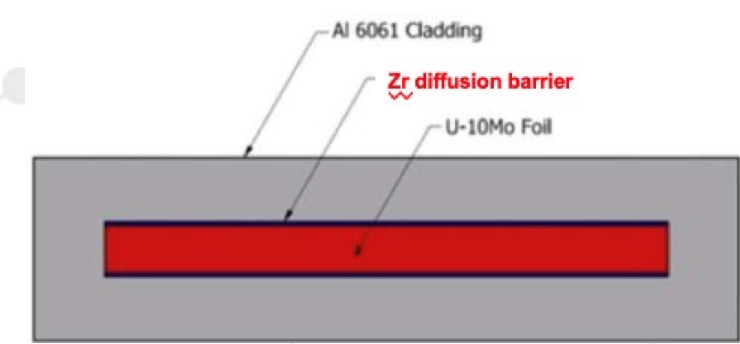
Notional configuration of U-10Mo plate fuel
