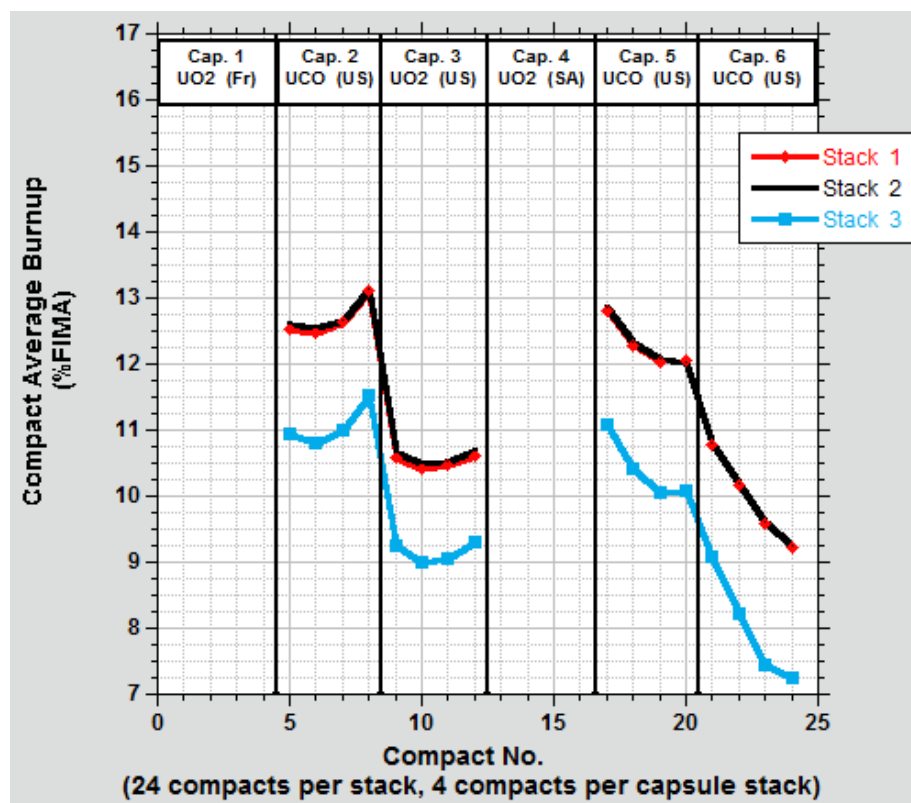
Figure 15. Calculated compact average burnups (%FIMA) by stack at the end-of-life (EOL 154B) for the four U.S. capsules.
