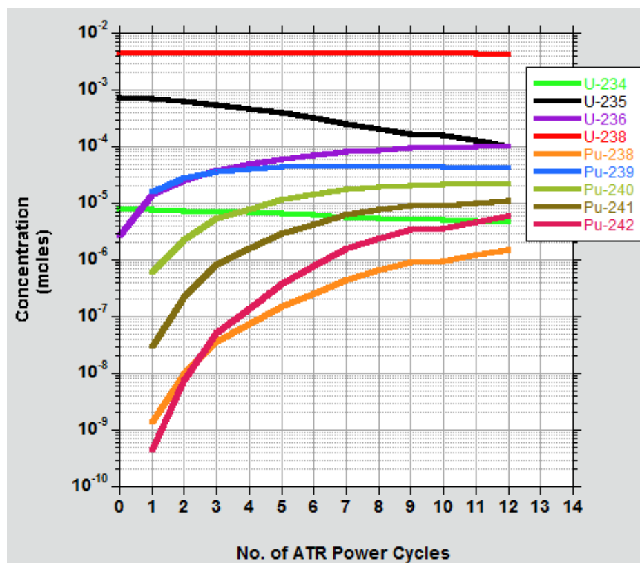
Figure 23. EOL 154B isotopic concentration as a function of the number of ATR power cycles for the high-burnup compact 2-4-2 (UCO U.S.).
