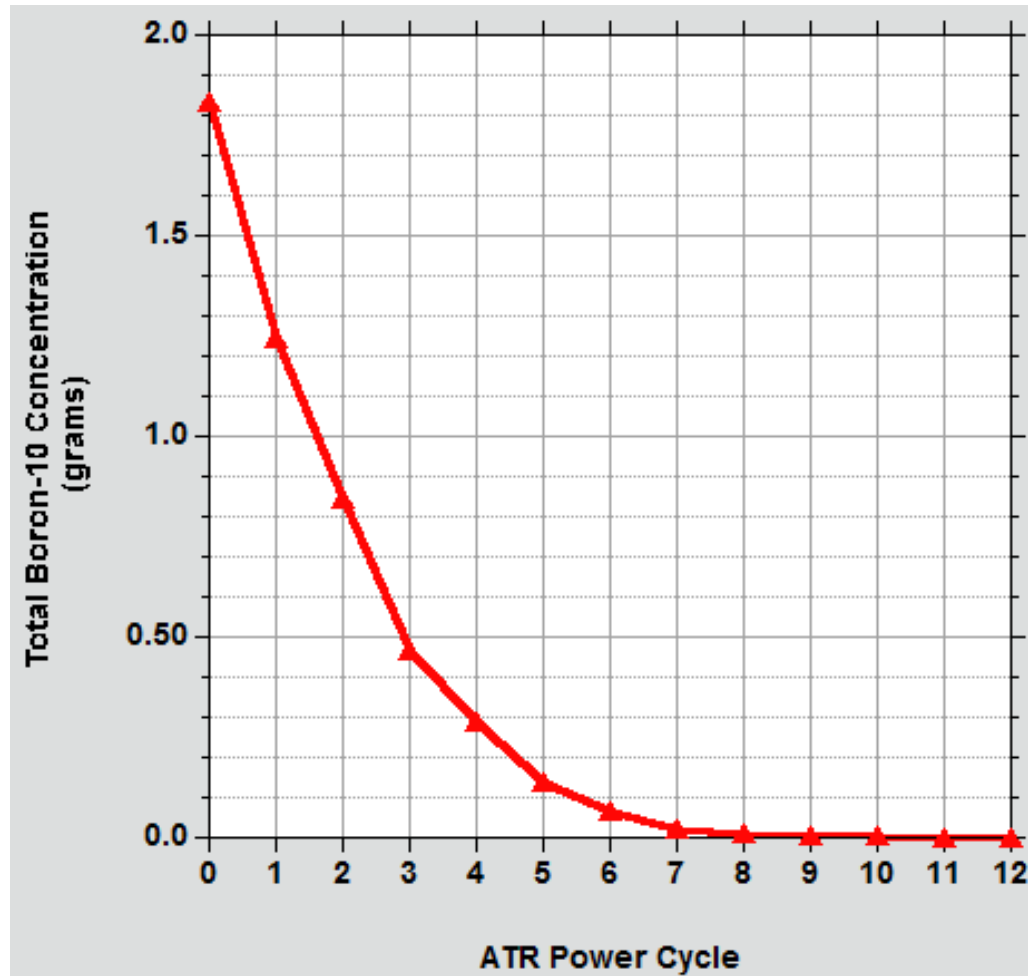
Figure 9. Total boron-10 mass in the six borated graphite holders at the end of each cycle.
