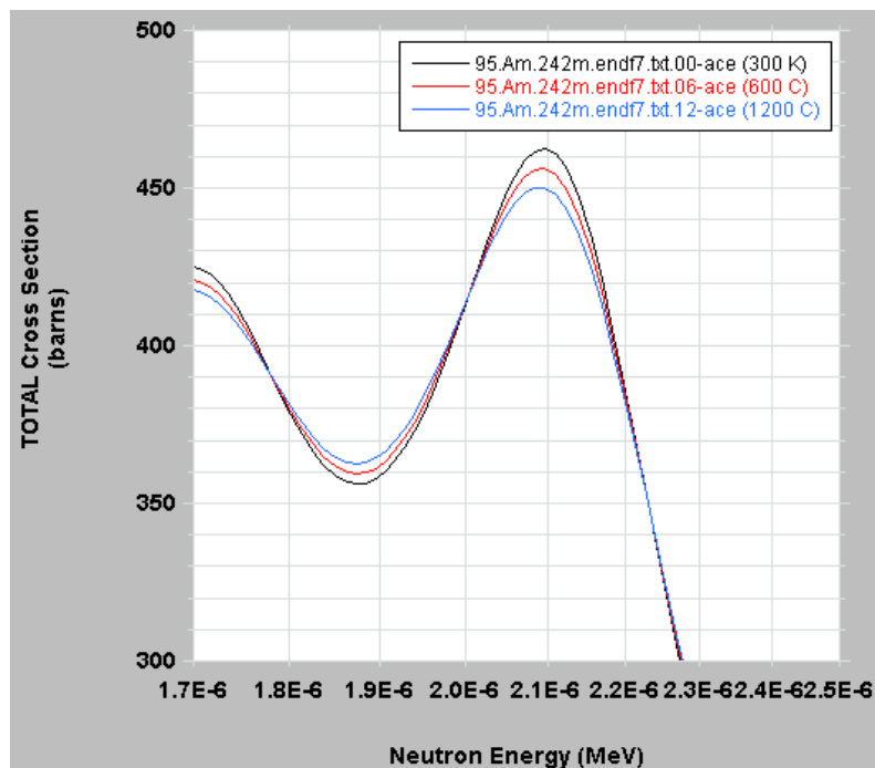
Figure C.6. Comparison of the Am-242m TOTAL cross section at 300 K, 600°C and 1200°C for a single resonance.
