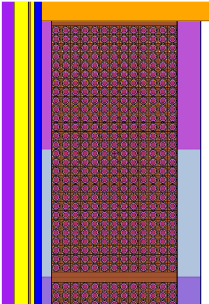
Figure 4. Axial view of the TRISO-coated particles in a UCO (U.S) compact (AGR-2 Capsule 6). Note the 28 particle layers per compact.
