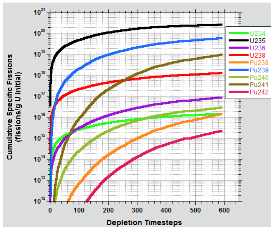
Figure 18. Isotopic cumulative specific fissions as a function of depletion timestep (burnup) for high-burnup compact 2-4-2 (UCO (U.S.)).
