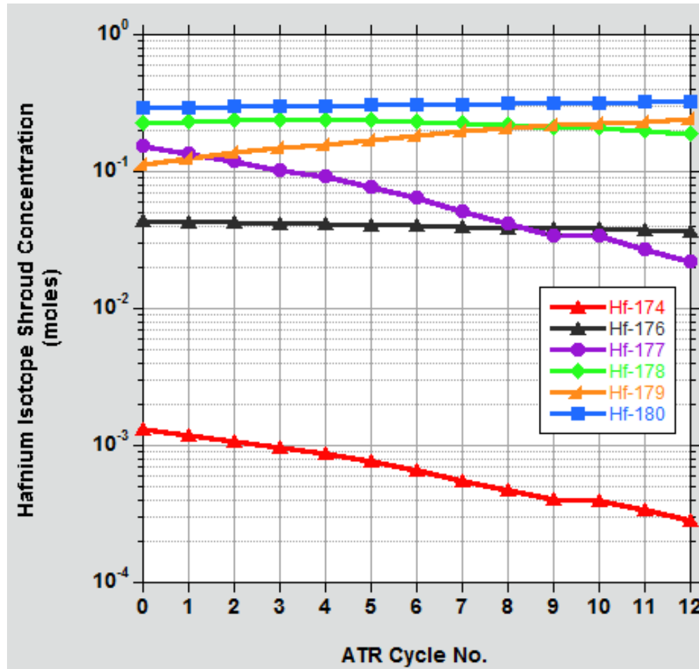
Figure 10. Total hafnium shroud isotopic mass as a function of the number of ATR power cycles.
