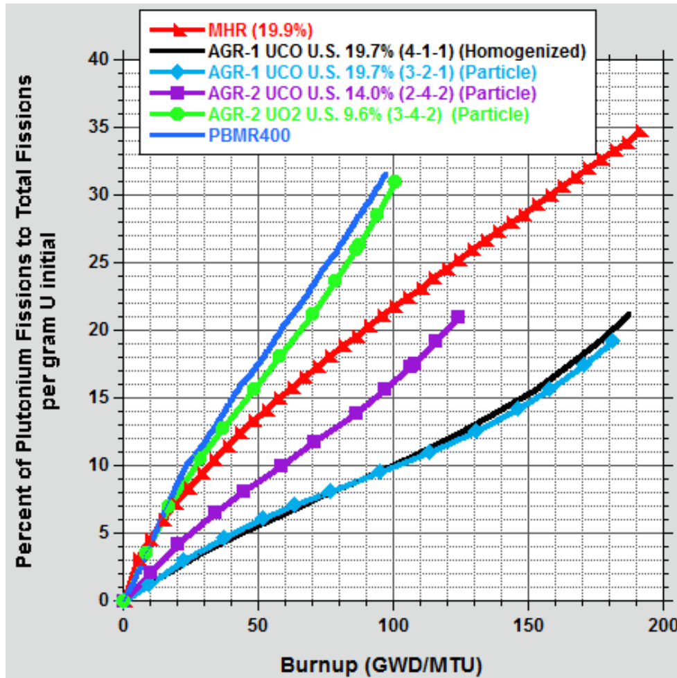
Figure 20. Comparison of plutonium fission fractions for different enrichment fuels from AGR-1, AGR-2, MHR [19], and PBMR400 [19].
