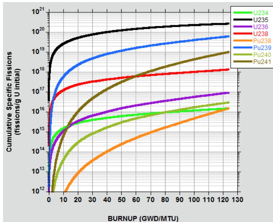
Figure 19. Isotopic cumulative specific fissions as a function of burnup (GWD/MTU) for high-burnup compact 2-4-2 (UCO U.S.).
