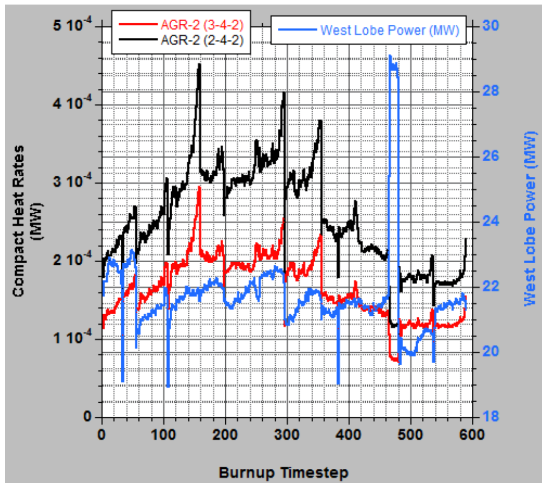
Figure 14. Calculated compact heat rates for compacts (3-4-2) and (2-4-2) as a function of burnup timestep over the 12 ATR power cycles.
