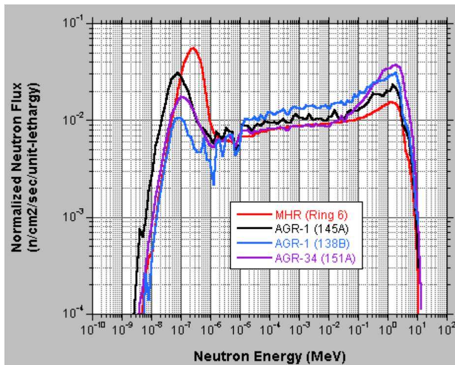
Figure 22. Neutron spectra comparison between the MHR, AGR-1, AGR-34, and MHR.
