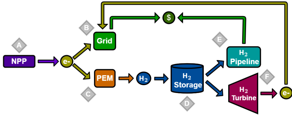
Figure 5. Diagram of DISPATCHES nuclear case components and the exchange of resources within the model.
