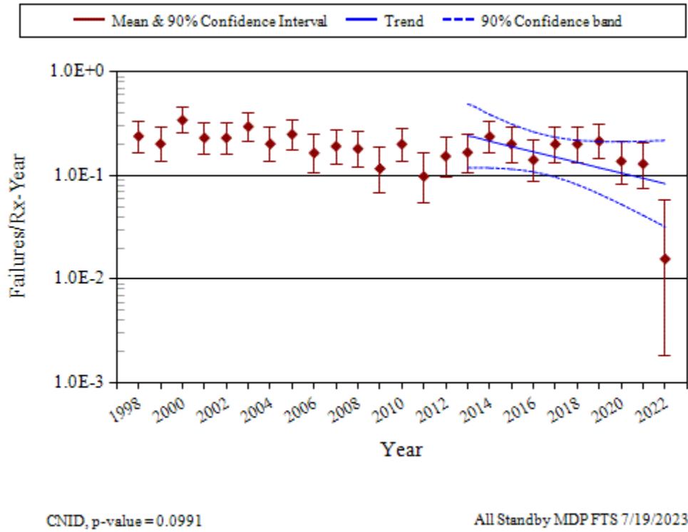
Figure 12. Frequency of FTS events (events per reactor year) trend for standby MDPs.
