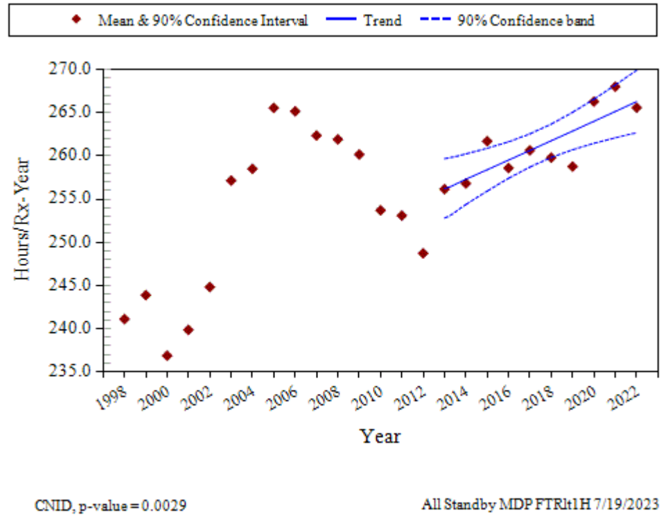
Figure 10. Frequency of run \leq 1H hours (hours per reactor year) trend for standby MDPs.
