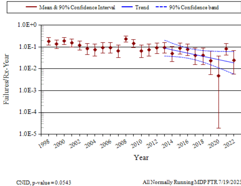
Figure 18. Frequency of FTR events (events per reactor year) trend for normally running MDPs.
