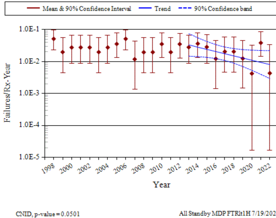
Figure 13. Frequency of FTR \leq 1H events (events per reactor year) trend for standby MDPs.
