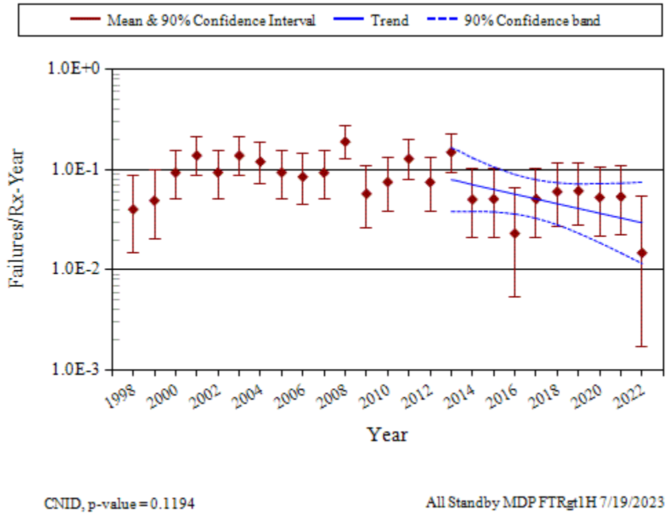
Figure 14. Frequency of FTR > 1H events (events per reactor year) trend for standby MDPs.
