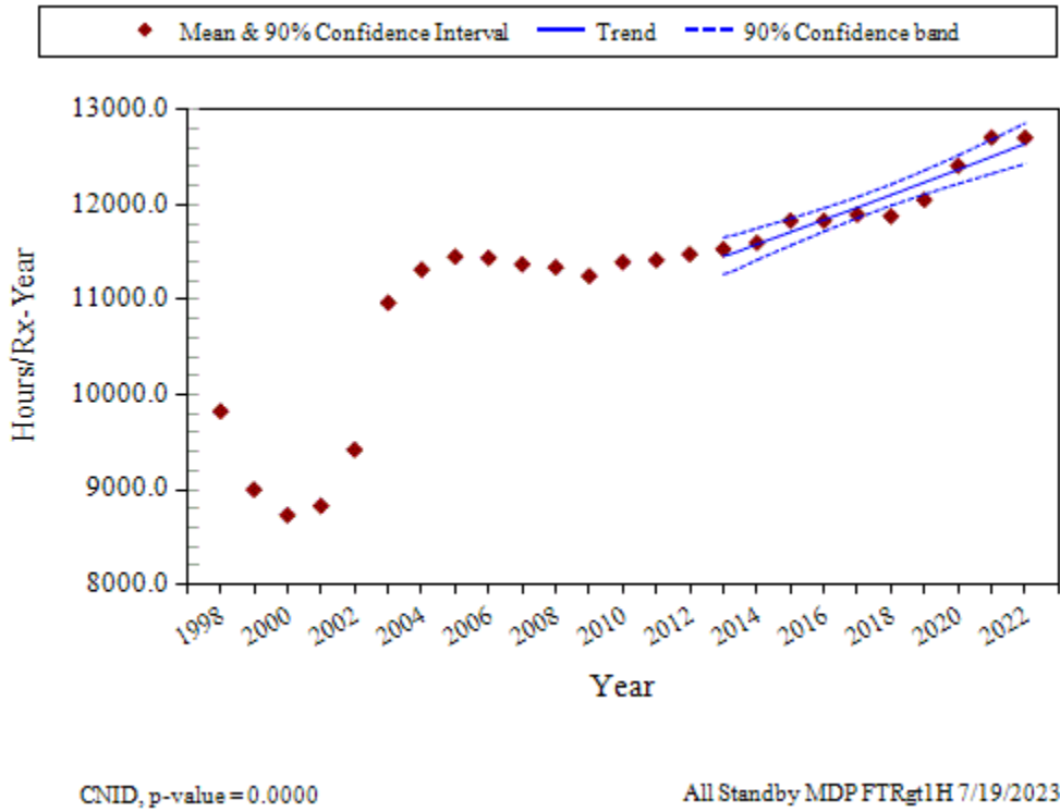
Figure 11. Frequency of run > 1H hours (hours per reactor year) trend for standby MDPs.
