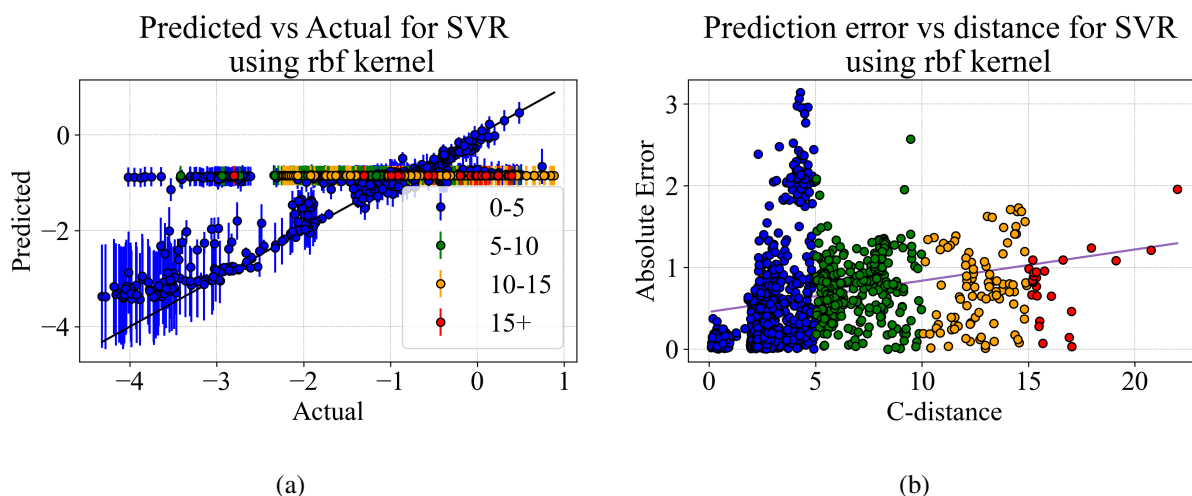
Figure 32. RBF SVR results: (a) predicted versus actual values (after standardization) for a set of outliers; (b) absolute prediction error versus Chebyshev distance from the nearest training data point (after standardization) for a set of outliers.
