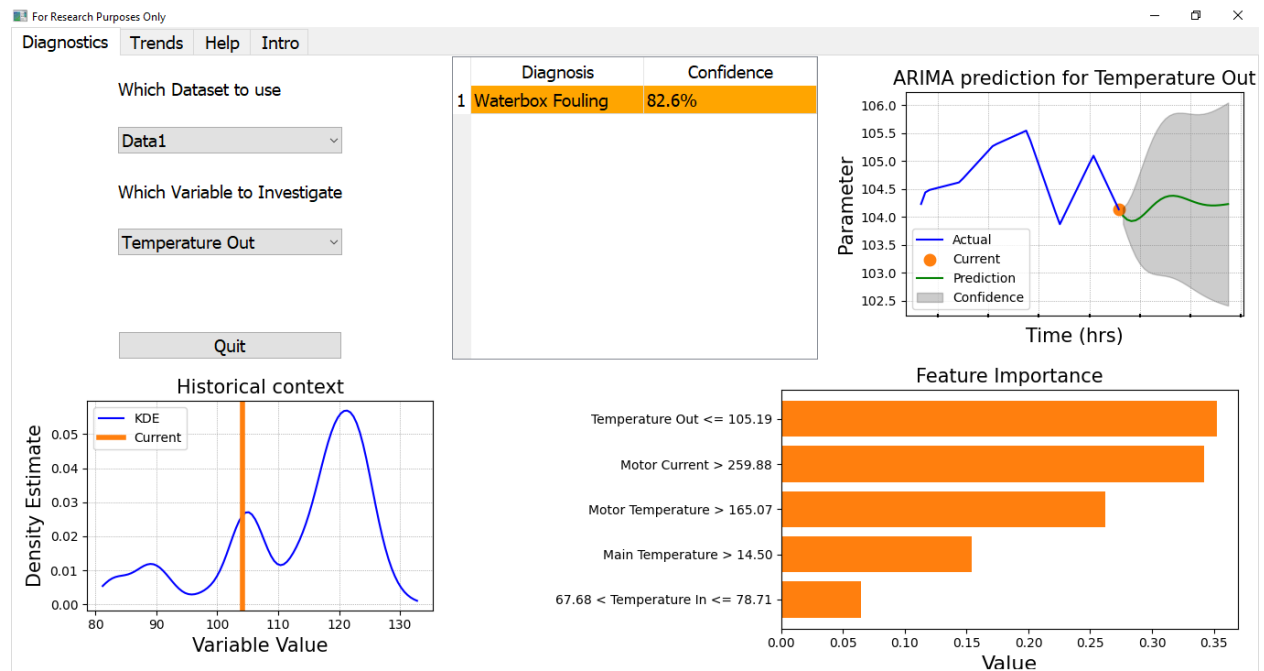
Figure 36. Front page of the NPIC application. This app has been tailored and focused for a diverse conference audience.
