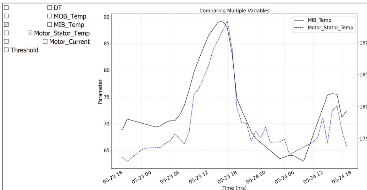
Figure 35. This figure is included in the M&D operator-version of the application and allows the operator to compare multi-signals on the same plot. This is useful to see how or if features are trending similarly.
