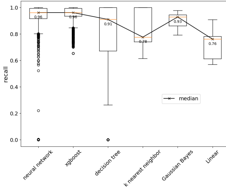
Figure 21. Distribution of model performance trained by healthy data twice as WBF data.
