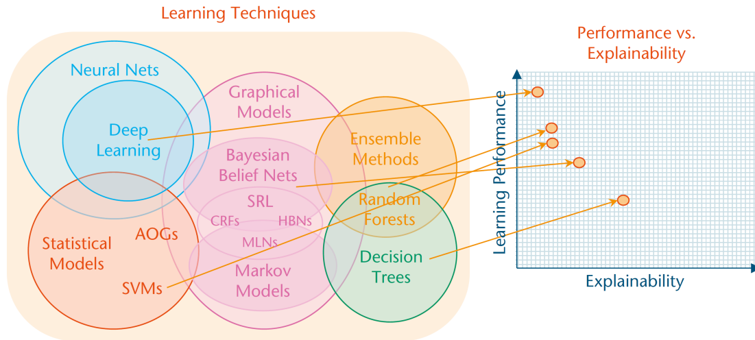
Figure 15. Synthetic learning performance versus explainability trade-off for several categories of learning techniques from [55].
