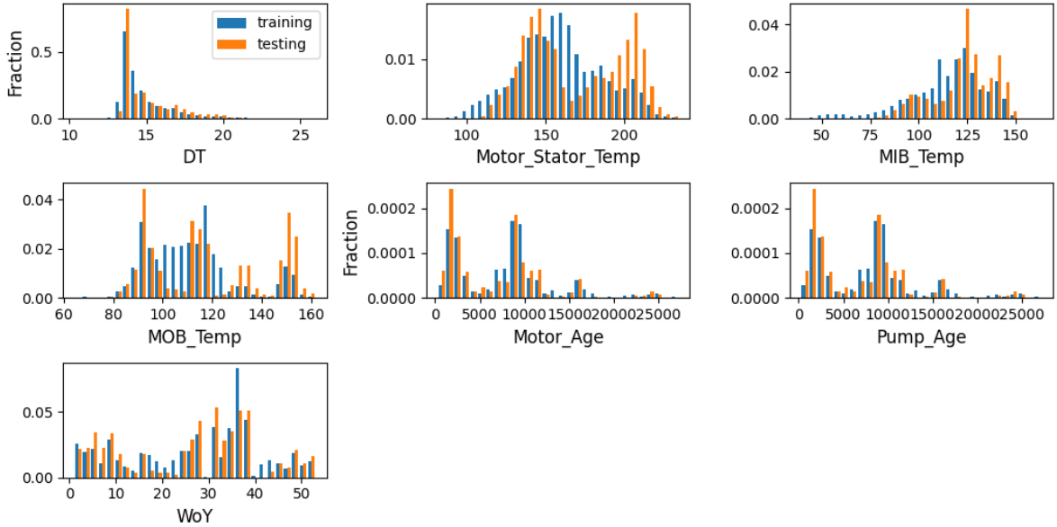
Figure 17. Comparison of training and testing data distributions with random sampling.
