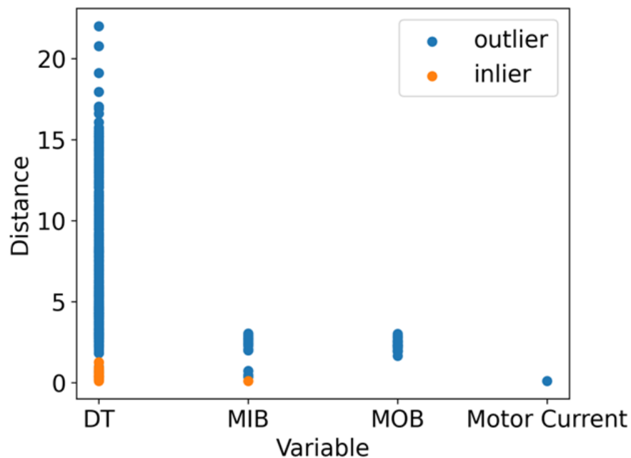
Figure 28. Chebyshev distance of all test data points and the parameter used to calculate it. Each data point was colored by isolation forest in accordance with its inlier/outlier status.
