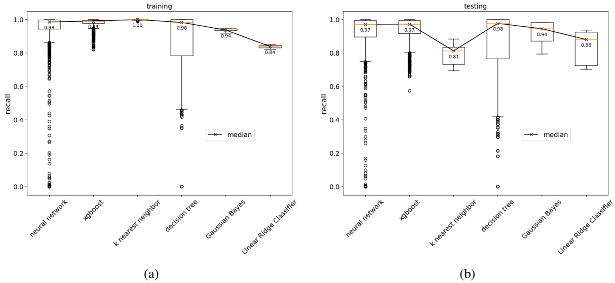
Figure 19. ML model performance for group-based sampling measured by recall rates in predicting (a) training data and (b) testing data.
