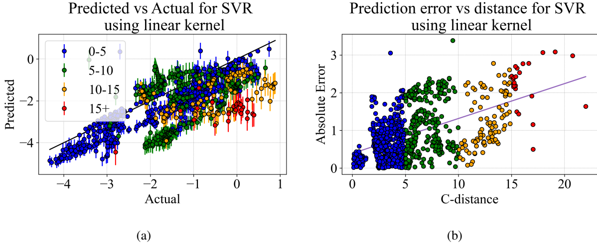
Figure 30. Linear SVR results: (a) predicted versus actual values (after standardization) for a set of outliers; (b) absolute prediction error versus Chebyshev distance from the nearest training data point (after standardization) for a set of outliers.
