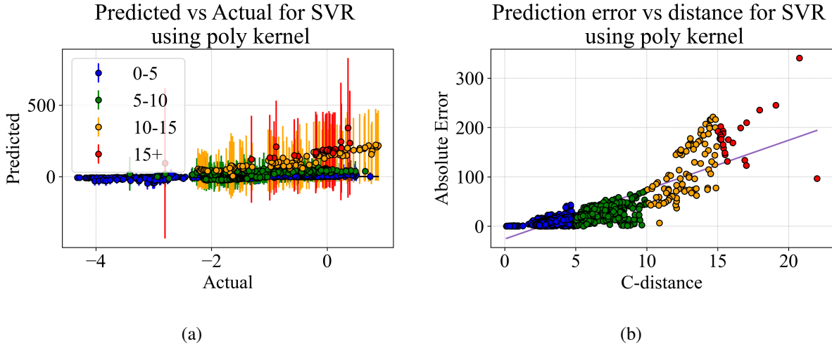
Figure 31. Polynomial SVR results: (a) predicted versus actual values (after standardization) for a set of outliers; (b) absolute prediction error versus Chebyshev distance from the nearest training data point (after standardization) for a set of outliers.
