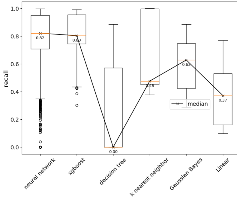
Figure 22. Distribution of model performance trained by healthy data five times as WBF data.
