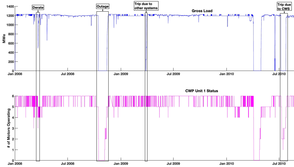
Figure 14. A sample of data showing the impact of availability of number of circulating water motors on the gross load.
