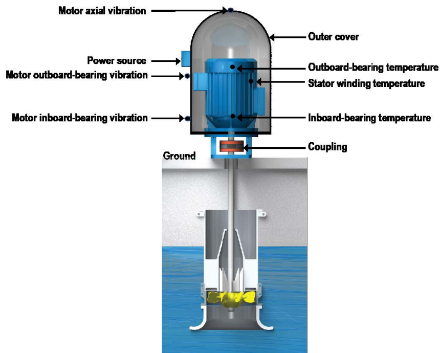
Figure 12. Schematic representation of a CWP and motor, along with vibration and temperature measurement locations.
