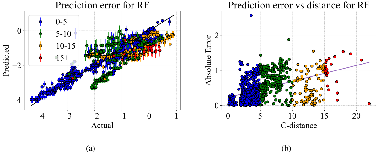
Figure 29. RF results: (a) predicted versus actual values (after standardization) for a set of outliers; (b) prediction error versus Chebyshev distance from the nearest training data point (after standardization) for a set of outliers.
