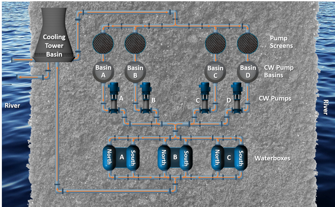
(b) Plant Site 2.
