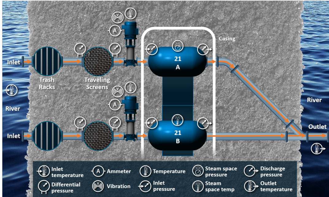
(a) Plant Site 1 Unit 2 CWP combination 21A and 21B.
