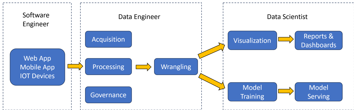
Figure 8. Data engineering and developer tools for big data (from [25]).
