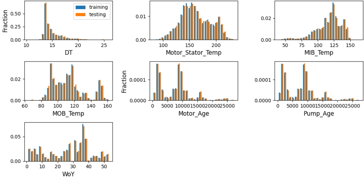
Figure 16. Comparison of training and testing data distributions with random sampling.
