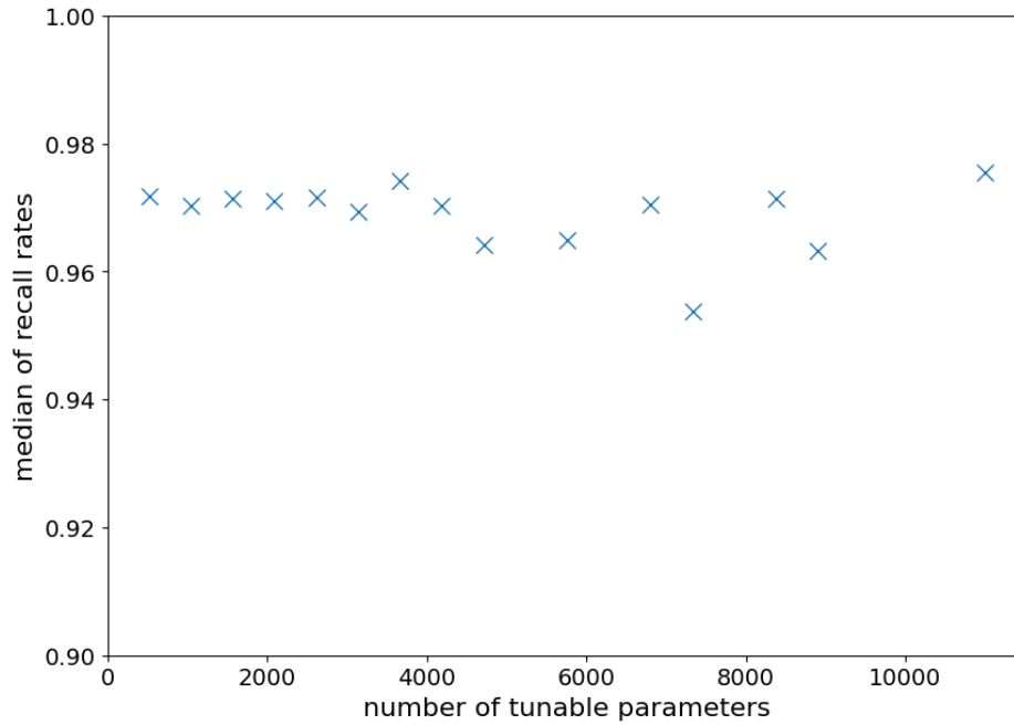
Figure 20. Relationship between number of tunable parameters in NN and the median of recall rates.
