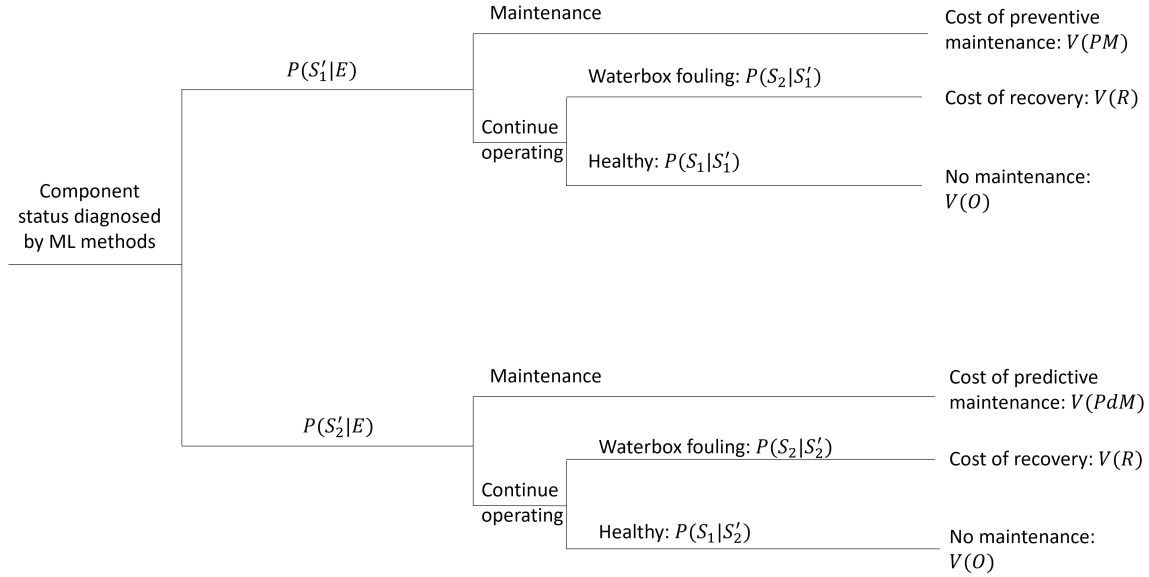
Figure 25. Decision tree model for maintenance based on diagnosis results. All possible states, prior probabilities, and expected values are included.
