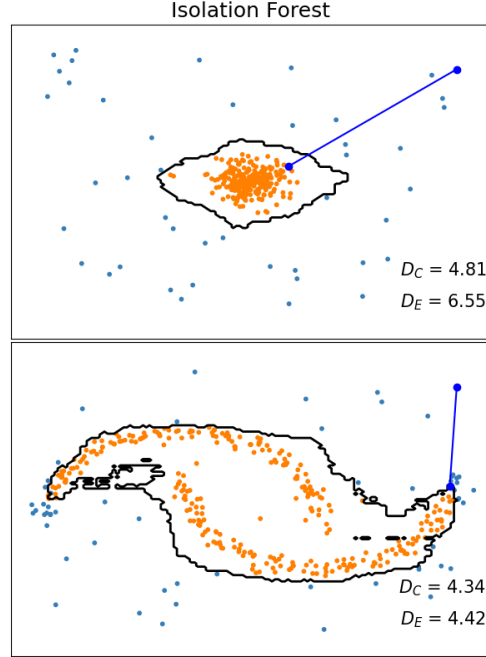
Figure 26. Distance measures applied to two different data distributions.
