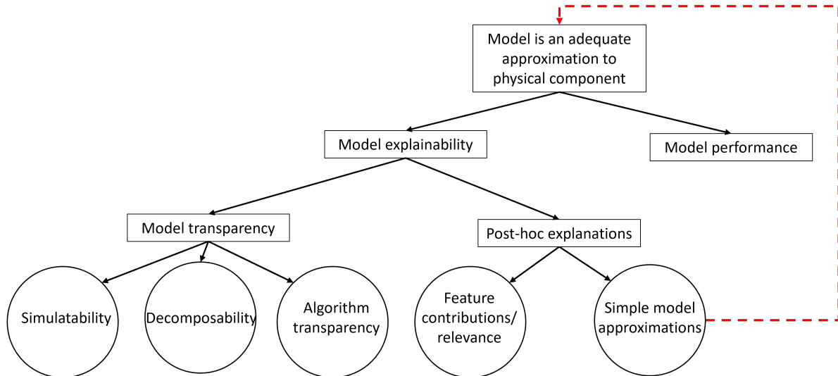
Figure 23. Explainability measures supported by qualitative attributes and corresponding evidence.
