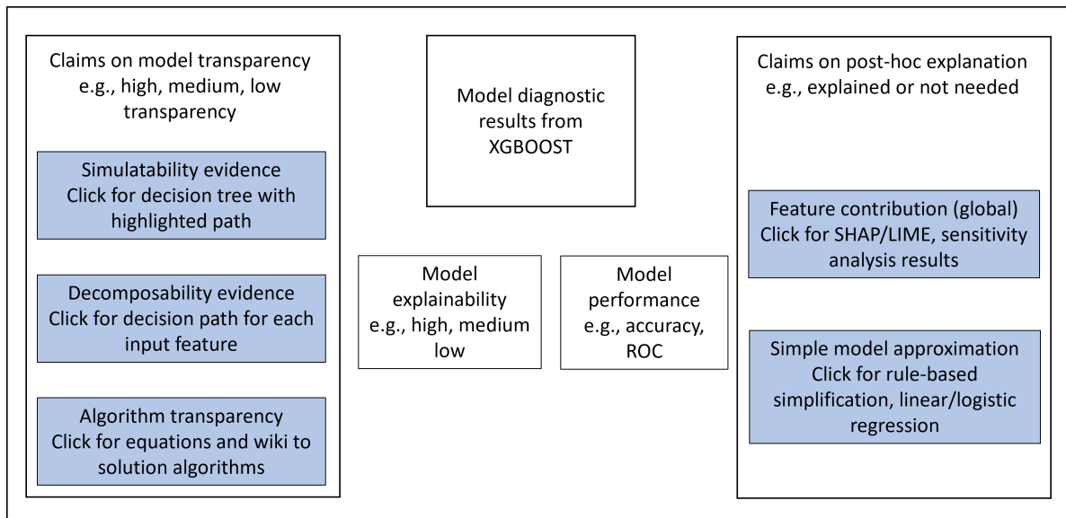
Figure 24. Explainability measures supported by qualitative attributes and corresponding evidence.
