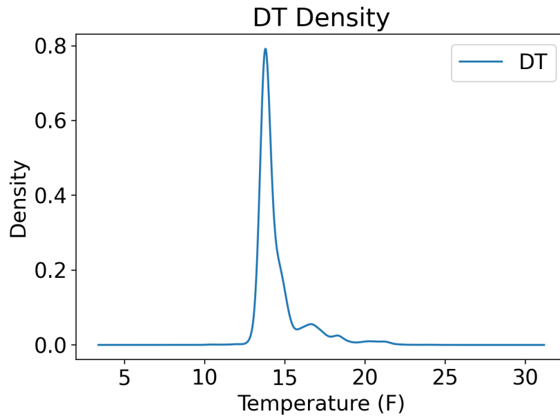
Figure 27. Kernel density estimate of the DT for the entire dataset.
