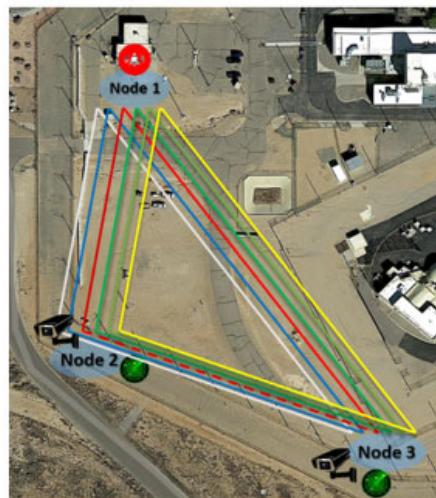
Example of CARBON Wireless nodes using multiple diverse underlay networks to transmit the same data streams
