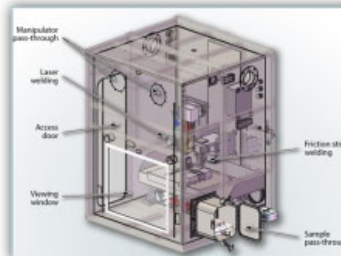
Fig. 1 Schematic (left) and actual photo (right) of friction stir welding and laser welding setup in hot cell
