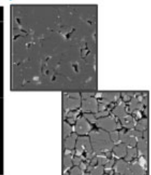
Fig. 3 SEM of the pristine (top) and irradiated (bottom) meta-chert samples showing grain boundary cracking (Maruyama et al. 2022)
