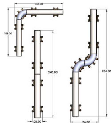
Example of 3D UAO Testing Configurations
