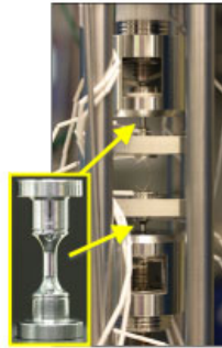
Fig. 1 SCC initiation & crack growth test system
