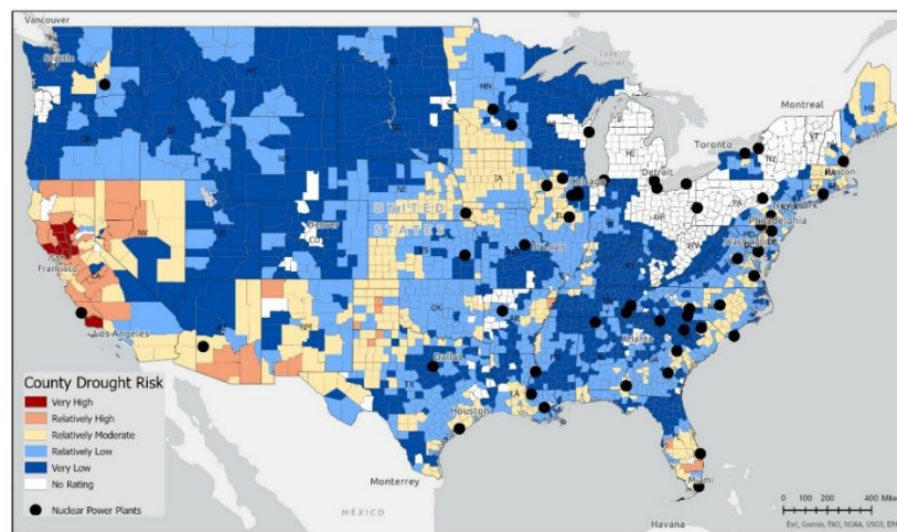
Figure 13. County-level drought risk index and operating nuclear power plant location.
