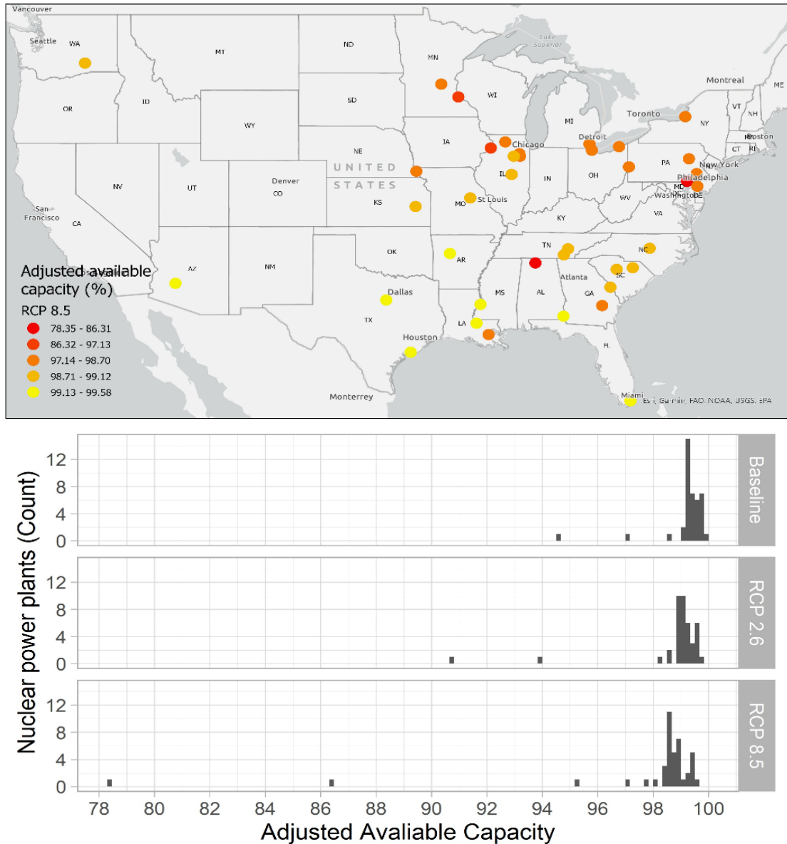
Figure 17. AAC histogram for 41 nuclear power plants under two future climate scenarios. Data source: (Miara et al. 2017). Results were modified to consider average summer temperatures as the inlet temperature thresholds, above which derating begins, to reflect regional design conditions more accurately for power plants. Data includes electricity generation performance for the months of June–August under a baseline (1985–2004), RCP2.6 (2045–2064), and RCP8.5 (2045–2064). Each AAC value is calculated as the mean of the four global circulation models (GFDL-ESM2M, HadGem2-es, MIROC-ESM-CHEM, and NORESM1-M) outputs. Power plant operations were simulated using the coupled Water Balance Model and Thermoelectric Power and Thermal Pollution Model (WBM–TP2M) at a daily time step.
