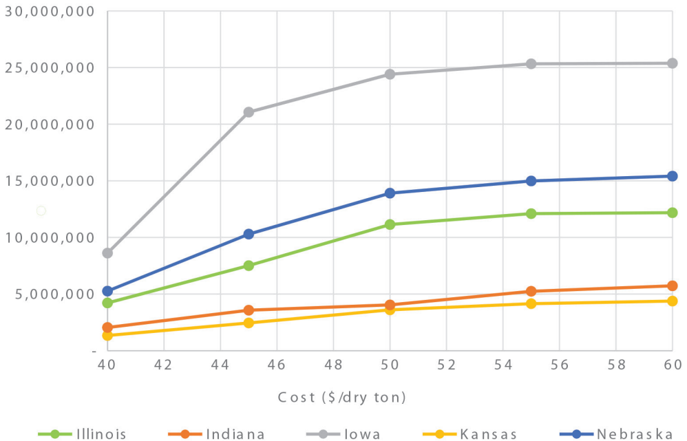
Figure 1. Corn stover availability by state as a function of farmgate price [33]. Availability and cost data assume base case corn stover yields for 2015. The data for each state is the sum of available corn stover for each county at a given farm gate price.
