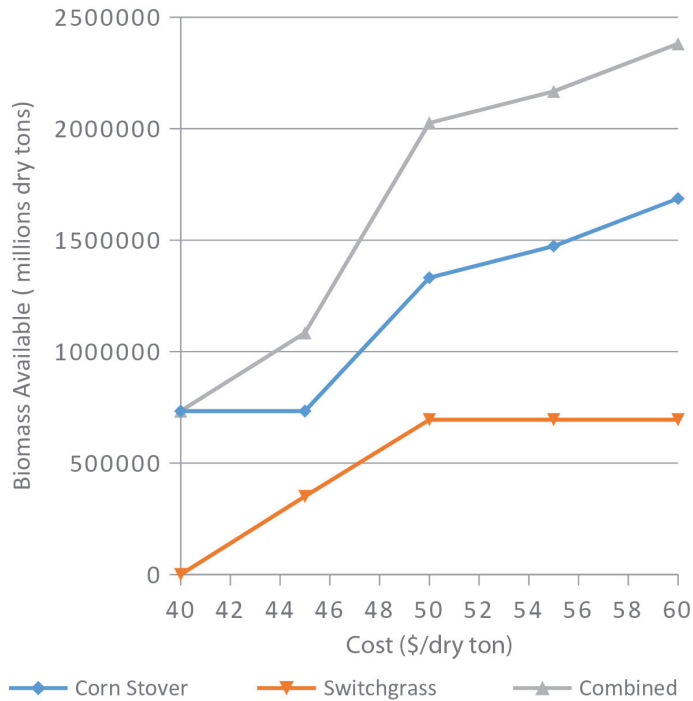
Figure 3. Biomass availability in northwestern Kansas as a function of farmgate price; prices and quantities shown are for 2015 and assume base case yields [34]. Supply curves illustrate biomass availability as a function of cost for a 12-county region in northwestern Kansas, with an approximate area of 90 miles \times 120 miles. Curves are shown for corn stover (blue), switchgrass (red), and combined for a blended supply of corn stover and switchgrass (green).
