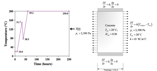
Figure 2. Initial conditions and time history of boundary conditions applied to the 2D axial symmetric model (modified from [13]). The thermal loading history on the inner surface is shown on the left.
