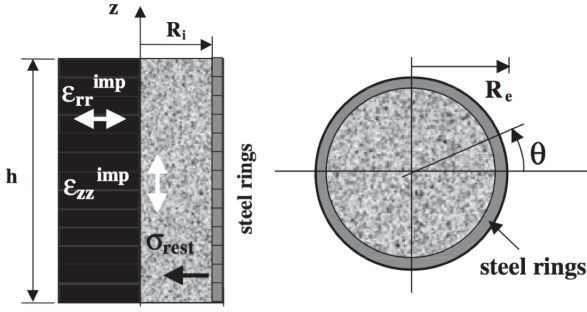
Figure 5. Schematic description of Multon and Toutlemonde's ASR expansion experiments [14]: (left) axial view and (right) plane view.
