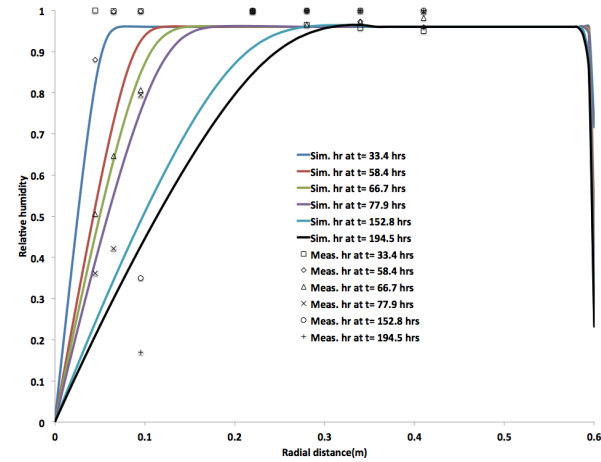
Figure 4: Comparisons of radial relative humidity profiles at various times between the simulation (lines) and experimental measurements (symbols).
