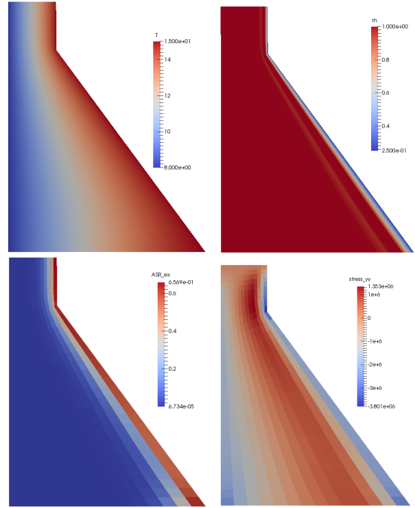
Figure 9. Simulated (upper-left) temperature, (upper-right) relative humidity, (lower-left) ASR reaction extend and (lower-right) vertical stress fields at 7 years.
