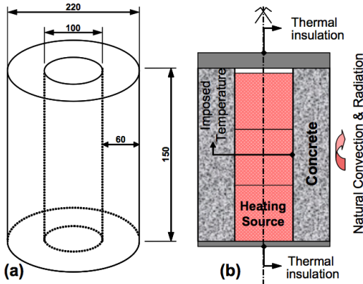
Figure 1. Geometric characteristics of MAQBETH mock-up concrete hollow cylinder (a) (from [12]) and
