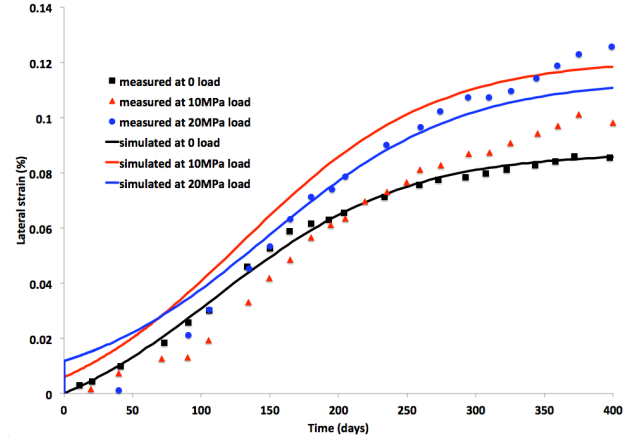
Figure 6. Comparisons of the measured and simulated lateral strains of specimens without lateral confinement under three axial loads, 0, 10 and 20 MPa.
