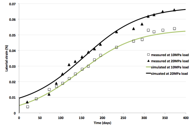
Figure 7. Comparisons between the simulated and measured lateral strains for confined specimens at 10 and 20 MPa axial loading stresses.
