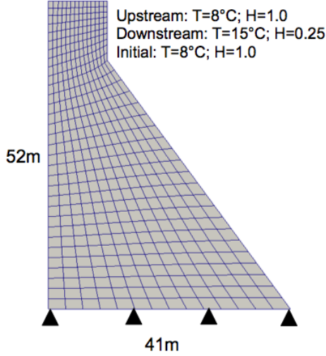
Figure 8. Structural dimension, FEM mesh, and boundary/initial conditions of a concrete gravity dam.
