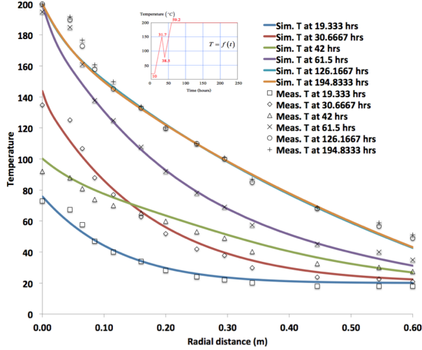
Figure 3. Comparisons of radial temperature profiles at various times between the simulation (lines) and experimental measurements (symbols).
