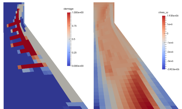
Figure 10. Simulated (left) damage and (right) vertical stress fields at time of \sim 8.2 years.
